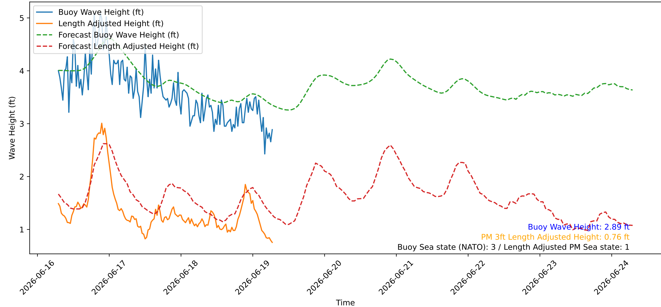
Wave Heights over Time for Green Beach at 2026-06-19 07:11:08
