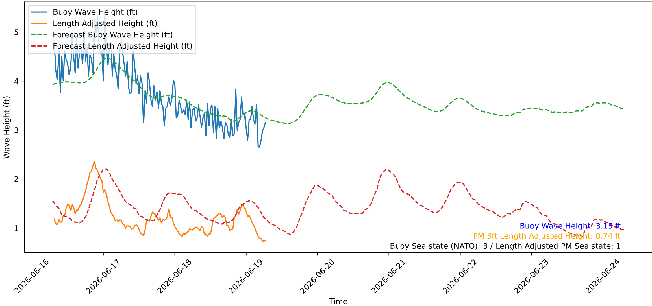
Wave Heights over Time for Red Beach at 2026-06-19 07:10:46
