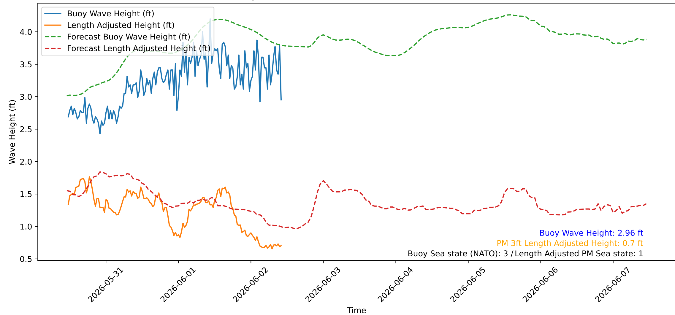
Wave Heights over Time for Red Beach at 2026-06-02 11:00:44
