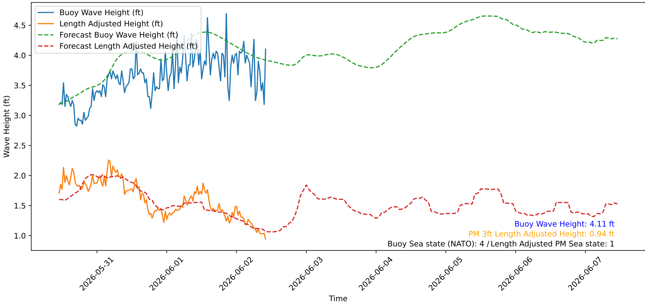
Wave Heights over Time for Oceanside Harbor at 2026-06-02 11:00:25
