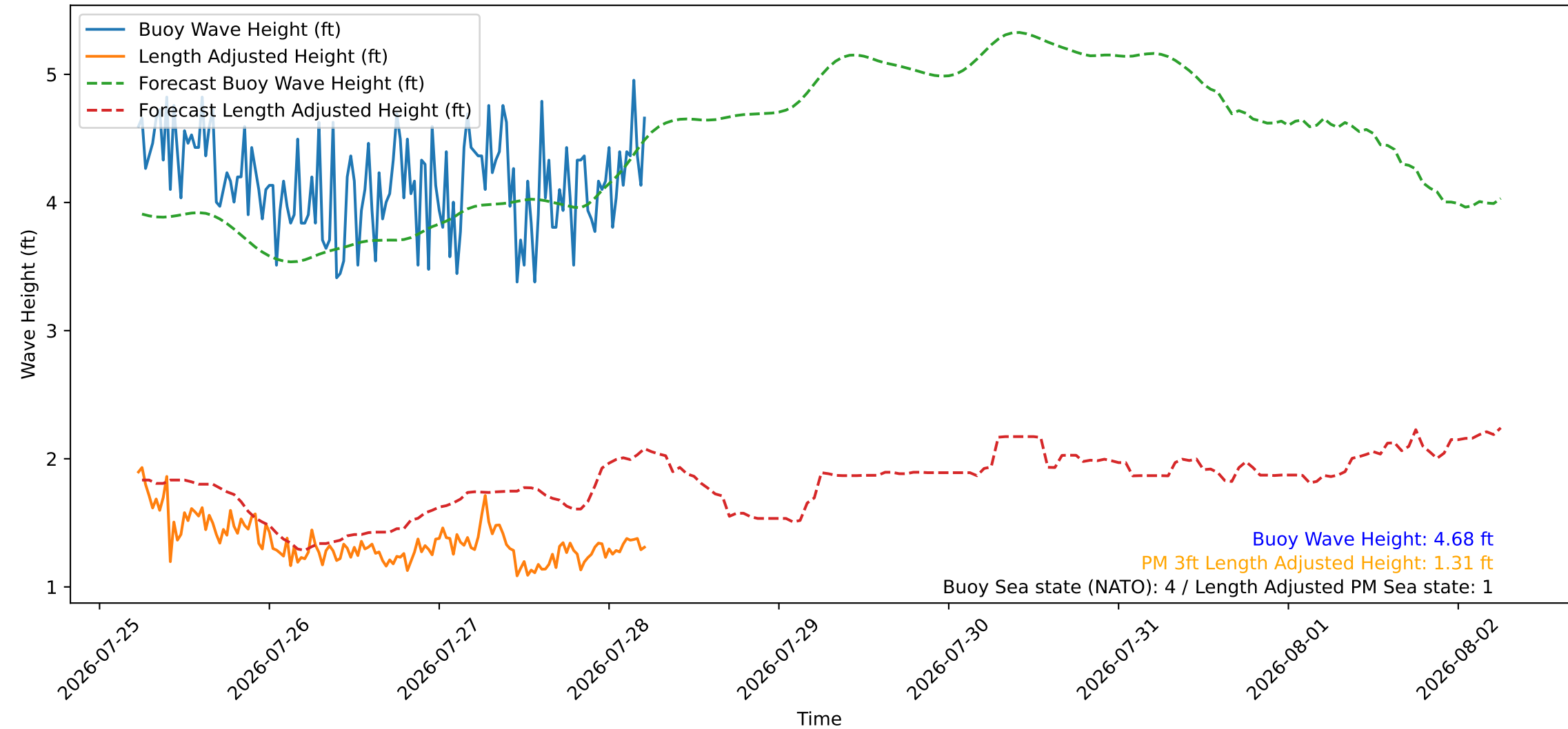
Wave Heights over Time for Green Beach at 2026-07-28 05:41:09
