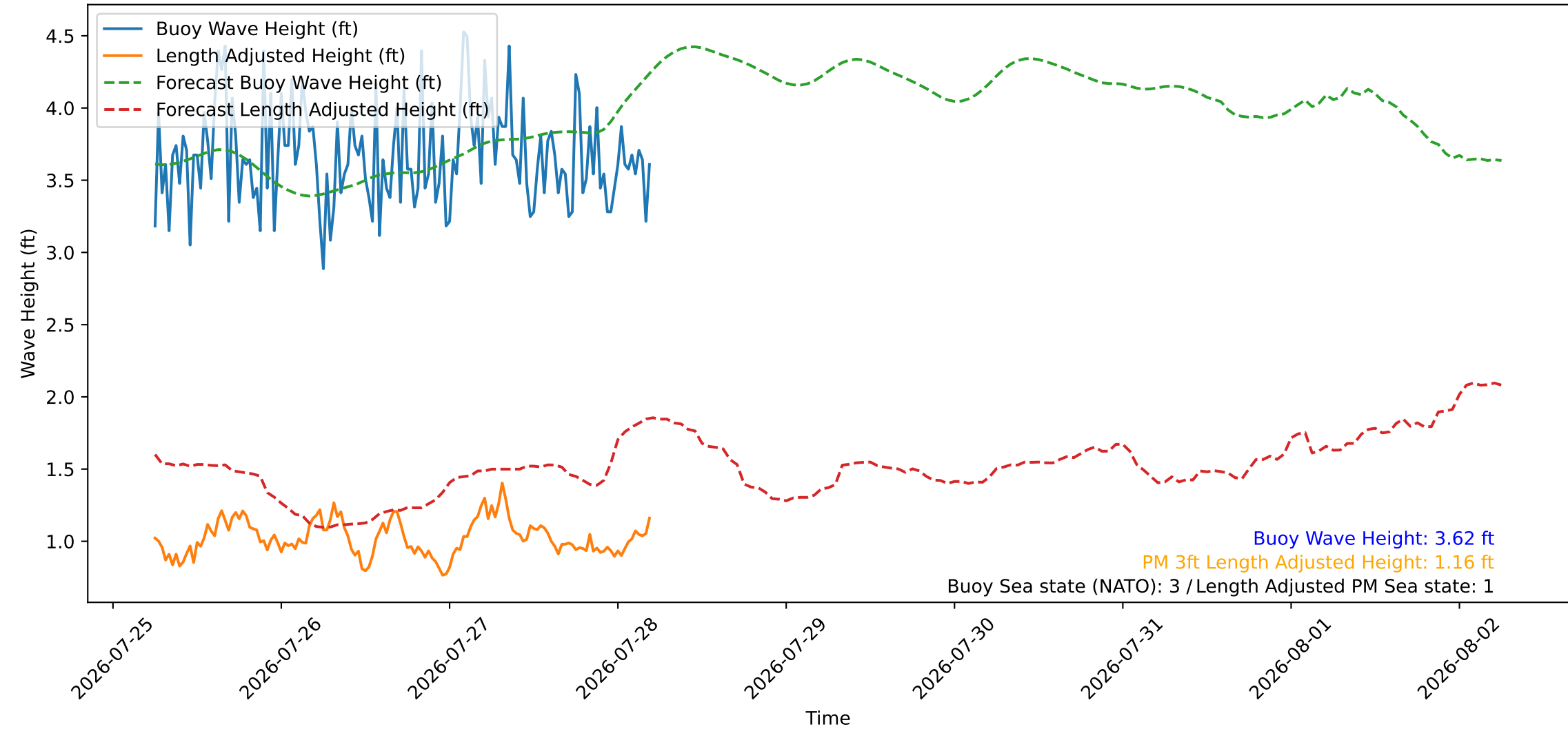
Wave Heights over Time for Red Beach at 2026-07-28 05:40:46
