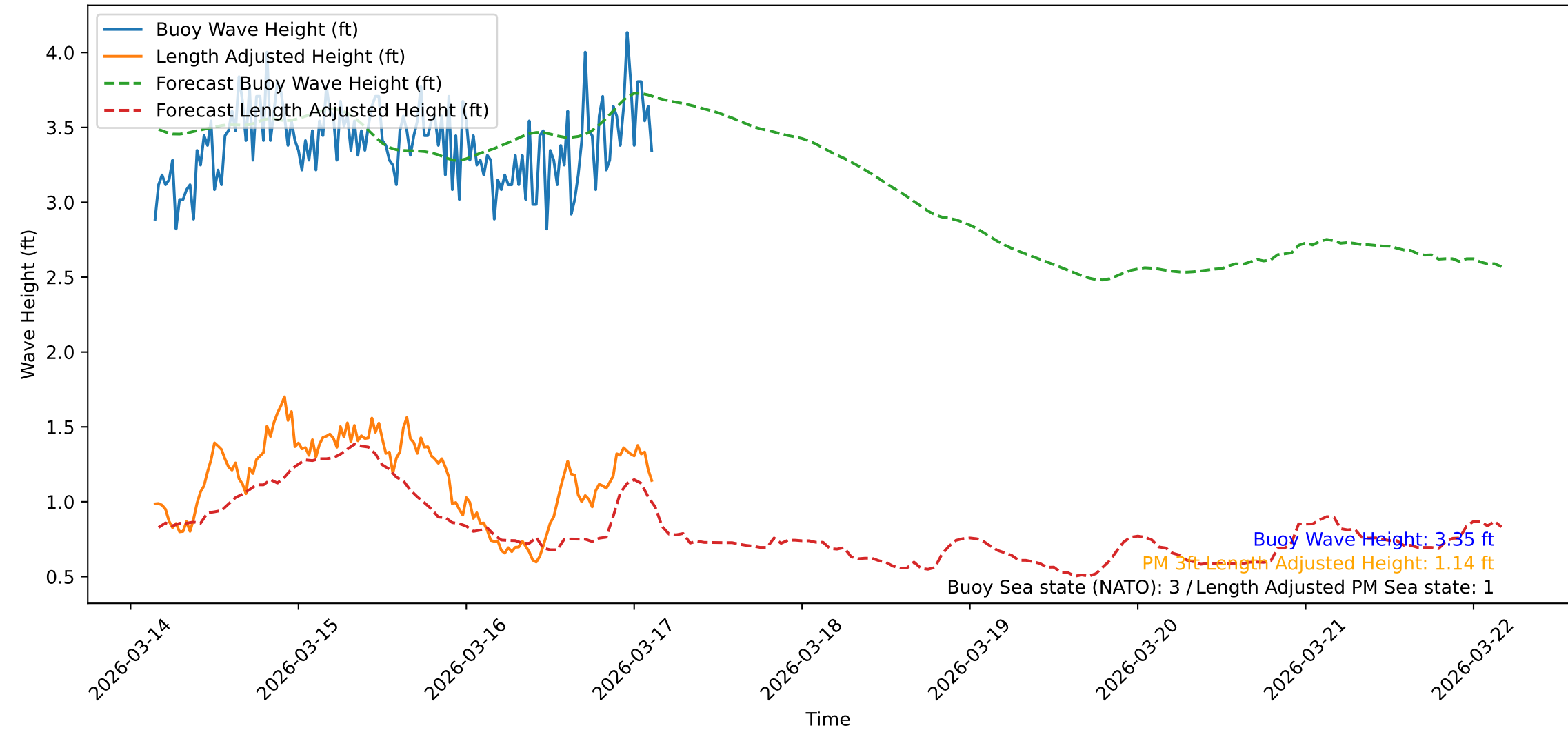
Wave Heights over Time for Green Beach at 2026-03-17 03:31:43
