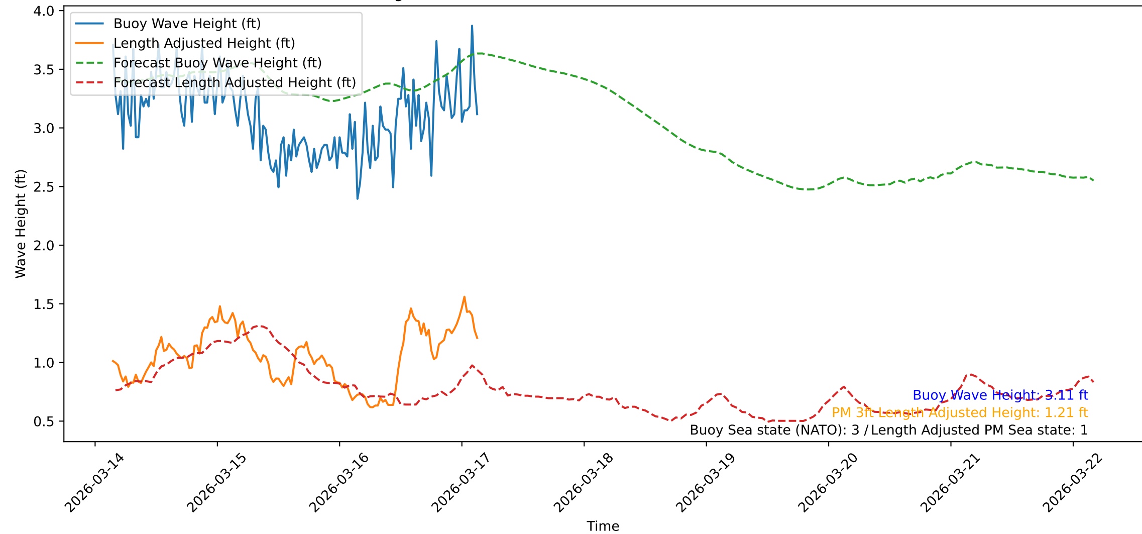
Wave Heights over Time for Oceanside Harbor at 2026-03-17 03:30:44
