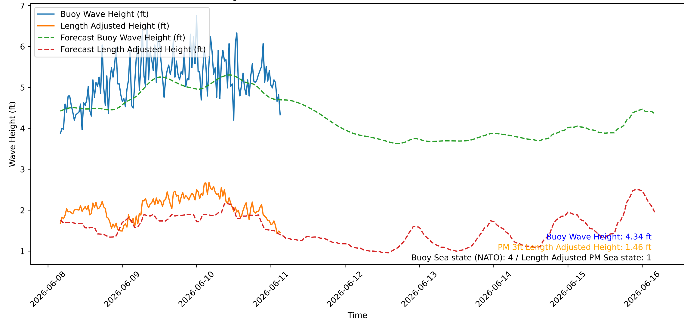
Wave Heights over Time for Oceanside Harbor at 2026-06-11 03:50:26
