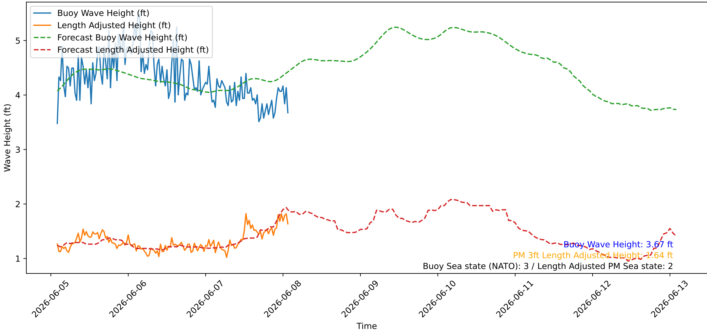
Wave Heights over Time for Oceanside Harbor at 2026-06-08 02:00:26
