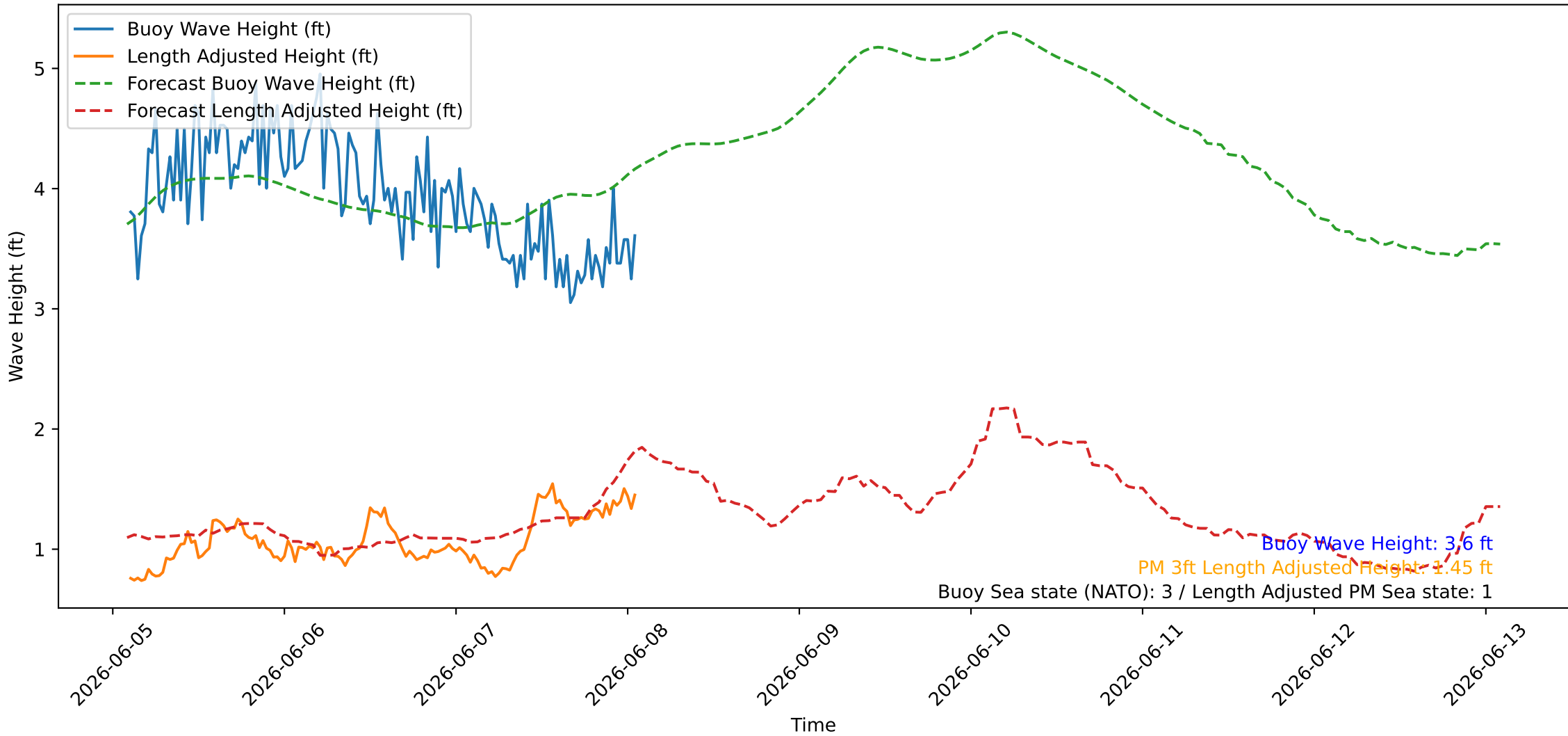
Wave Heights over Time for Red Beach at 2026-06-08 02:00:46
