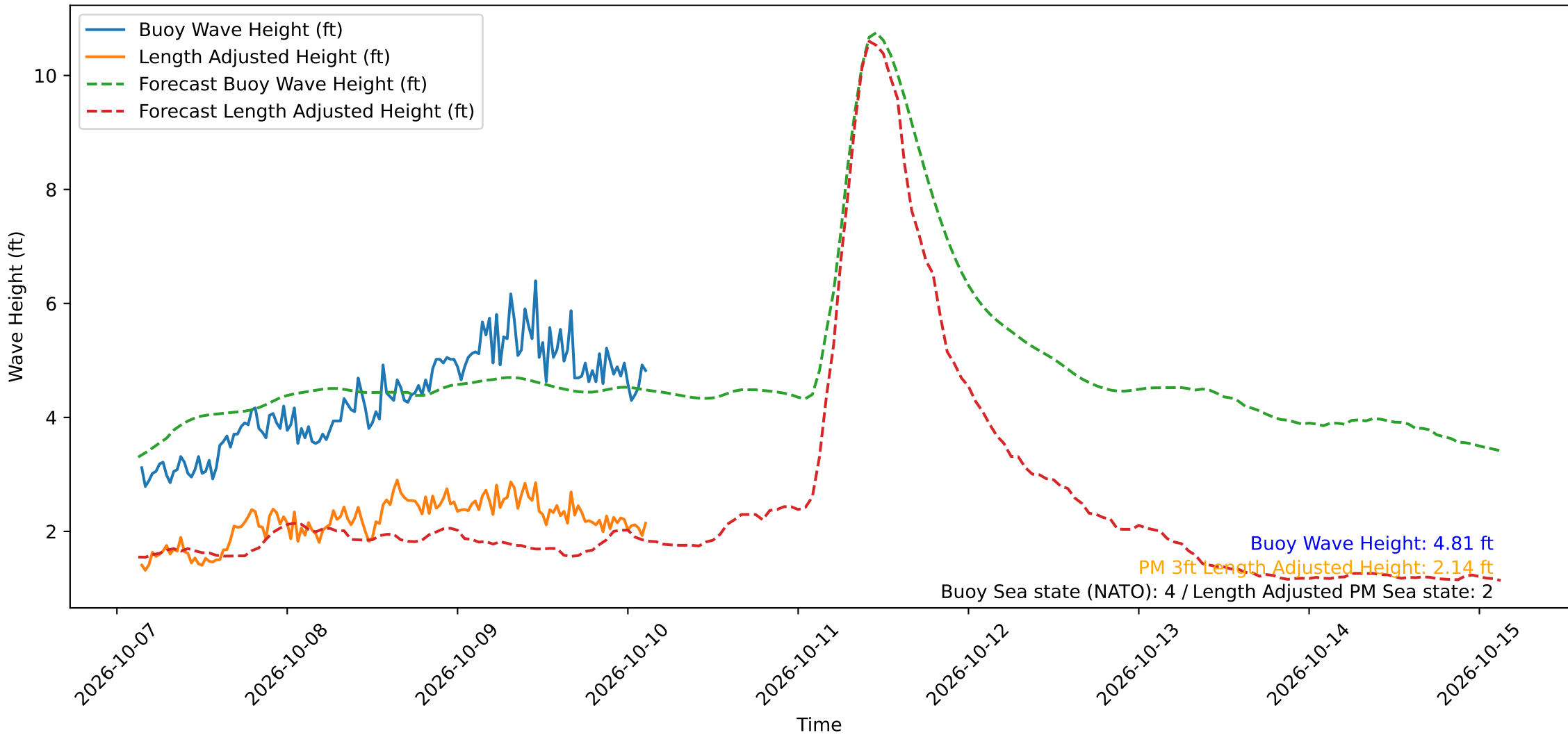
Wave Heights over Time for Oceanside Harbor at 2026-10-10 03:20:30
