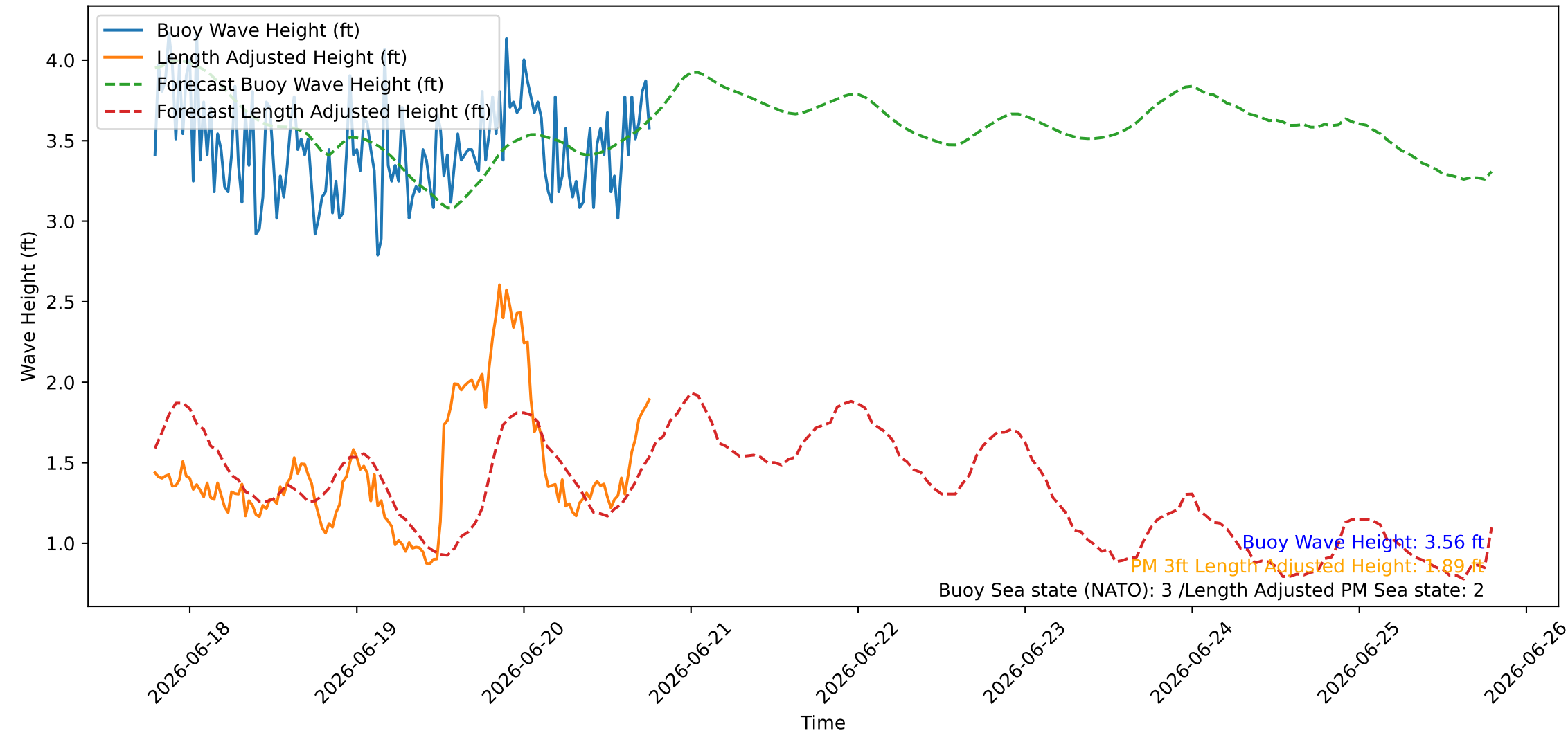
Wave Heights over Time for Oceanside Harbor at 2026-06-20 19:00:25
