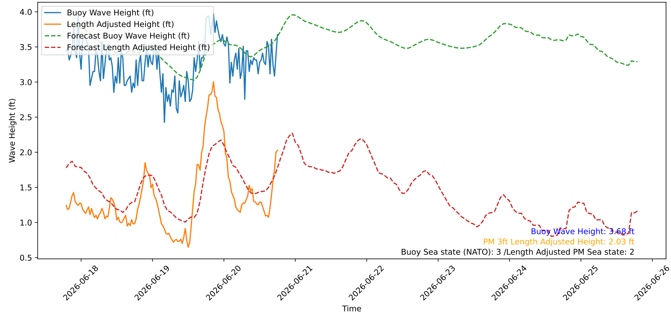
Wave Heights over Time for Green Beach at 2026-06-20 19:01:07
