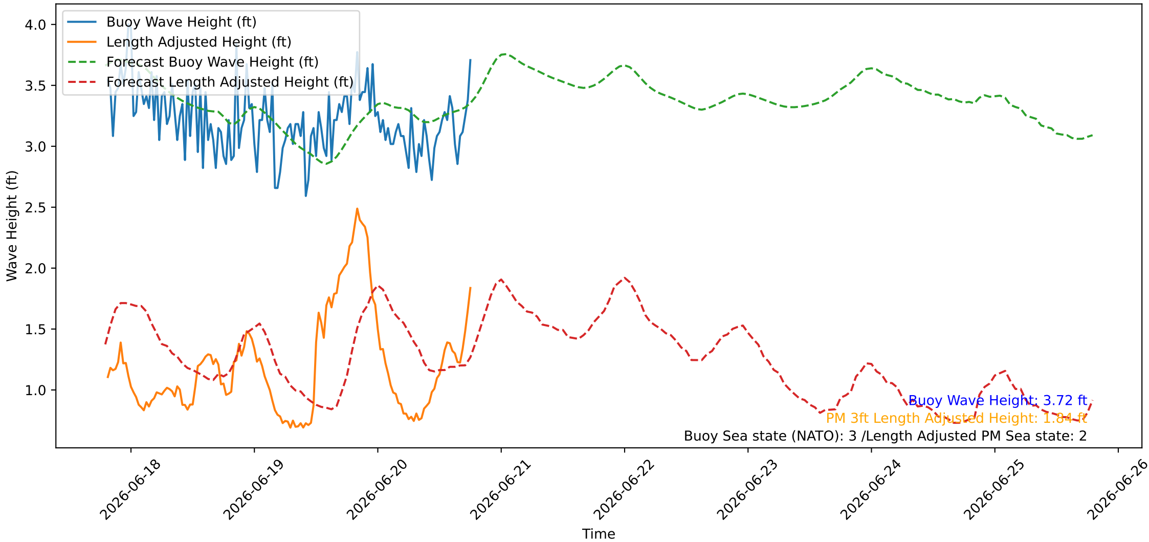
Wave Heights over Time for Red Beach at 2026-06-20 19:00:44
