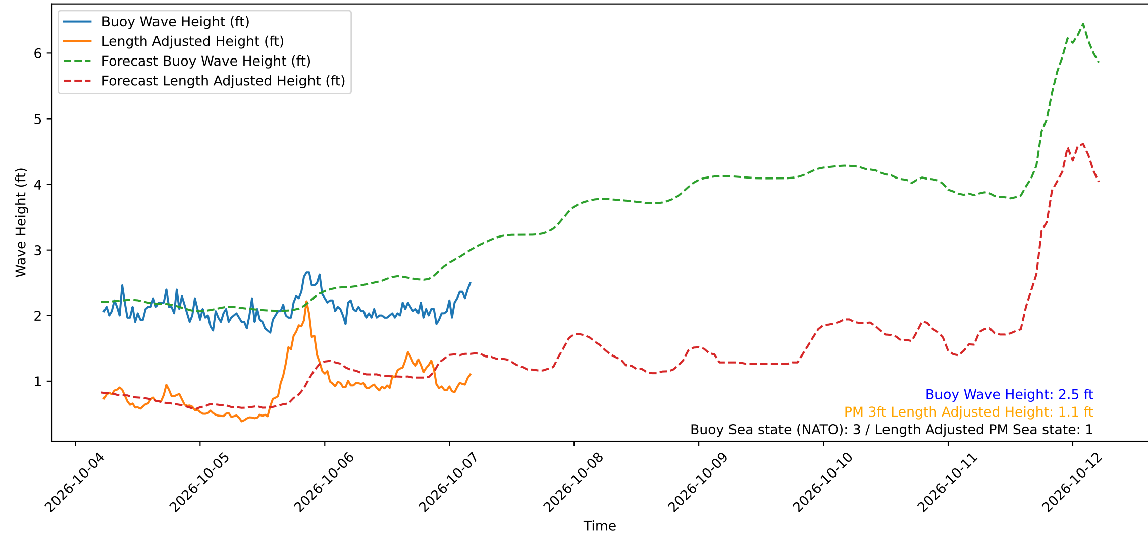
Wave Heights over Time for Red Beach at 2026-10-07 05:00:49
