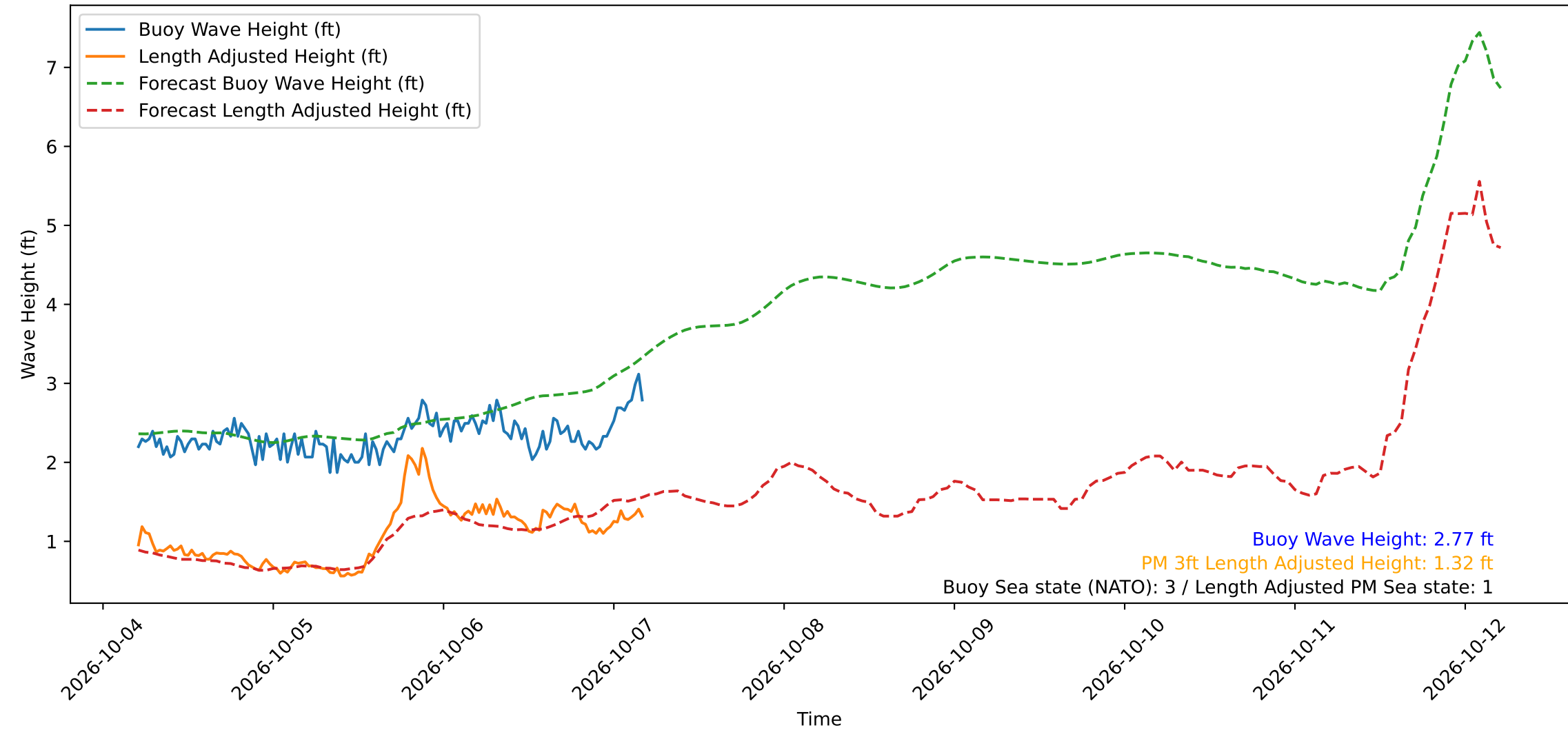
Wave Heights over Time for Oceanside Harbor at 2026-10-07 05:00:29
