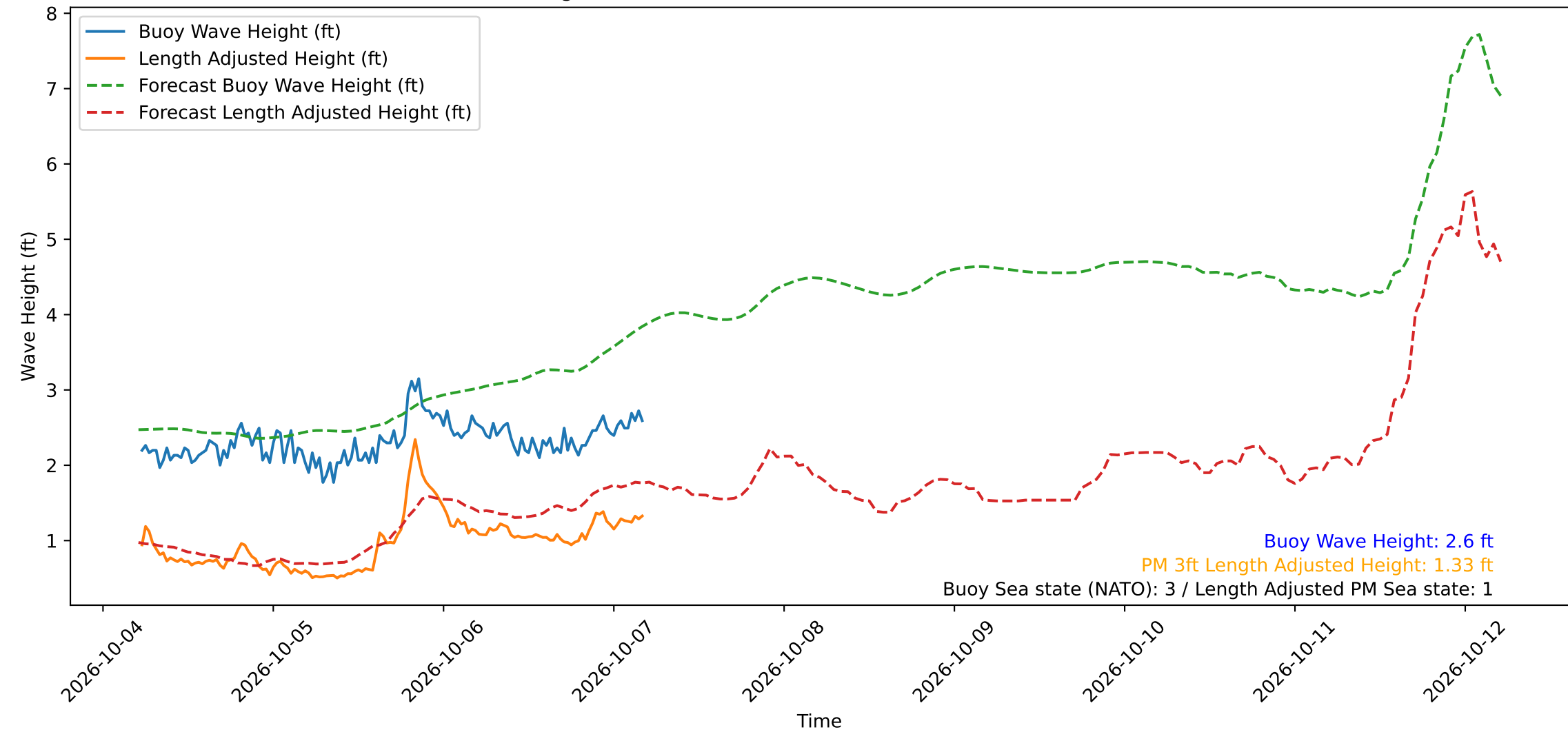
Wave Heights over Time for Green Beach at 2026-10-07 05:01:12
