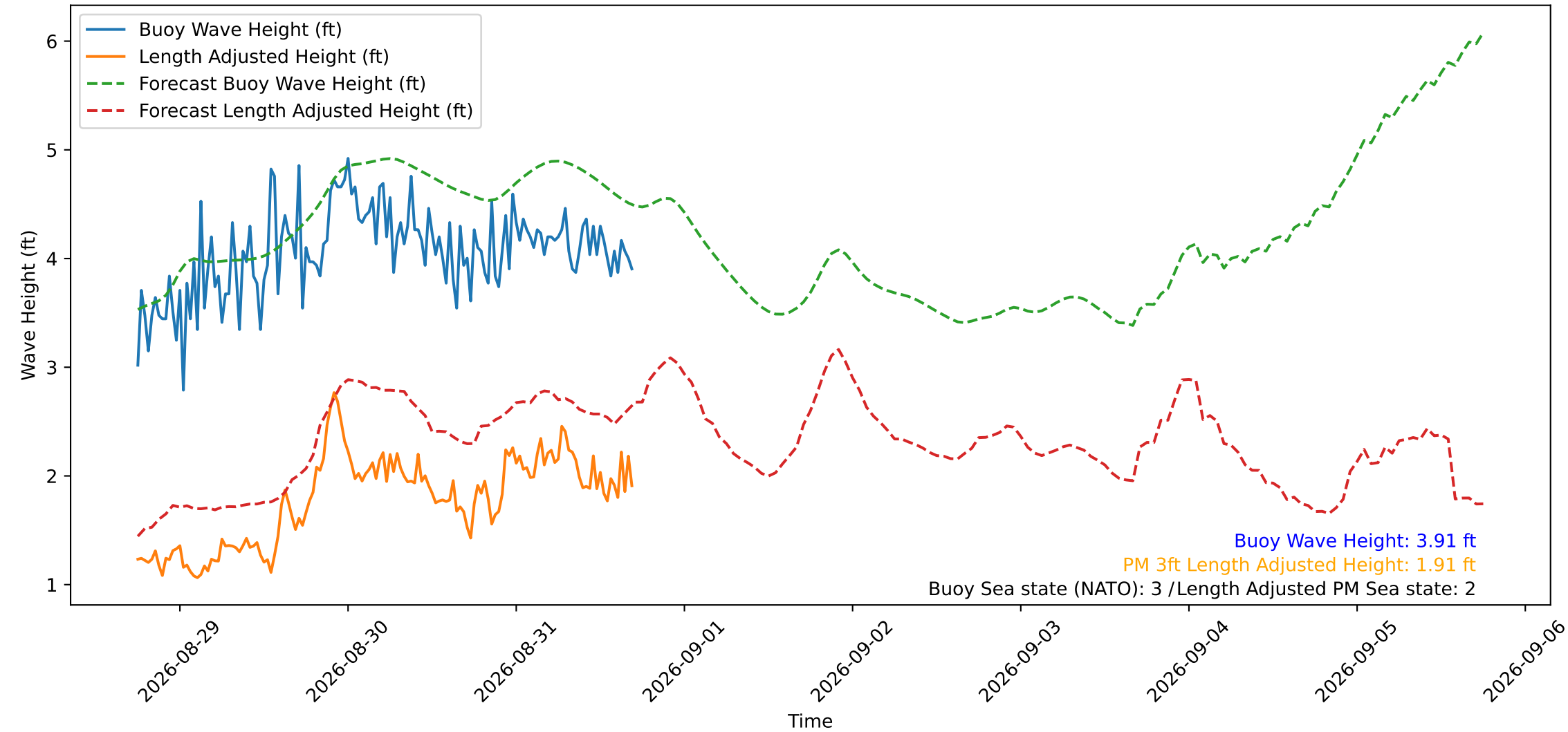
Wave Heights over Time for Green Beach at 2026-08-31 17:31:11
