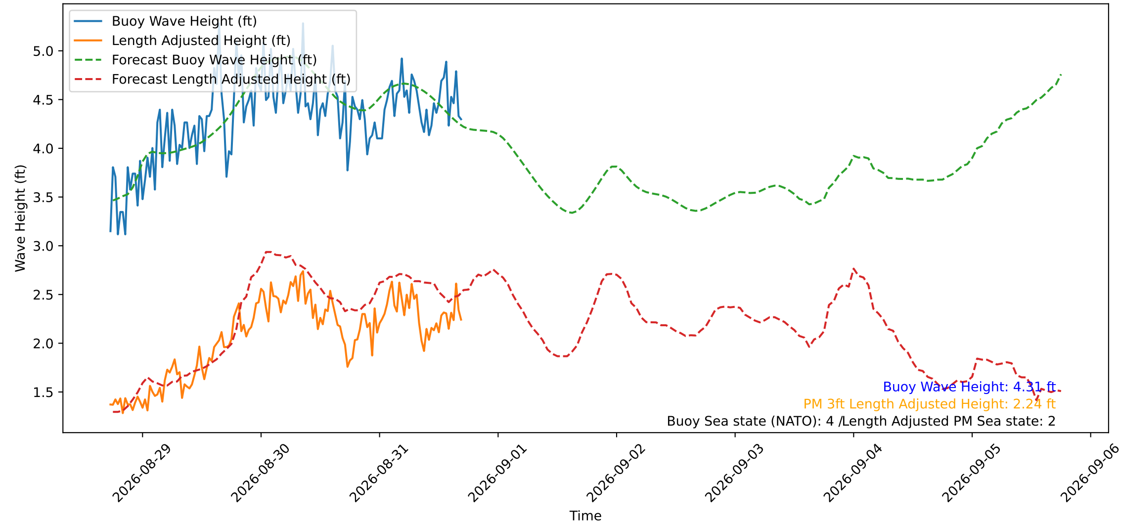
Wave Heights over Time for Oceanside Harbor at 2026-08-31 17:30:29
