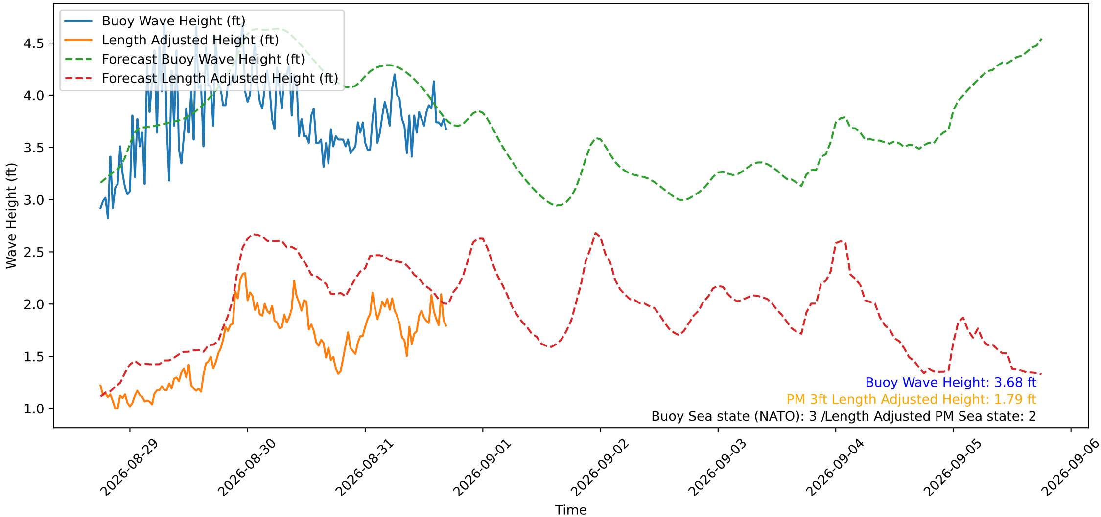
Wave Heights over Time for Red Beach at 2026-08-31 17:30:49
