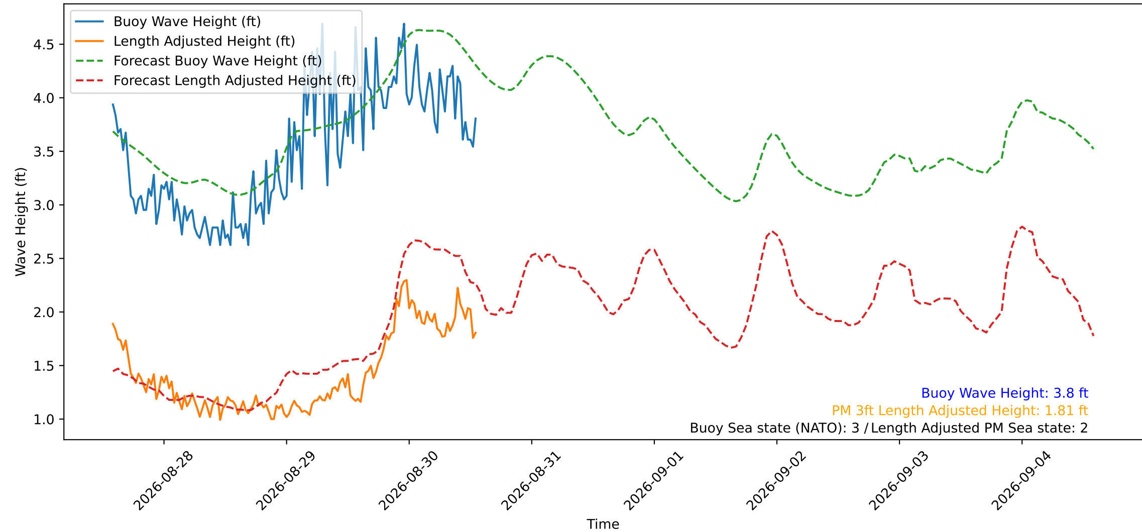
Wave Heights over Time for Red Beach at 2026-08-30 13:50:50
