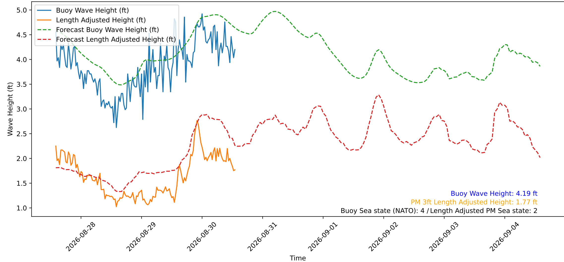
Wave Heights over Time for Green Beach at 2026-08-30 13:51:14
