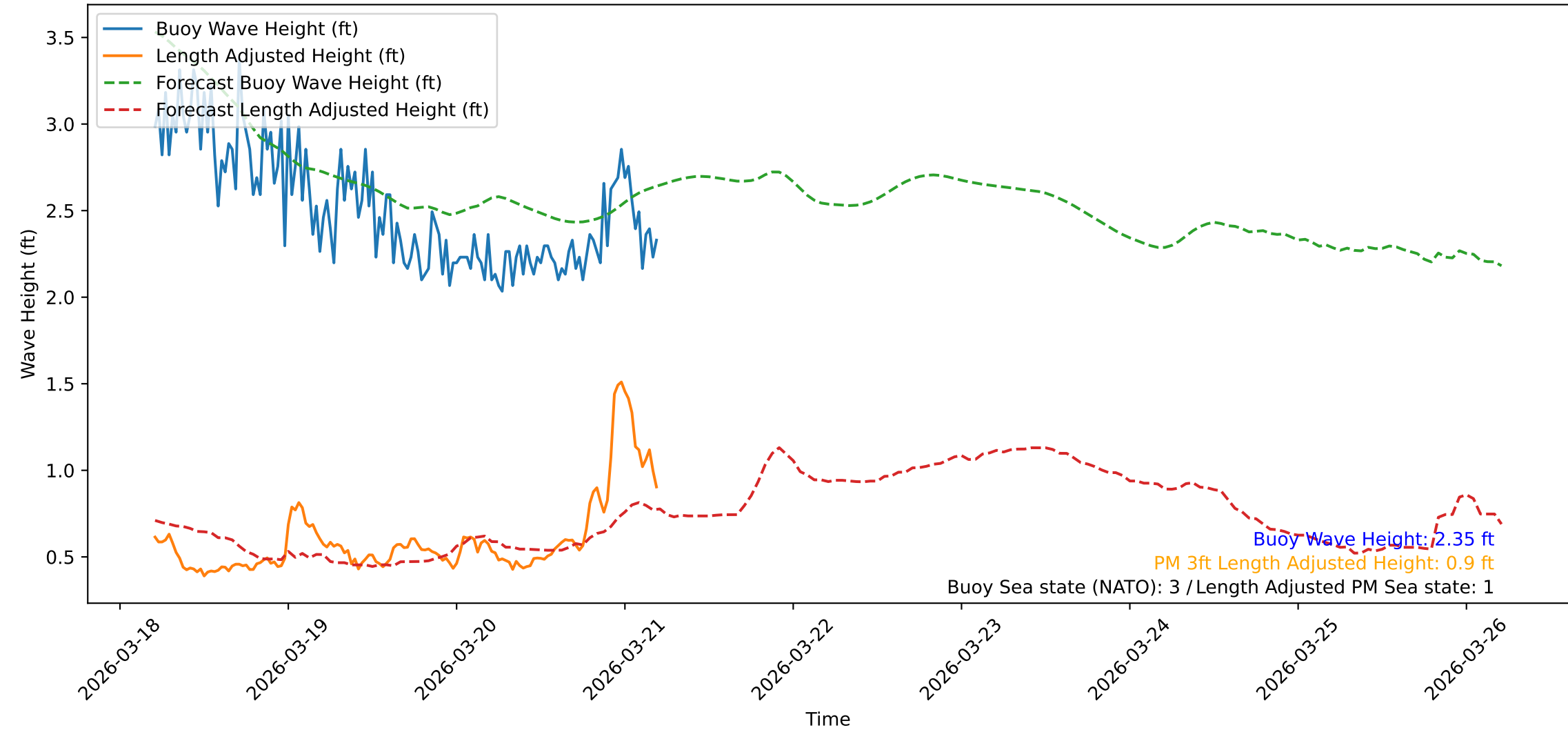
Wave Heights over Time for Green Beach at 2026-03-21 05:11:10
