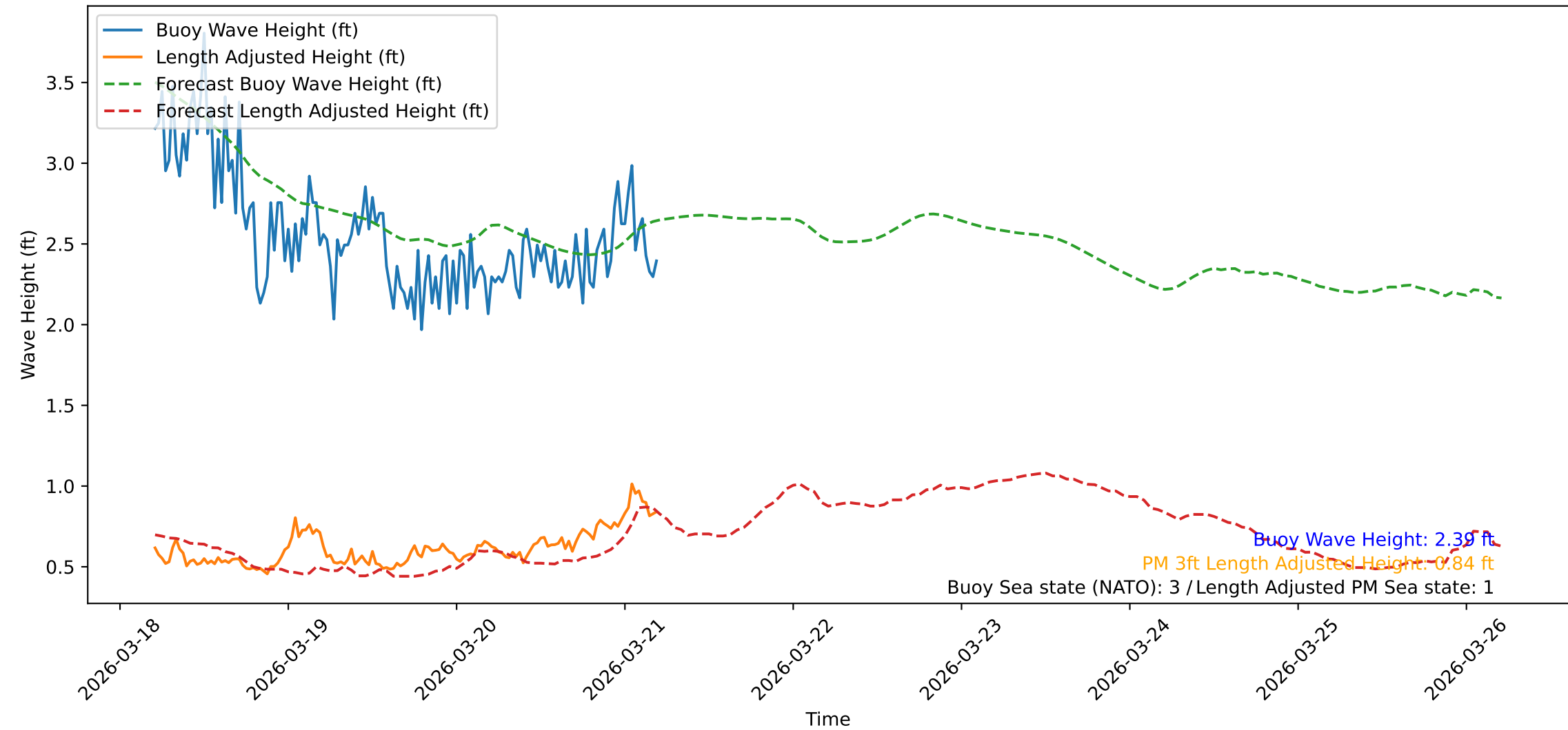
Wave Heights over Time for Oceanside Harbor at 2026-03-21 05:10:31
