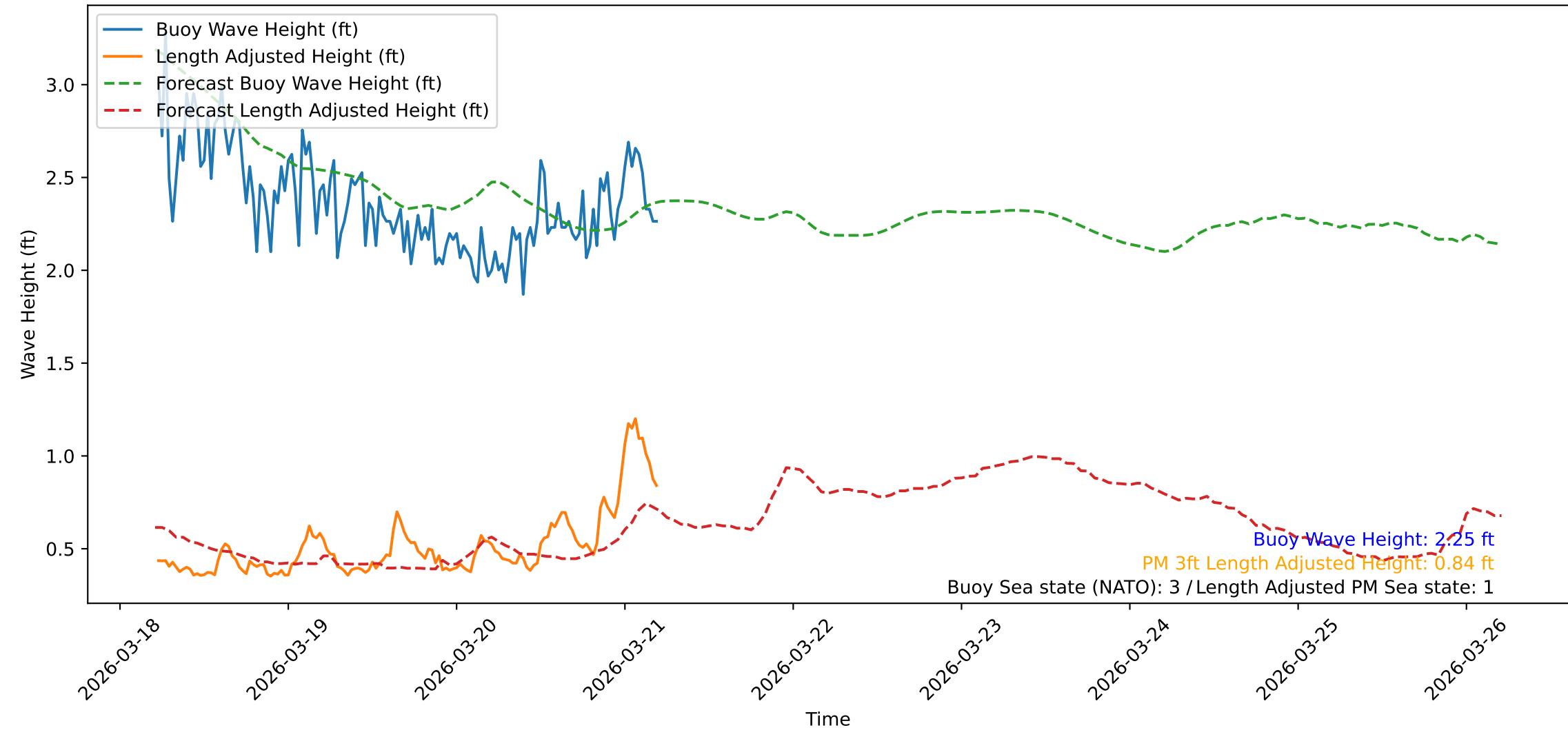
Wave Heights over Time for Red Beach at 2026-03-21 05:10:47
