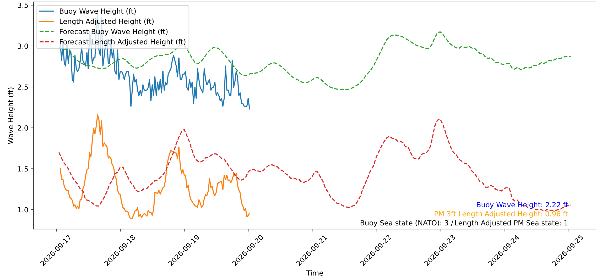
Wave Heights over Time for Red Beach at 2026-09-20 01:20:50
