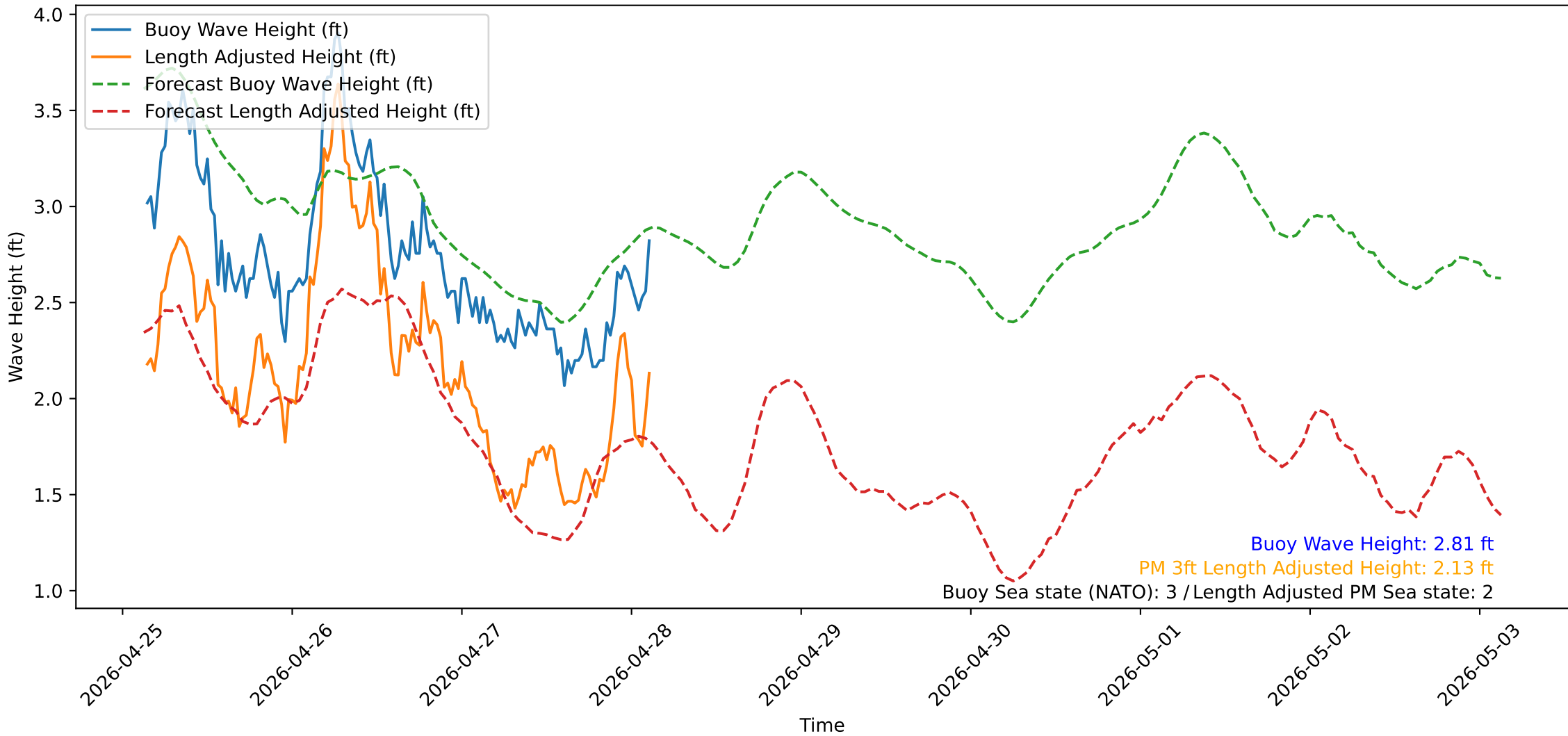
Wave Heights over Time for Oceanside Harbor at 2026-04-28 03:20:32
