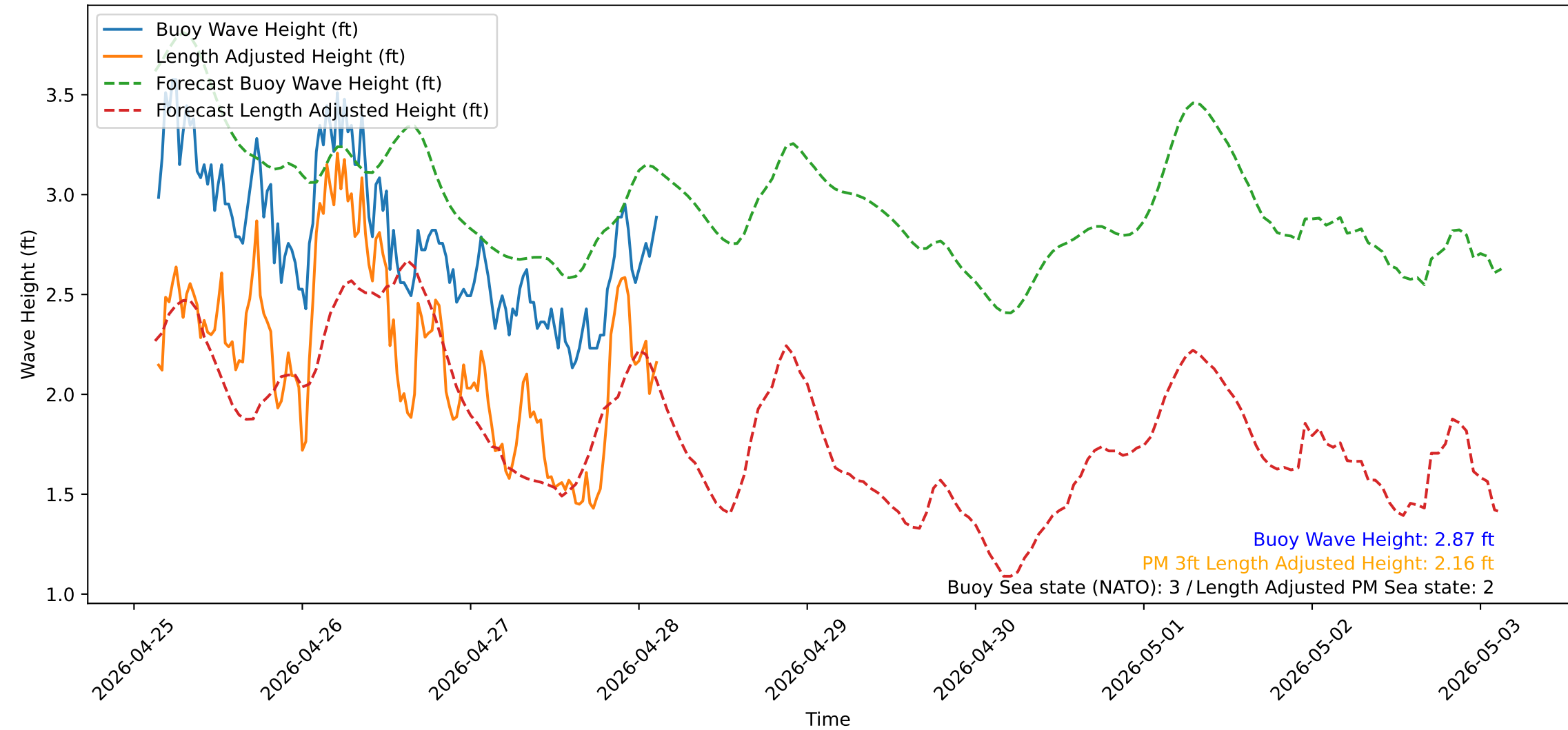
Wave Heights over Time for Green Beach at 2026-04-28 03:21:14
