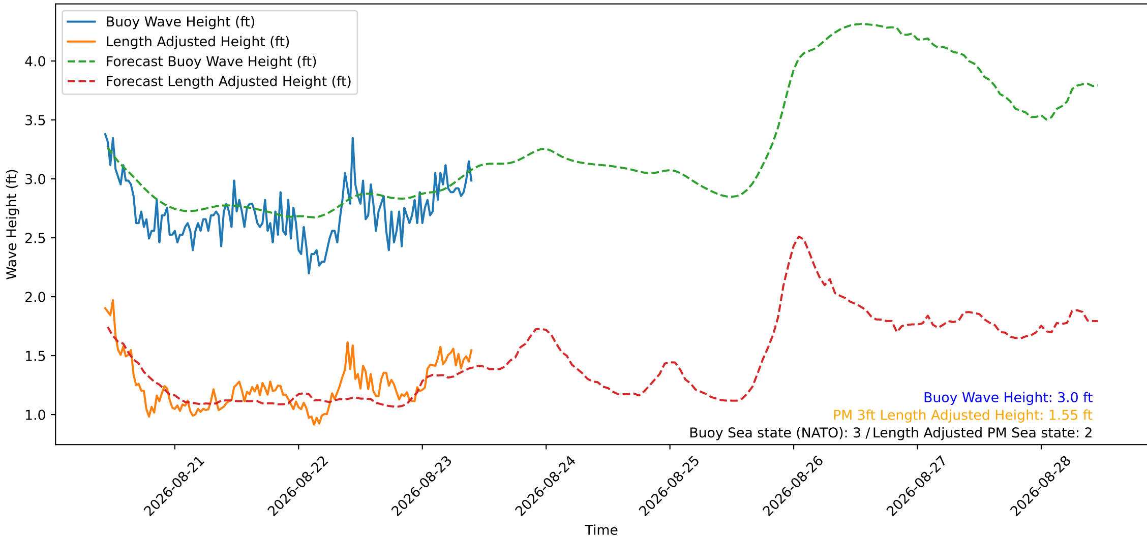
Wave Heights over Time for Oceanside Harbor at 2026-08-23 10:30:29
