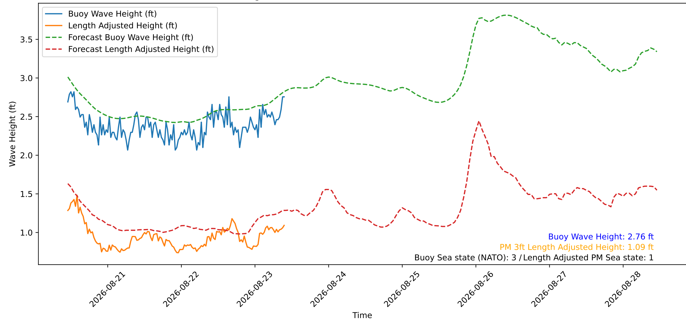
Wave Heights over Time for Red Beach at 2026-08-23 10:30:49
