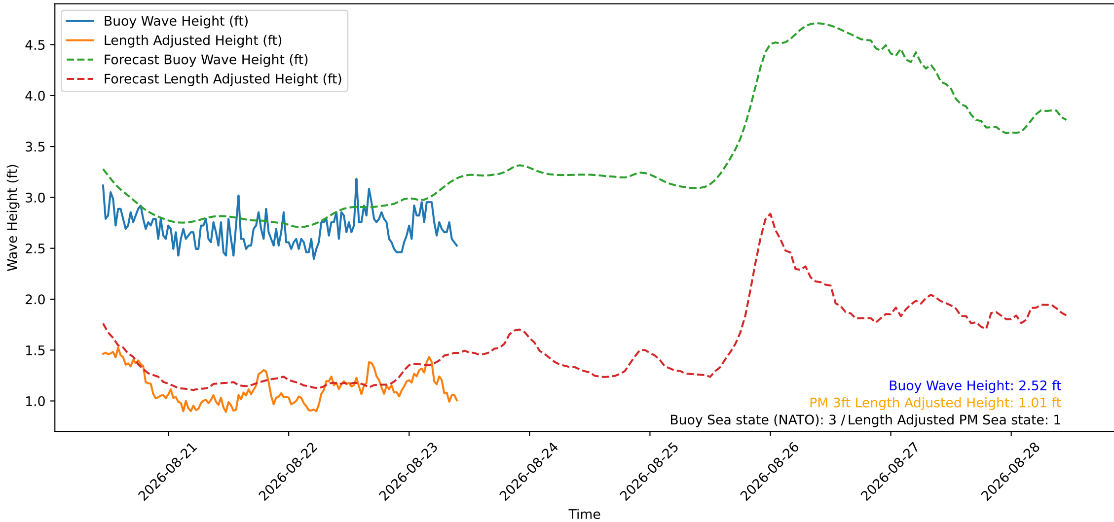
Wave Heights over Time for Green Beach at 2026-08-23 10:31:11
