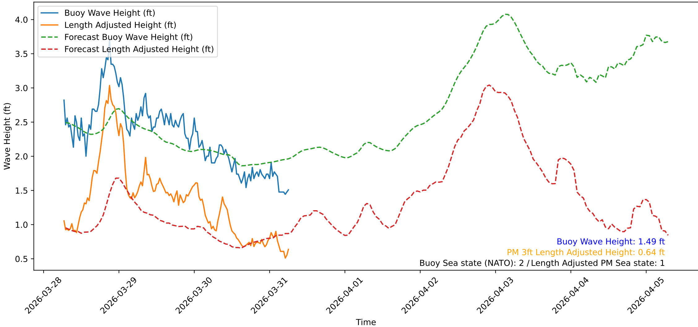
Wave Heights over Time for Green Beach at 2026-03-31 06:41:10
