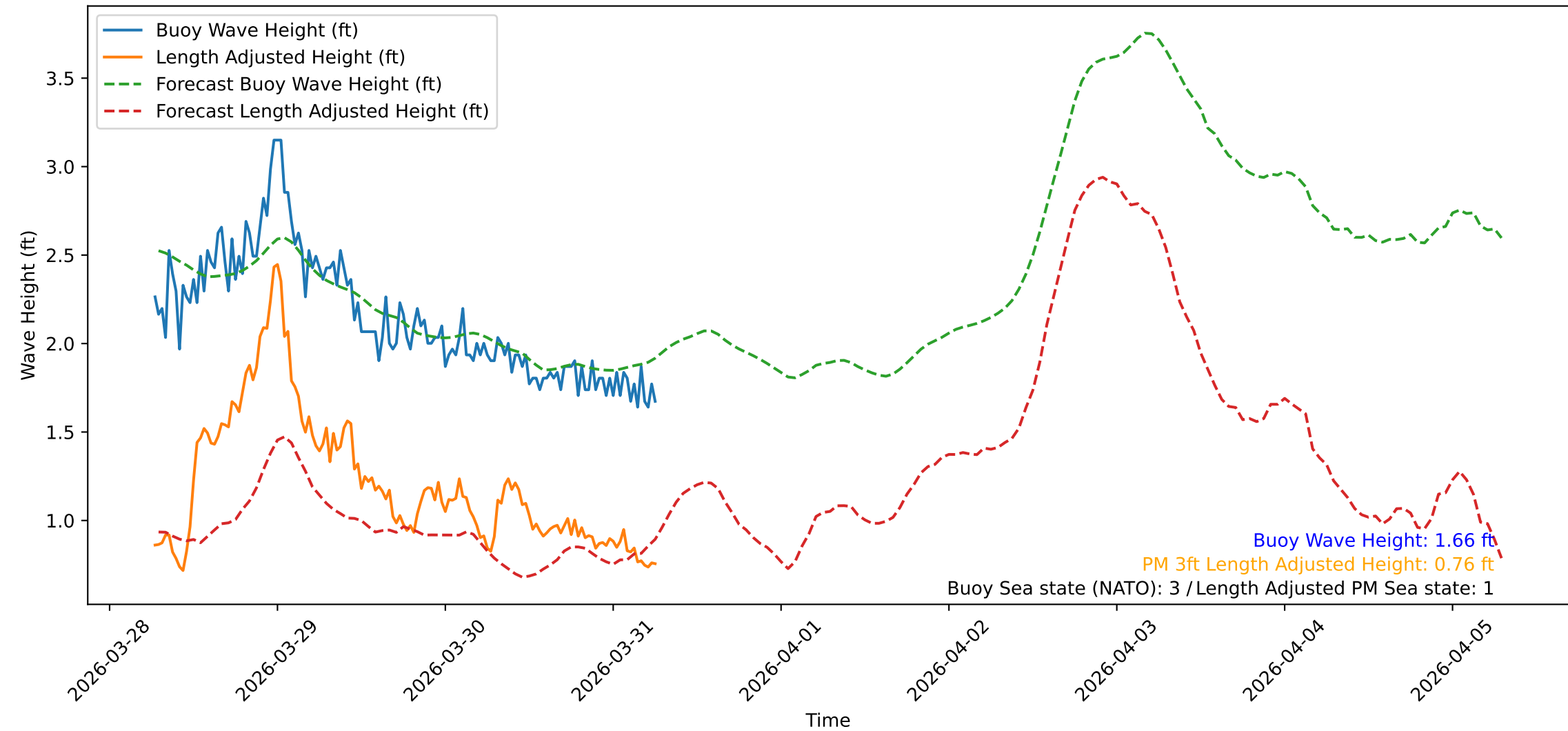
Wave Heights over Time for Oceanside Harbor at 2026-03-31 06:40:31
