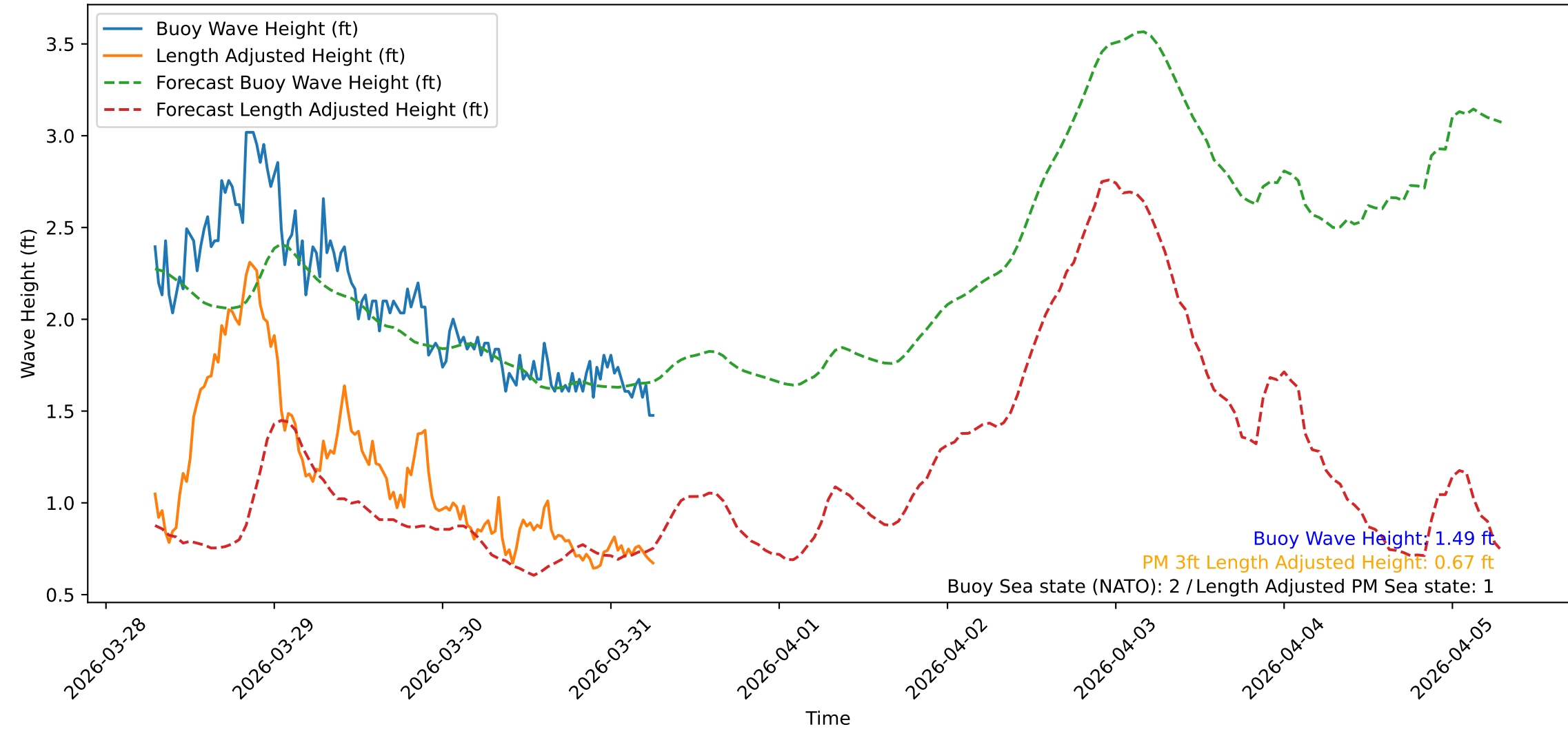
Wave Heights over Time for Red Beach at 2026-03-31 06:40:48
