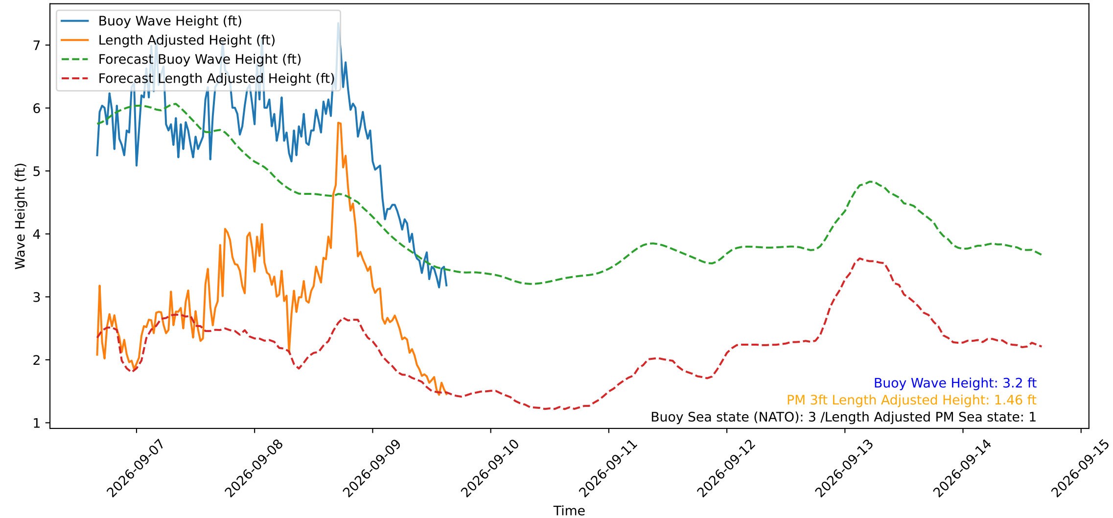
Wave Heights over Time for Oceanside Harbor at 2026-09-09 15:50:29
