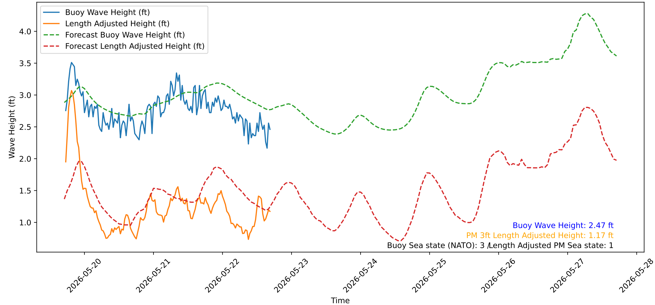
Wave Heights over Time for Red Beach at 2026-05-22 17:10:51
