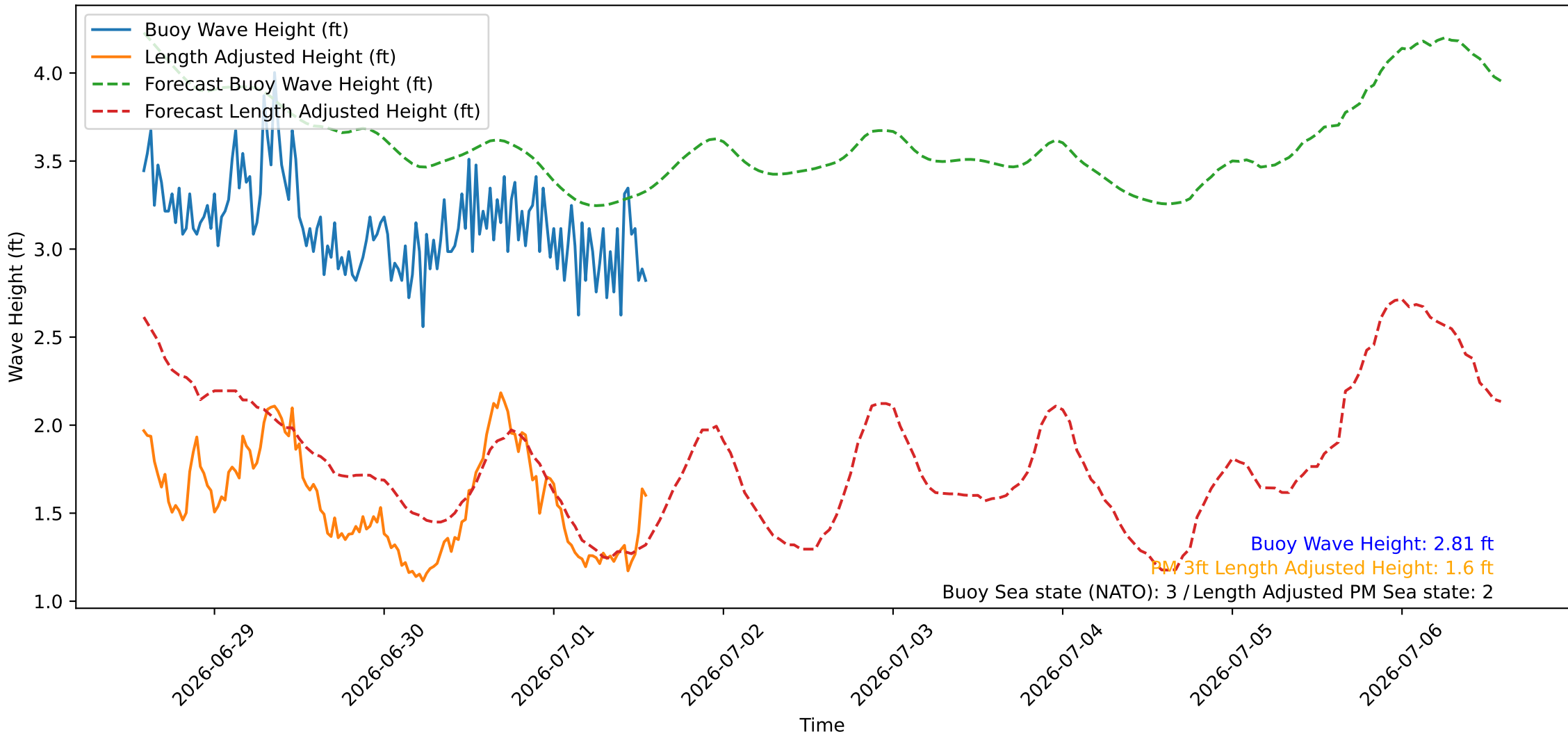
Wave Heights over Time for Oceanside Harbor at 2026-07-01 14:00:26
