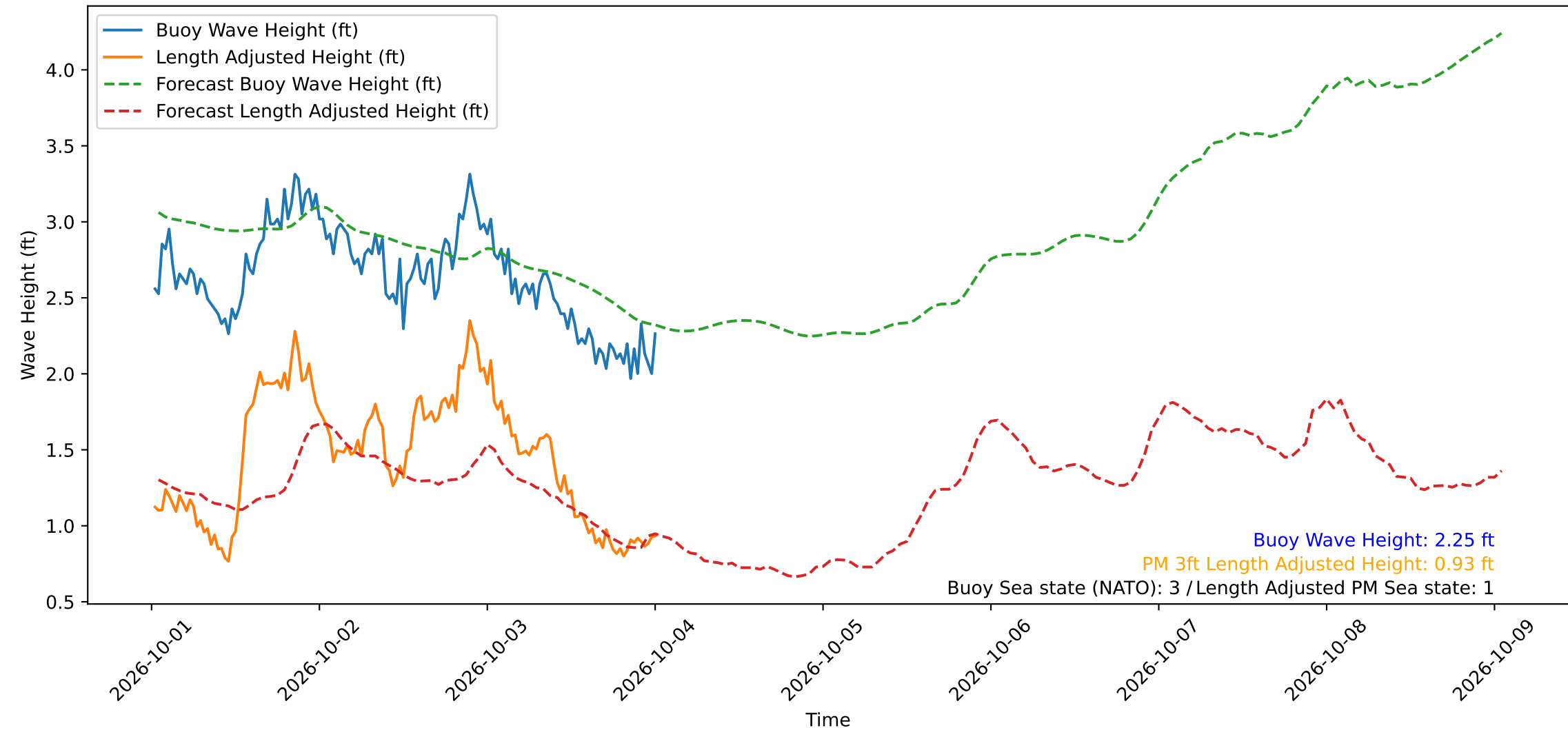
Wave Heights over Time for Oceanside Harbor at 2026-10-04 00:40:29
