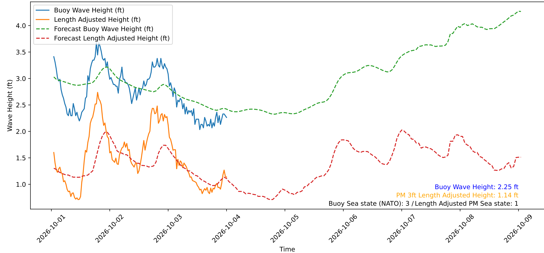
Wave Heights over Time for Green Beach at 2026-10-04 00:41:11
