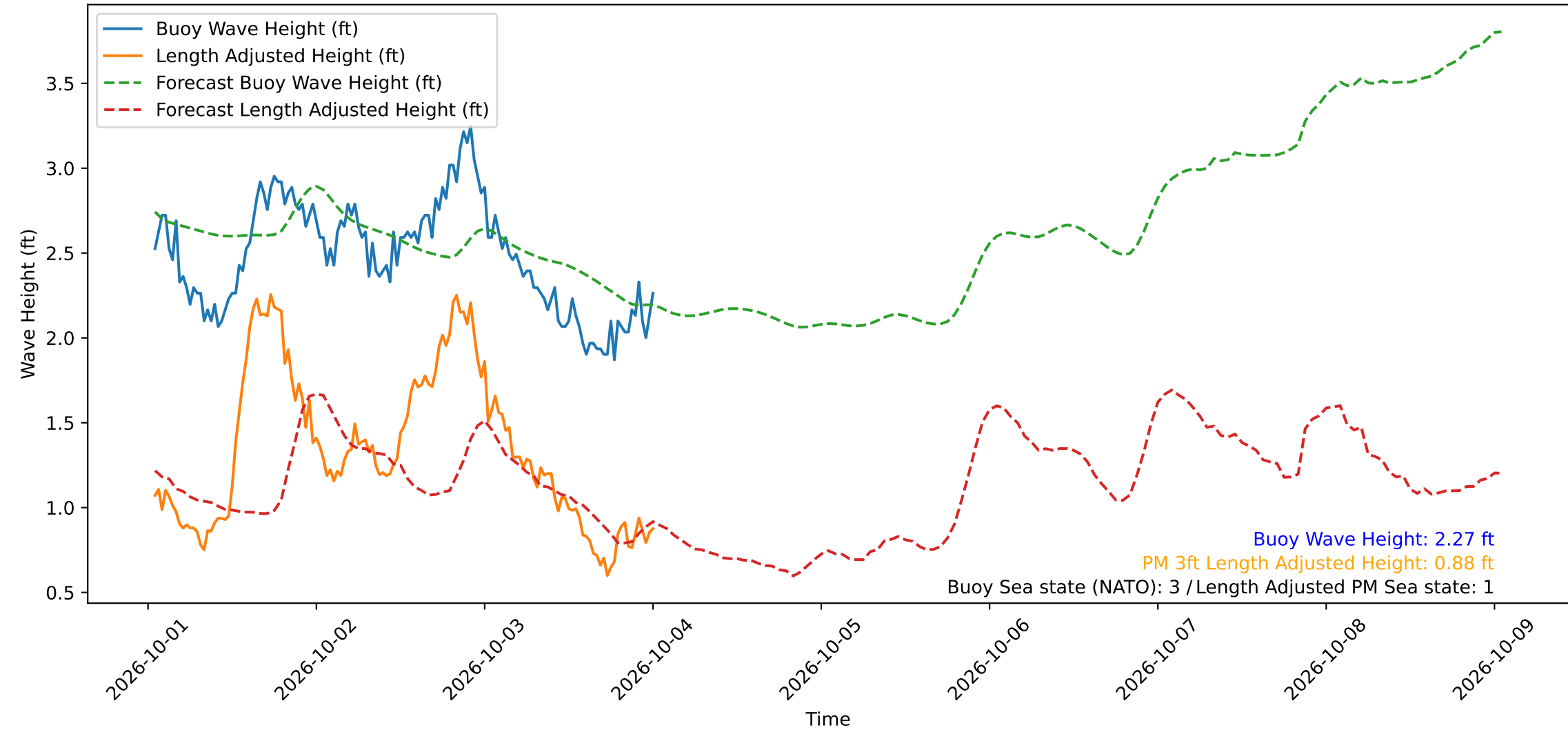
Wave Heights over Time for Red Beach at 2026-10-04 00:40:49
