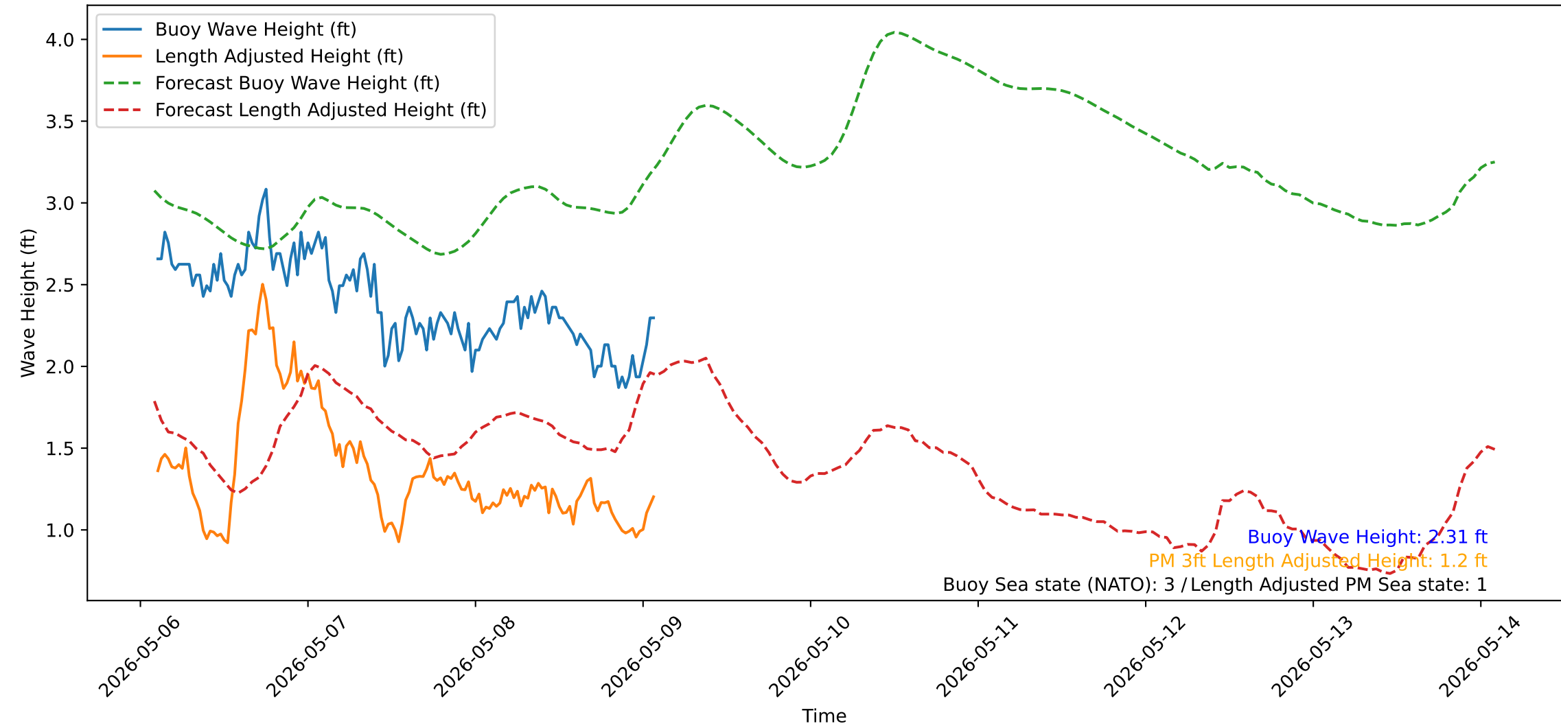
Wave Heights over Time for Oceanside Harbor at 2026-05-09 02:20:31
