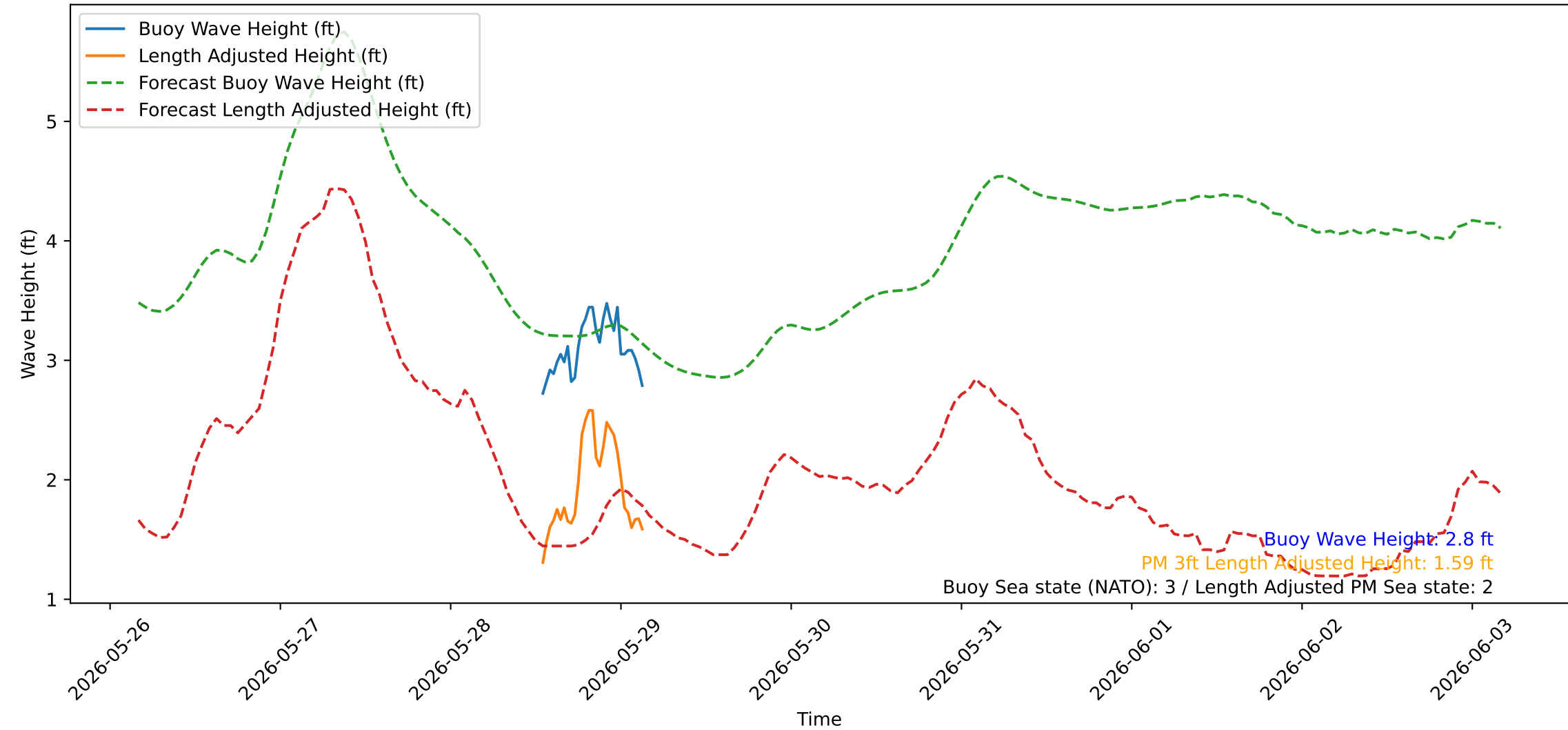
Wave Heights over Time for Oceanside Harbor at 2026-05-29 03:50:20
