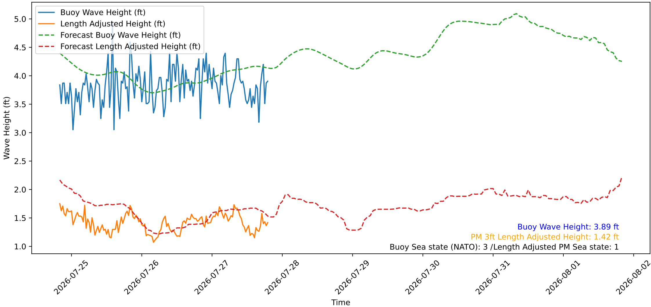
Wave Heights over Time for Oceanside Harbor at 2026-07-27 20:10:26
