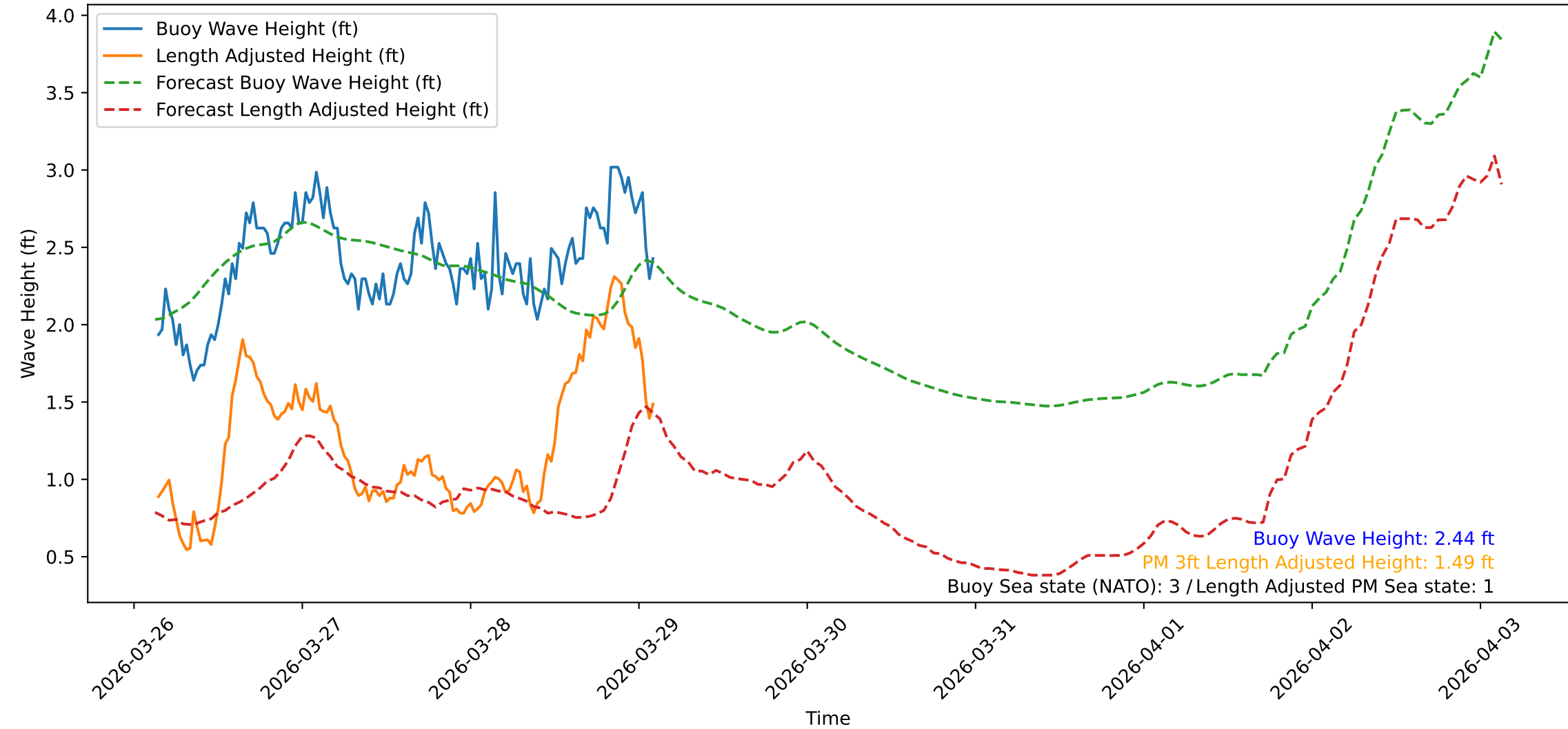
Wave Heights over Time for Red Beach at 2026-03-29 03:10:48
