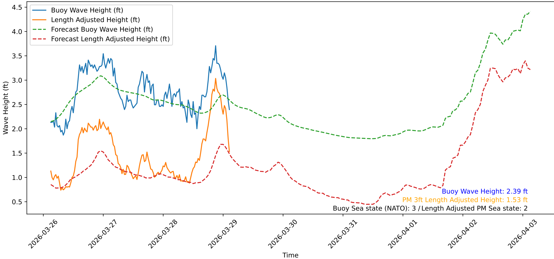
Wave Heights over Time for Green Beach at 2026-03-29 03:11:10
