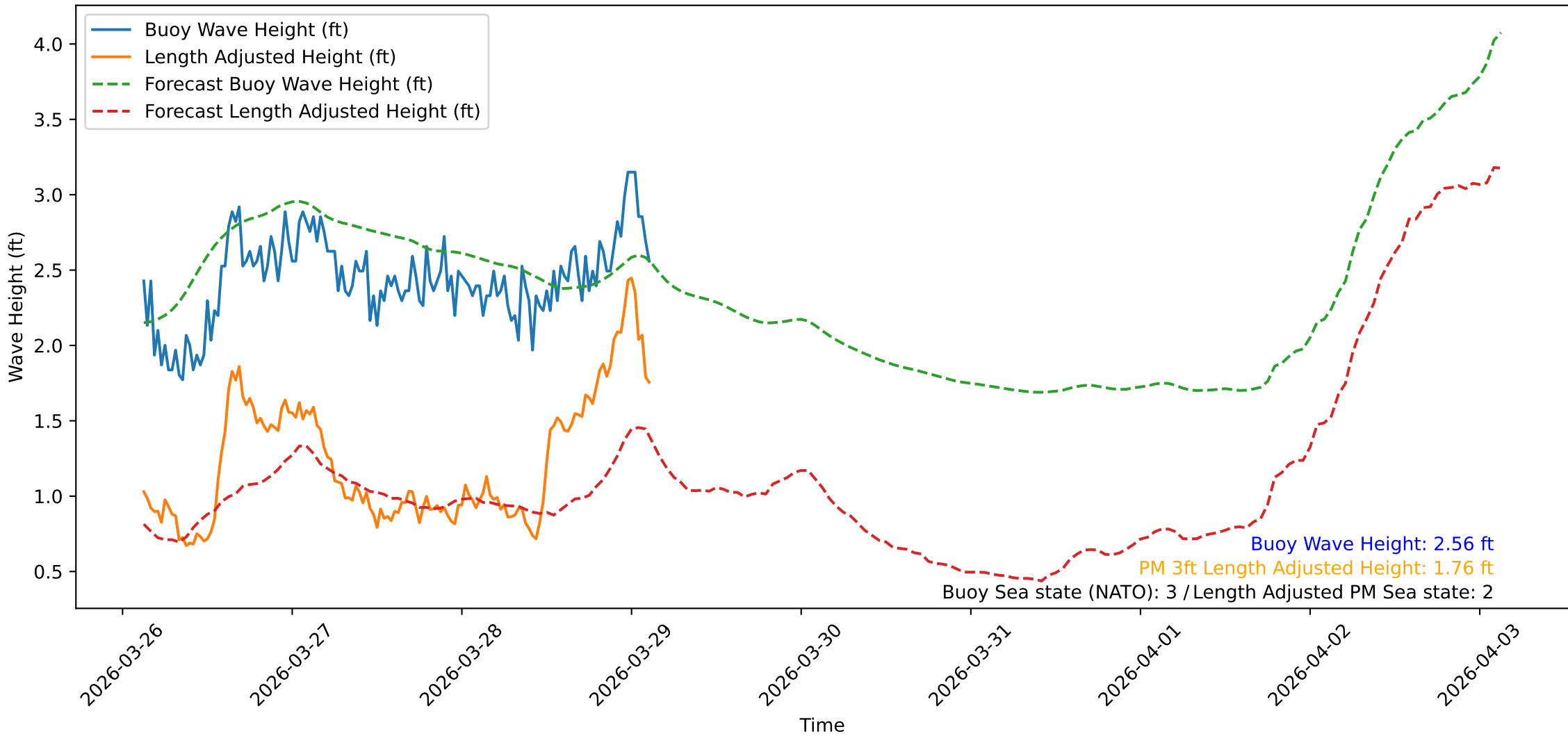
Wave Heights over Time for Oceanside Harbor at 2026-03-29 03:10:32
