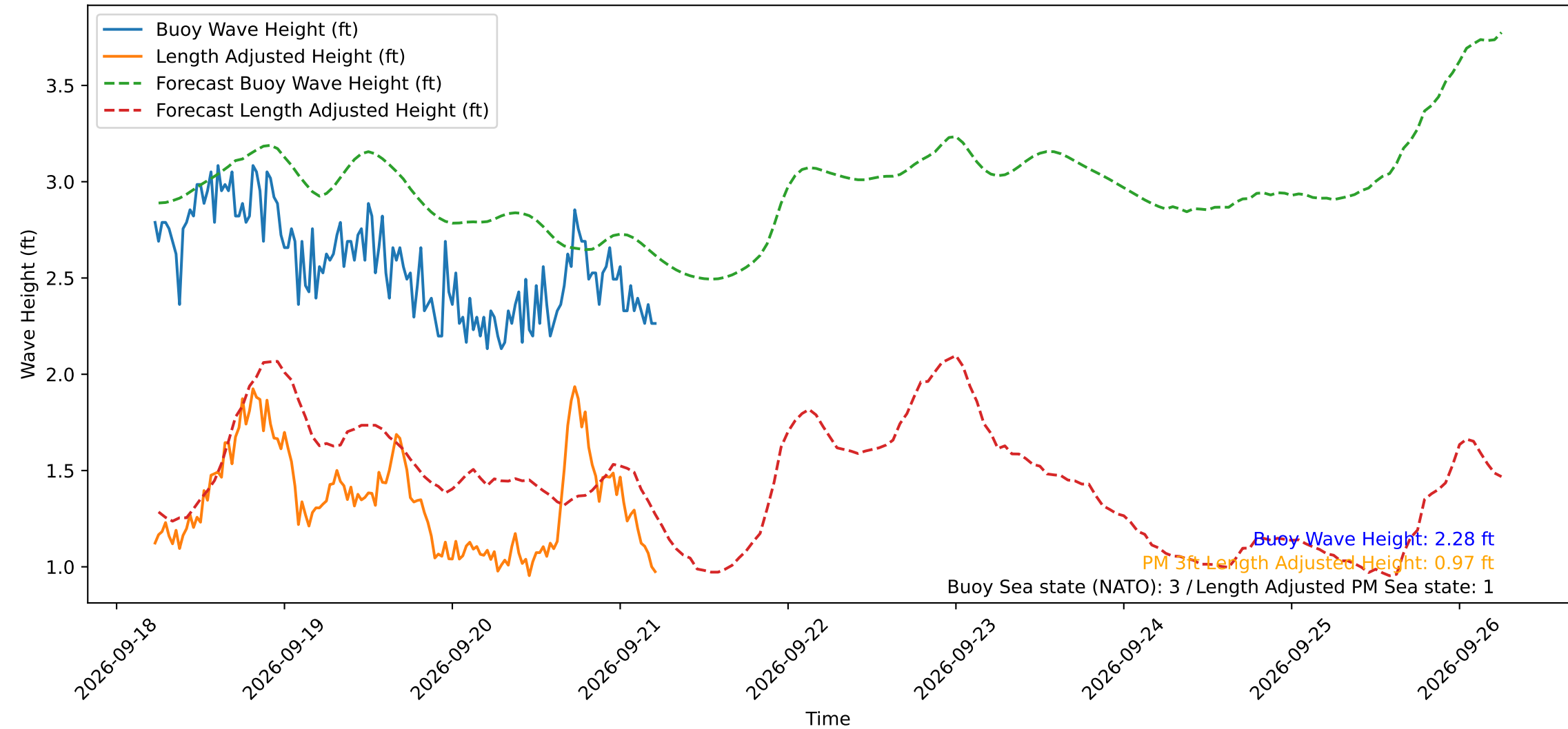
Wave Heights over Time for Oceanside Harbor at 2026-09-21 05:30:29
