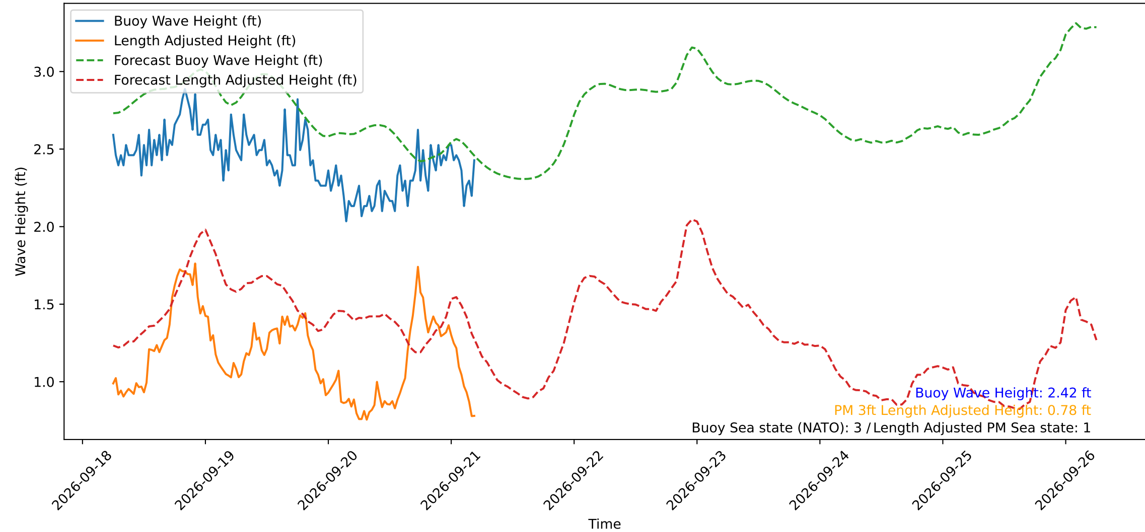
Wave Heights over Time for Red Beach at 2026-09-21 05:30:48
