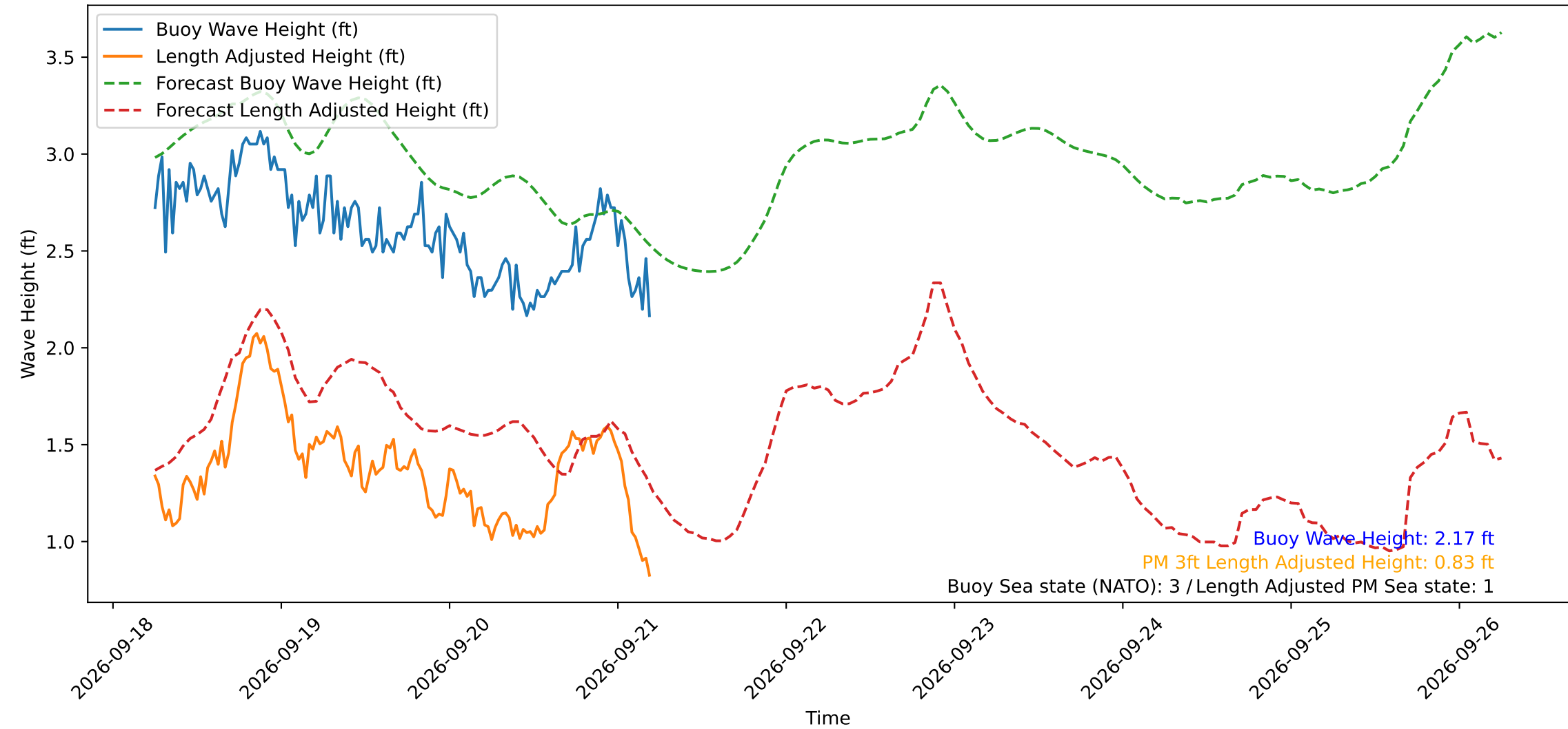
Wave Heights over Time for Green Beach at 2026-09-21 05:31:11
