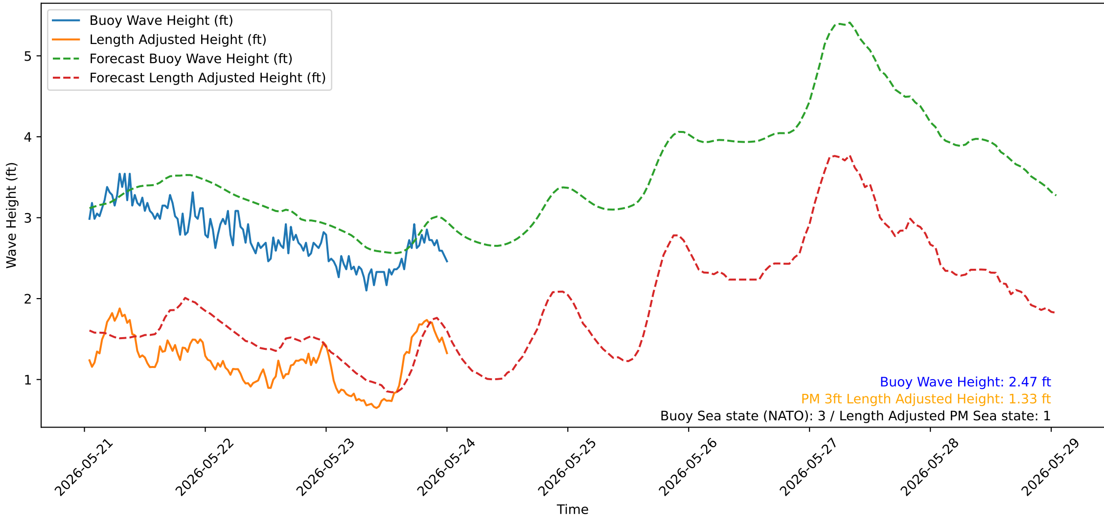
Wave Heights over Time for Green Beach at 2026-05-24 01:01:14
