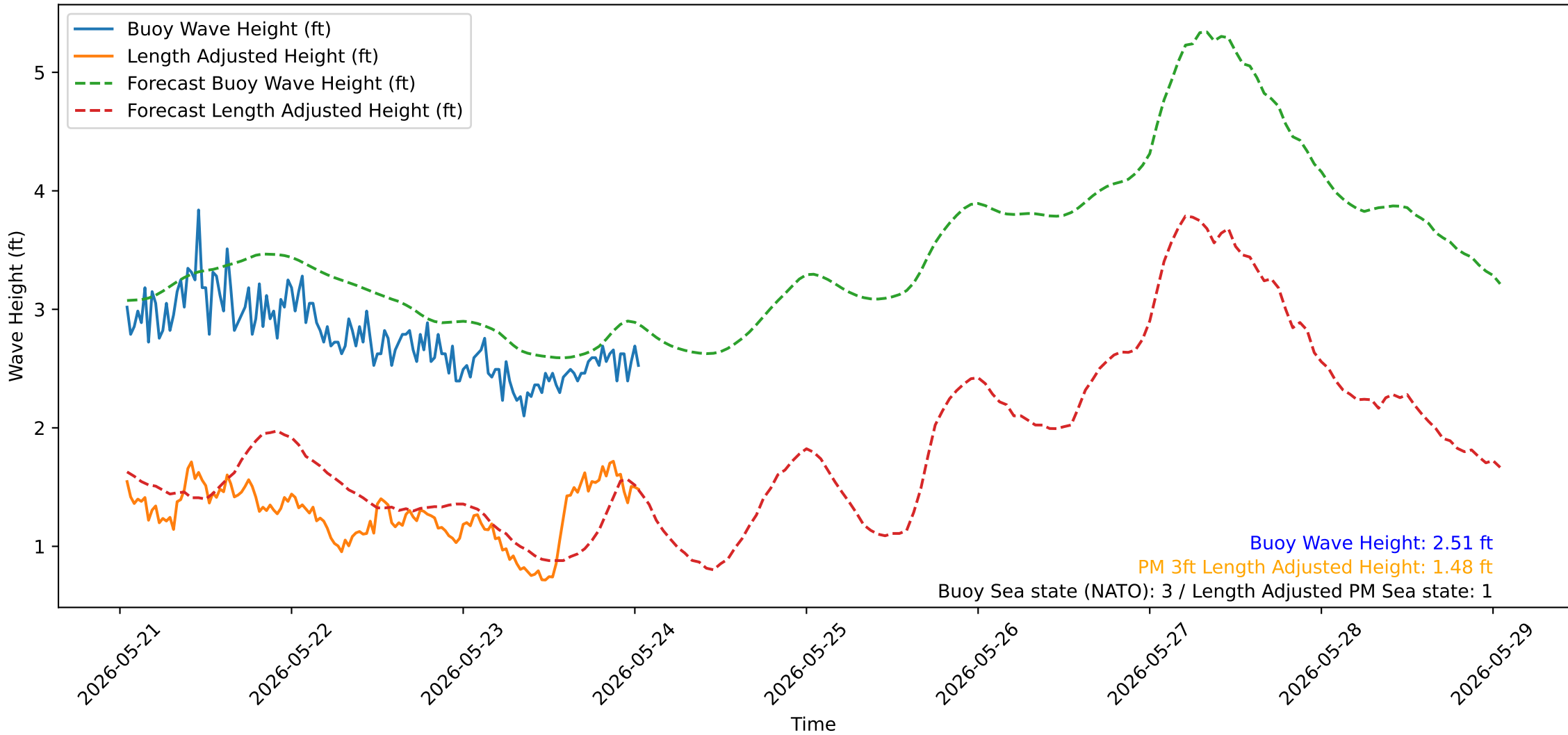
Wave Heights over Time for Oceanside Harbor at 2026-05-24 01:00:31
