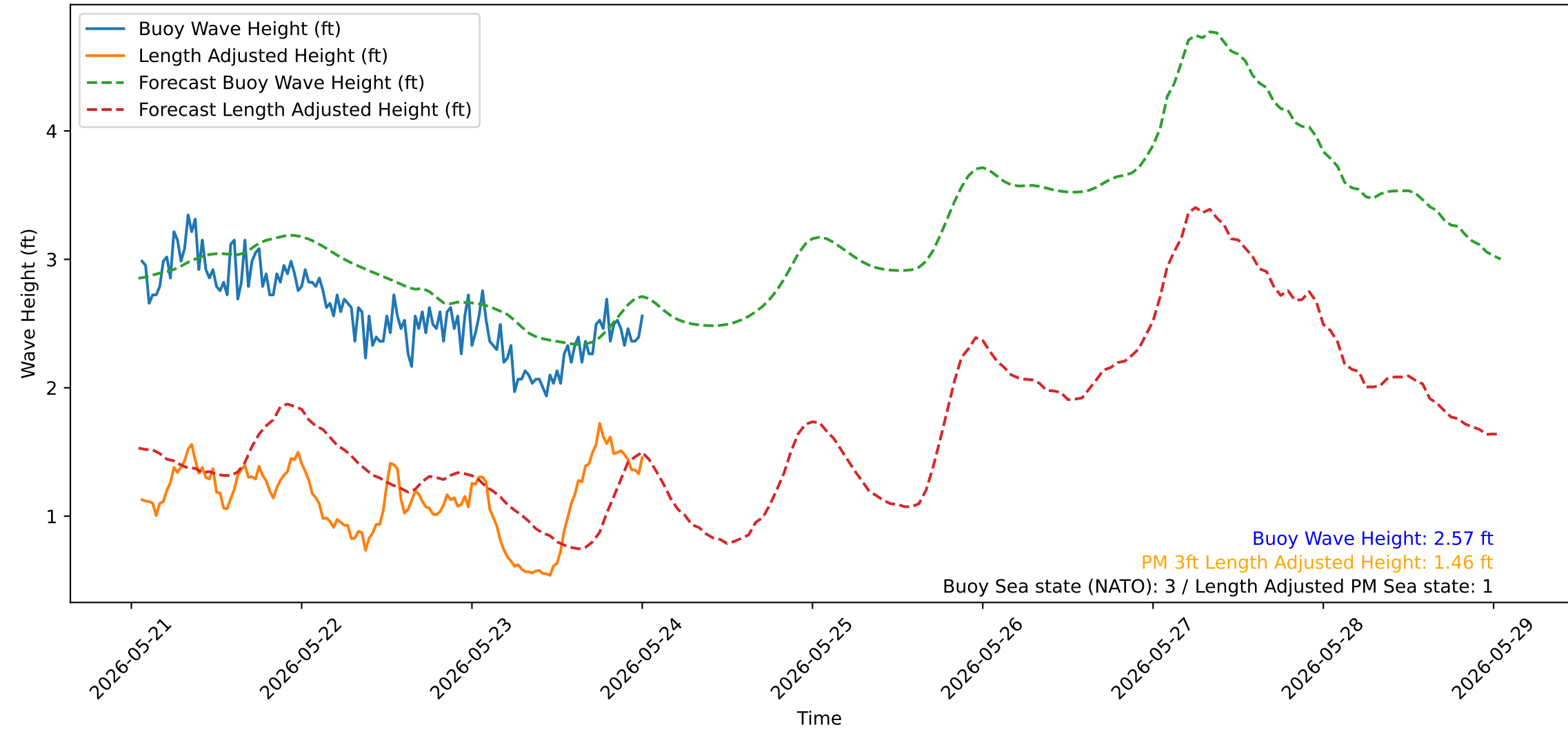
Wave Heights over Time for Red Beach at 2026-05-24 01:00:51
