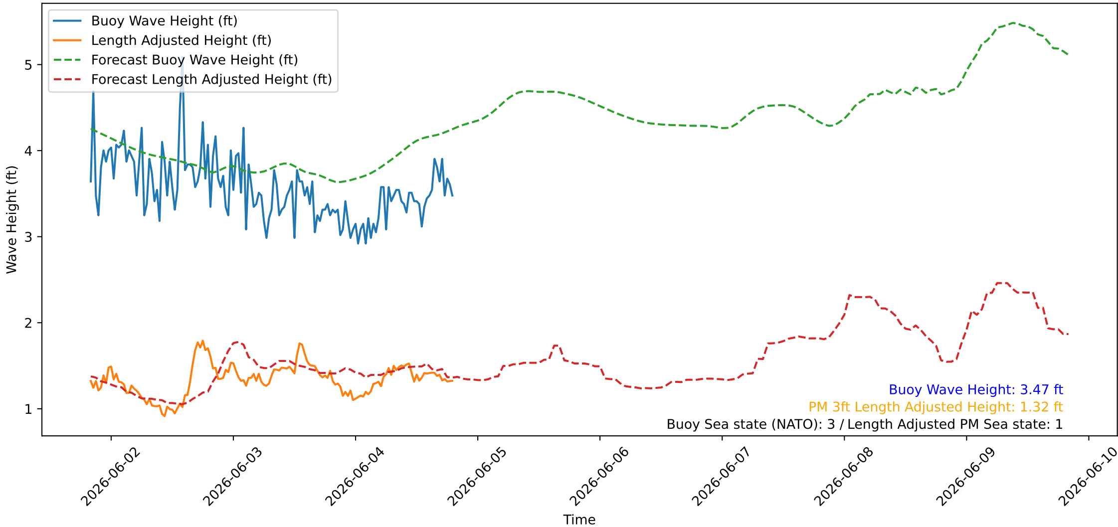
Wave Heights over Time for Oceanside Harbor at 2026-06-04 19:50:26
