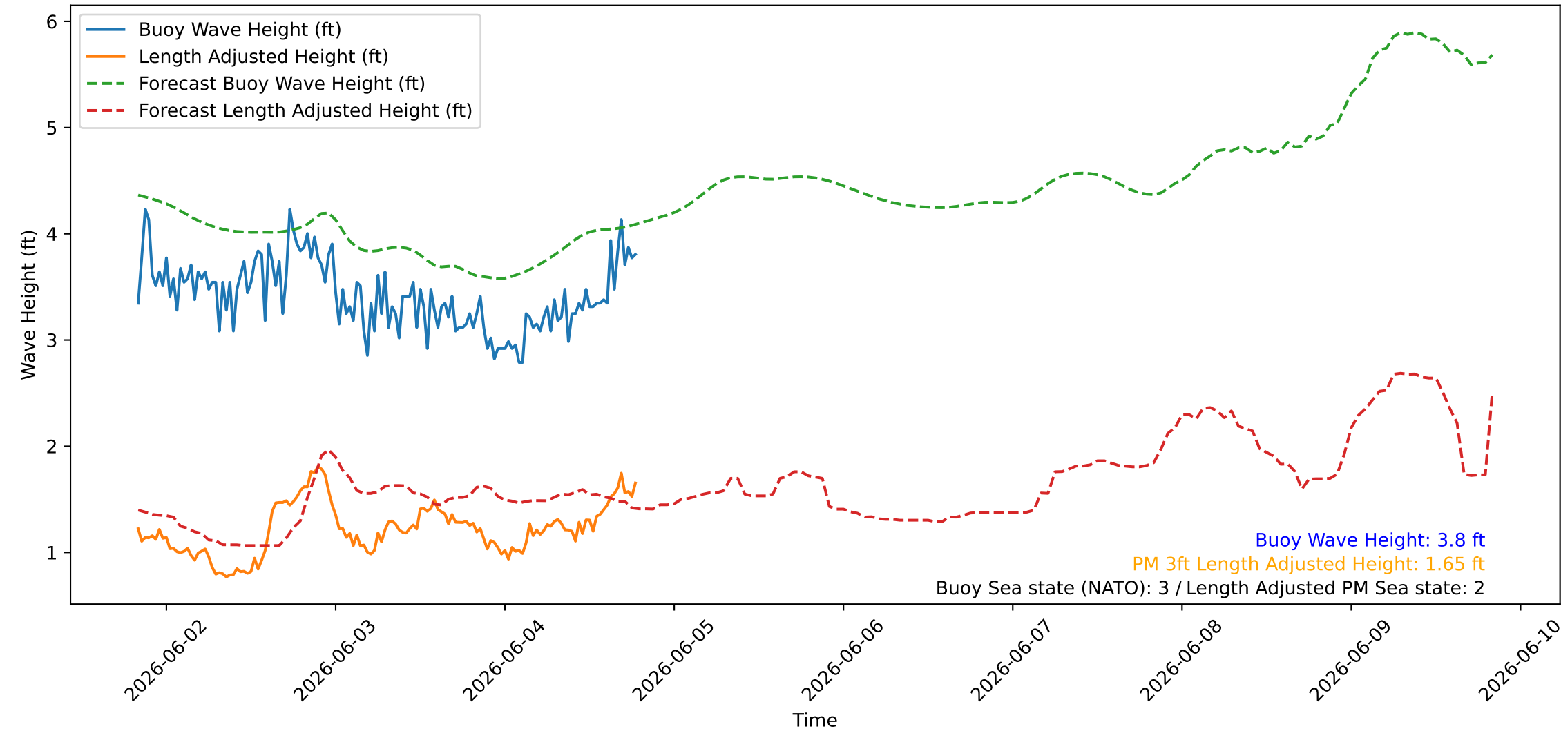
Wave Heights over Time for Green Beach at 2026-06-04 19:51:10
