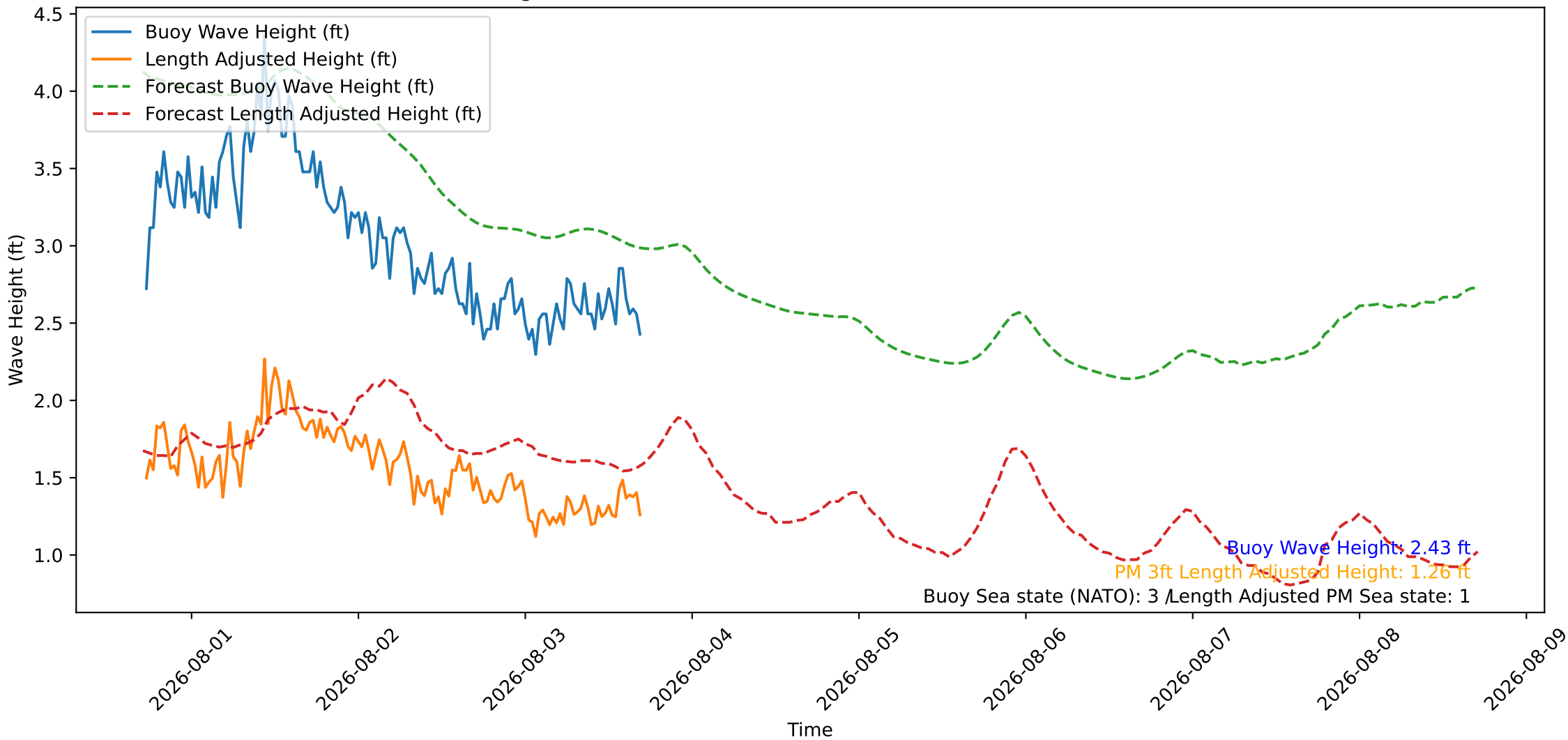
Wave Heights over Time for Oceanside Harbor at 2026-08-03 17:20:26
