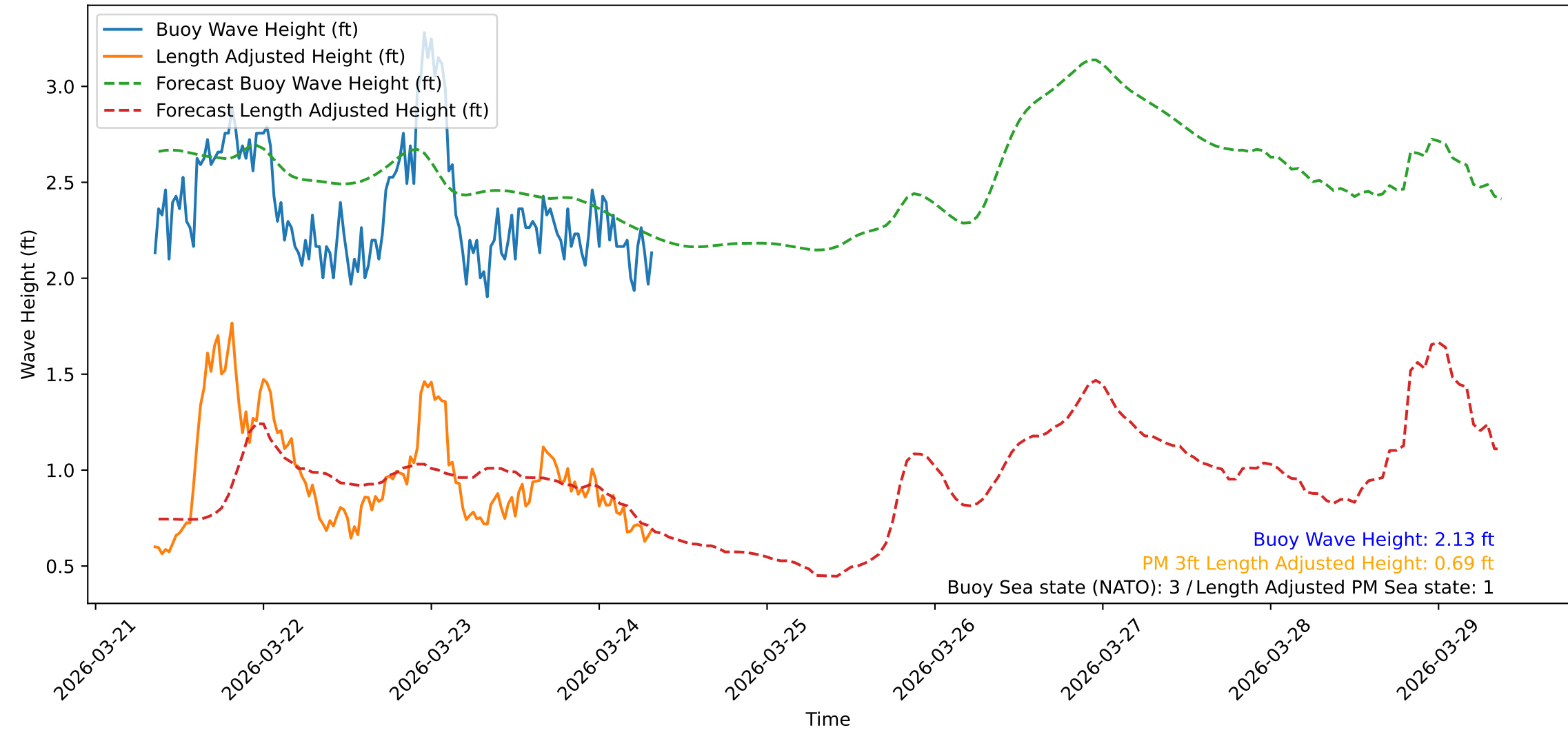
Wave Heights over Time for Green Beach at 2026-03-24 08:31:10
