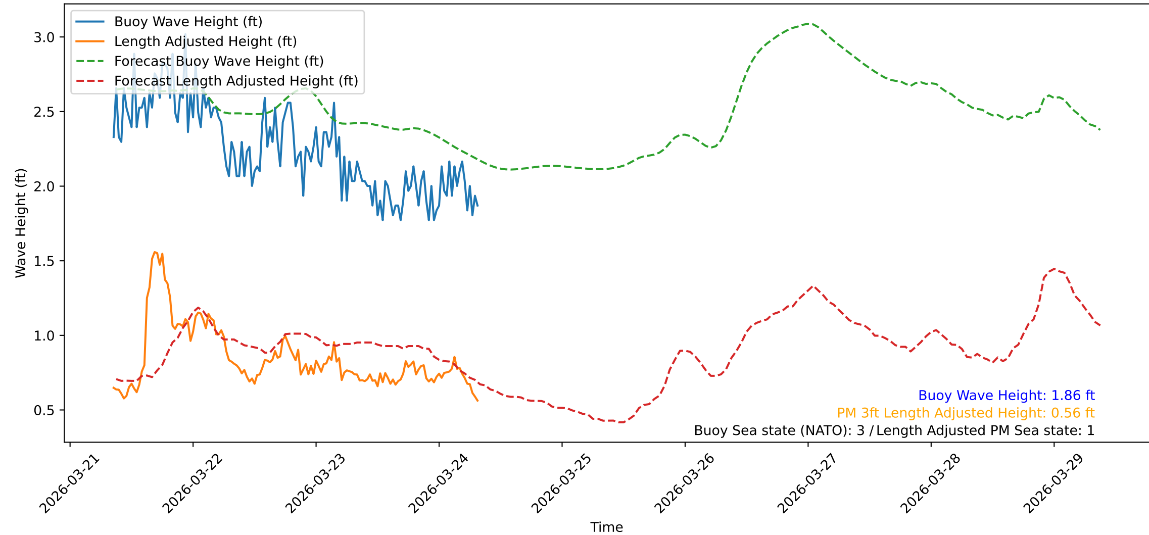
Wave Heights over Time for Oceanside Harbor at 2026-03-24 08:30:32
