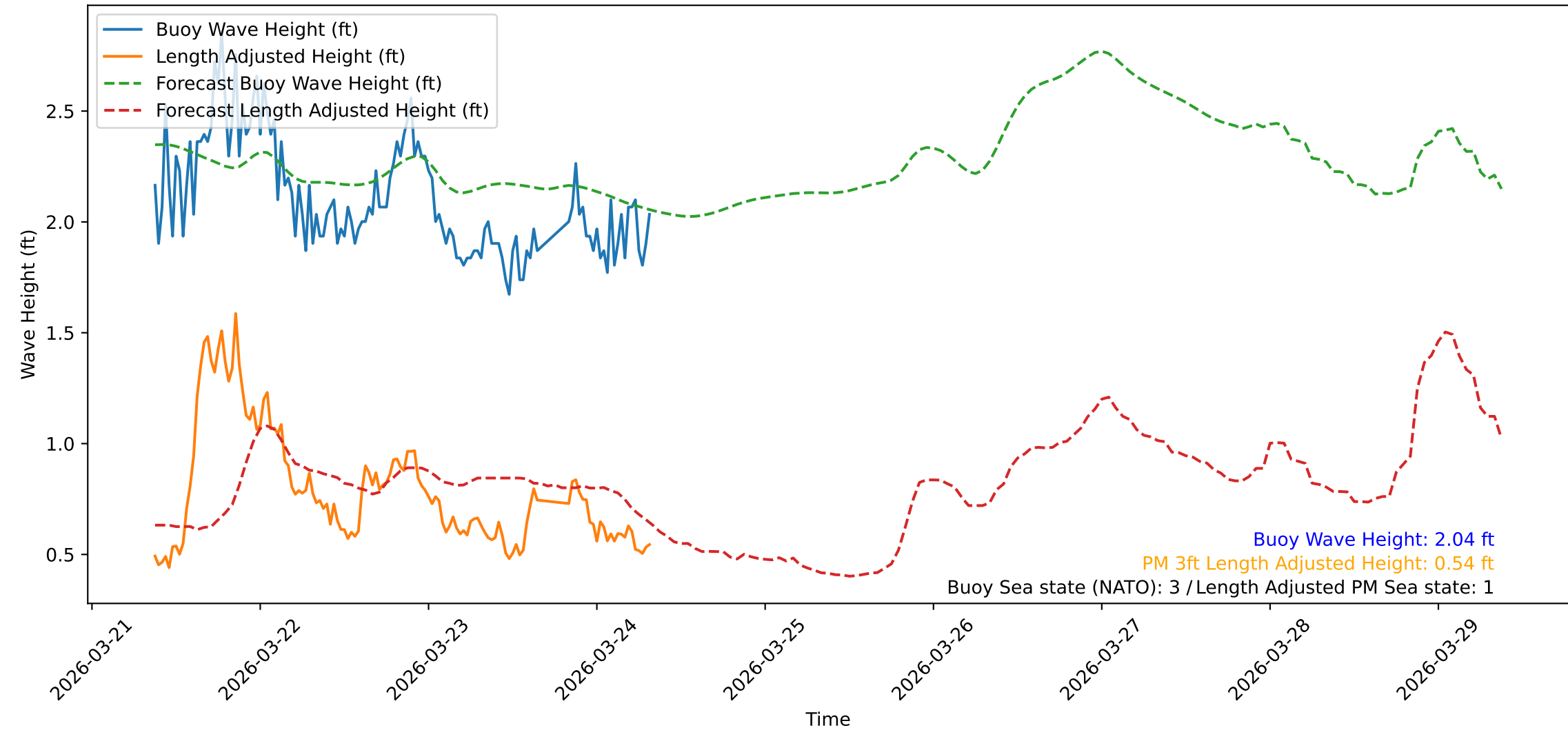
Wave Heights over Time for Red Beach at 2026-03-24 08:30:48
