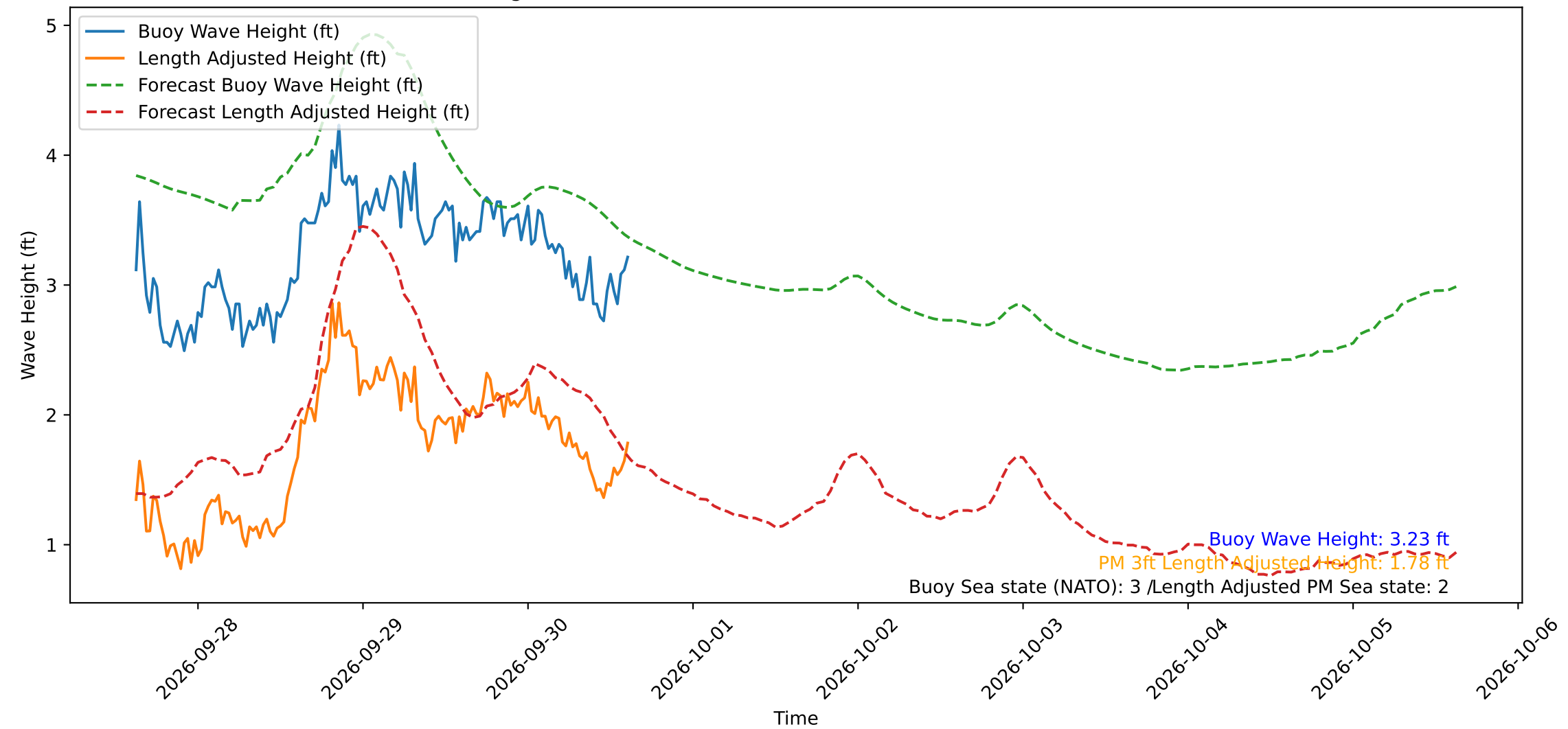
Wave Heights over Time for Oceanside Harbor at 2026-09-30 15:10:29
