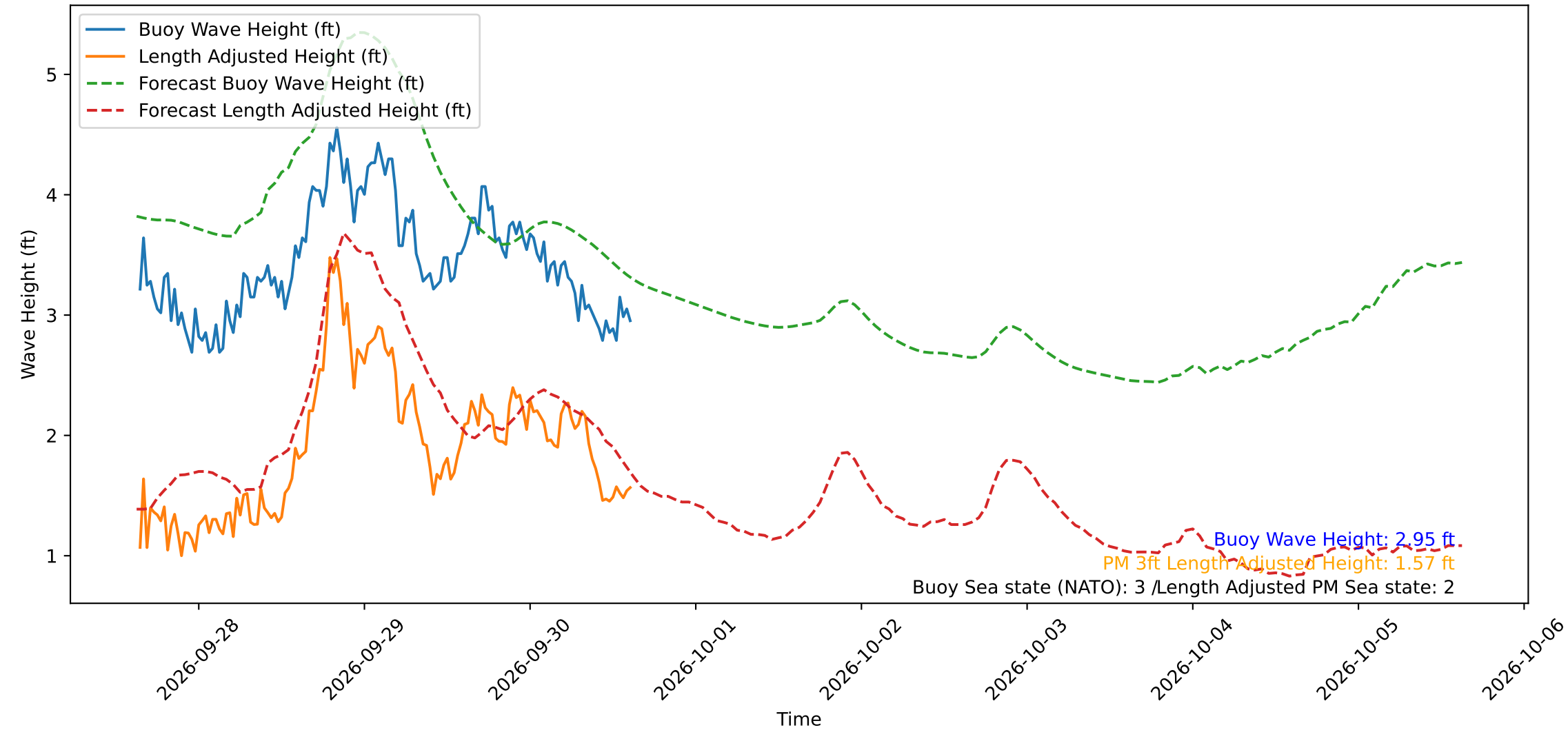
Wave Heights over Time for Green Beach at 2026-09-30 15:11:11
