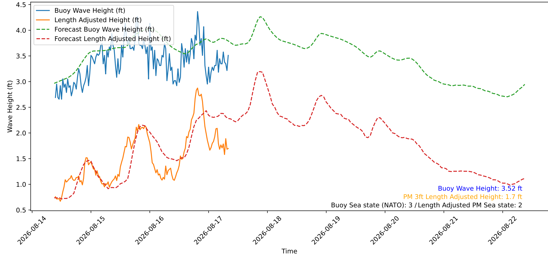
Wave Heights over Time for Green Beach at 2026-08-17 09:21:11
