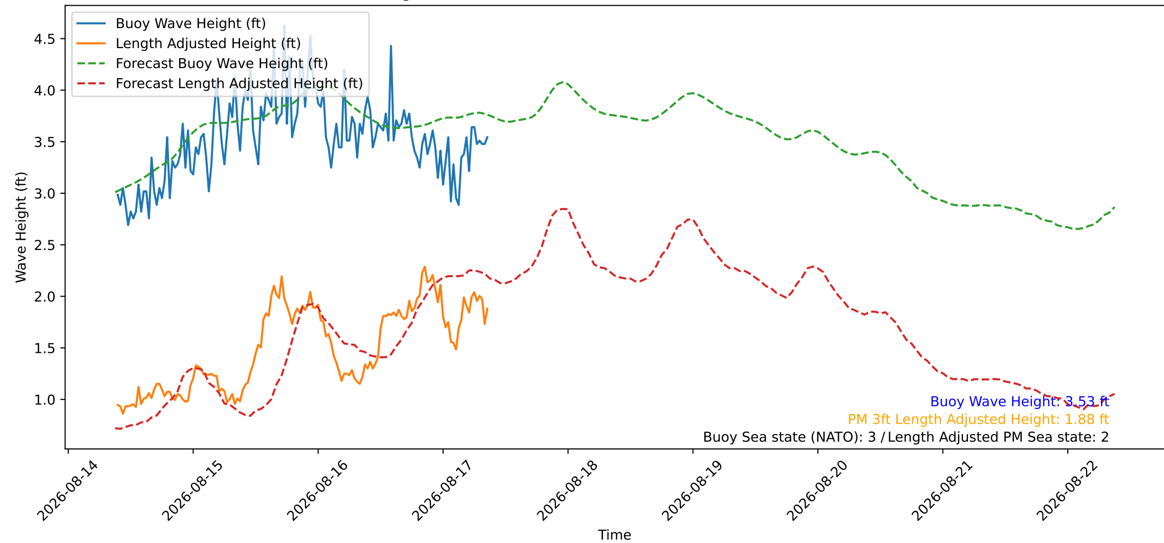
Wave Heights over Time for Oceanside Harbor at 2026-08-17 09:20:27
