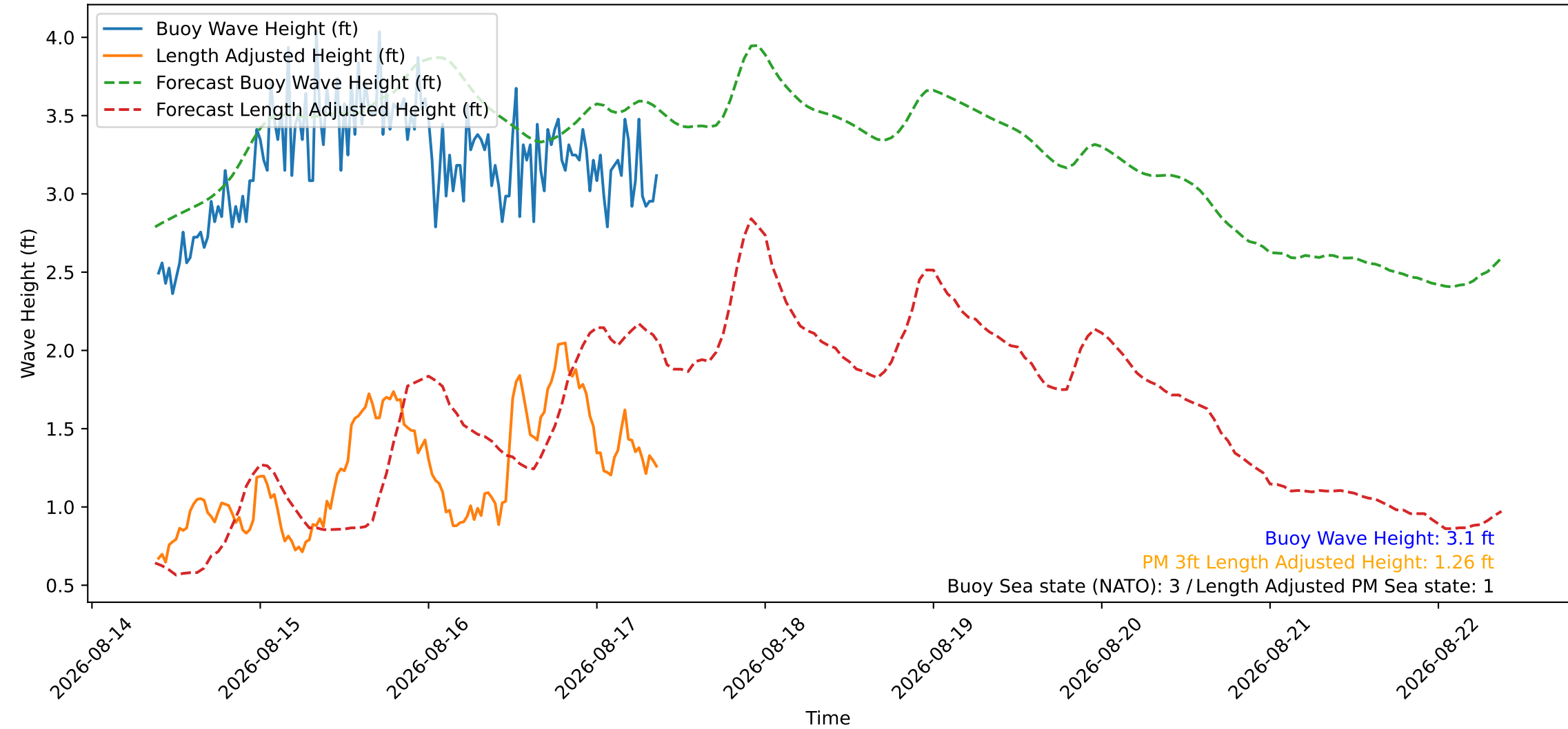
Wave Heights over Time for Red Beach at 2026-08-17 09:20:48
