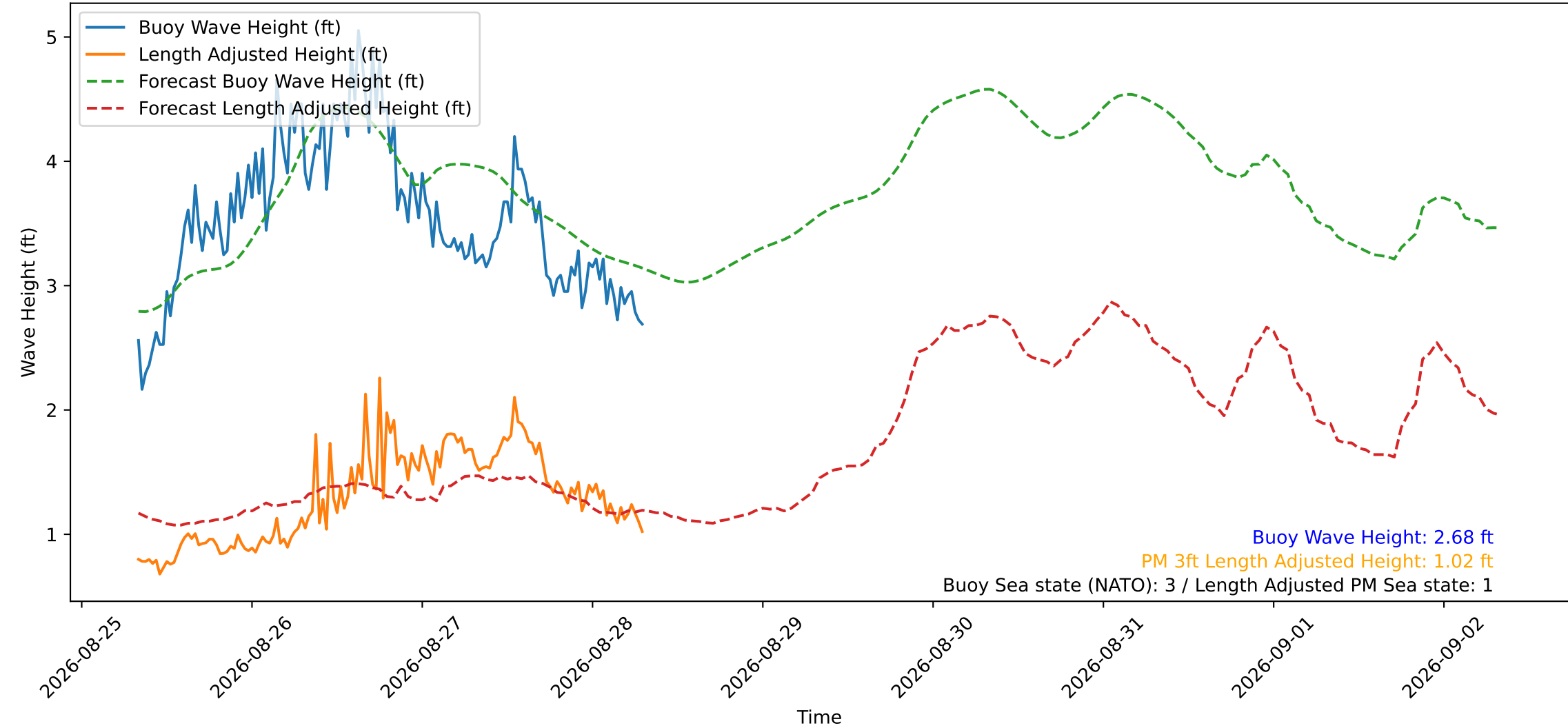
Wave Heights over Time for Red Beach at 2026-08-28 07:50:51
