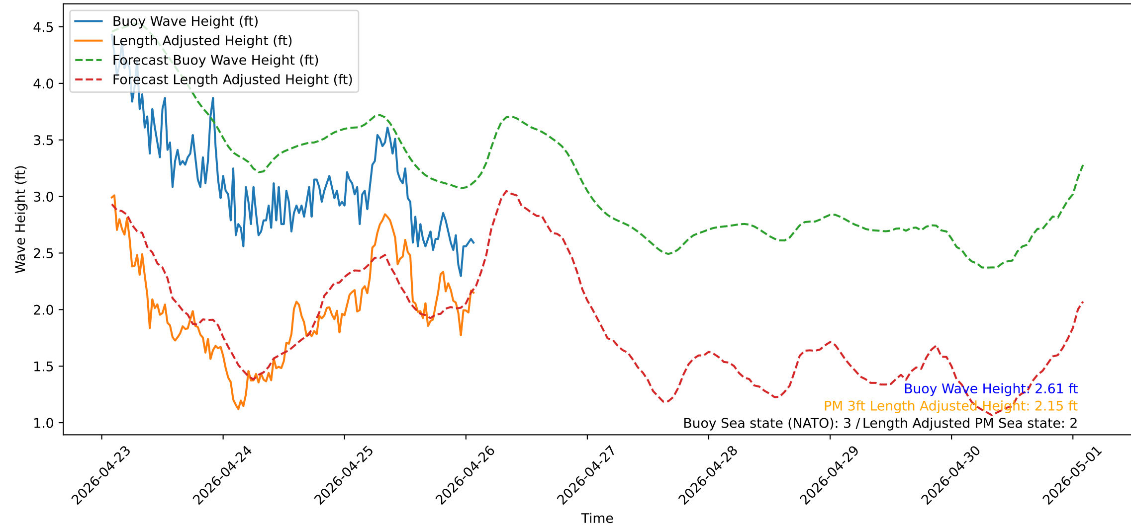
Wave Heights over Time for Oceanside Harbor at 2026-04-26 02:10:31
