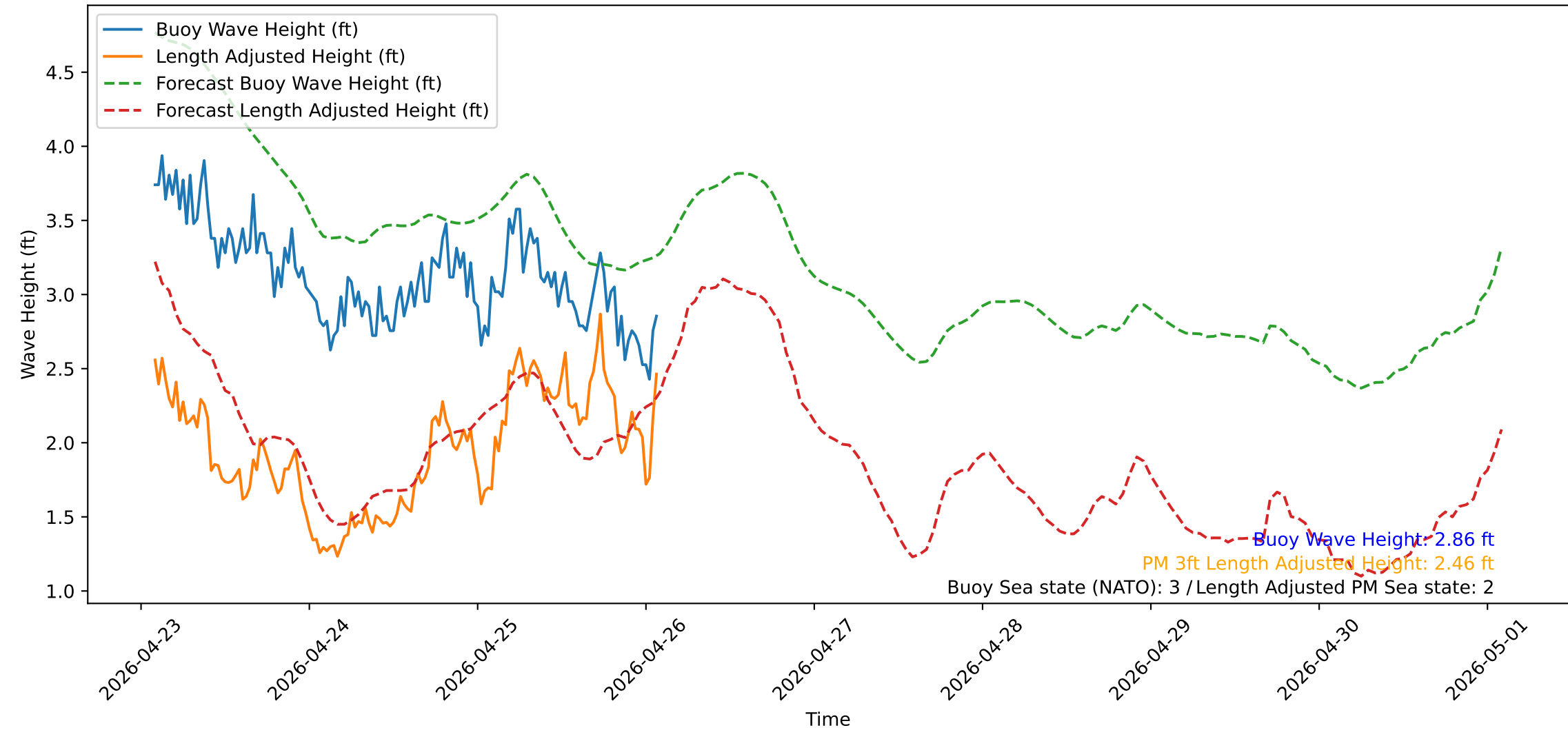
Wave Heights over Time for Green Beach at 2026-04-26 02:11:13
