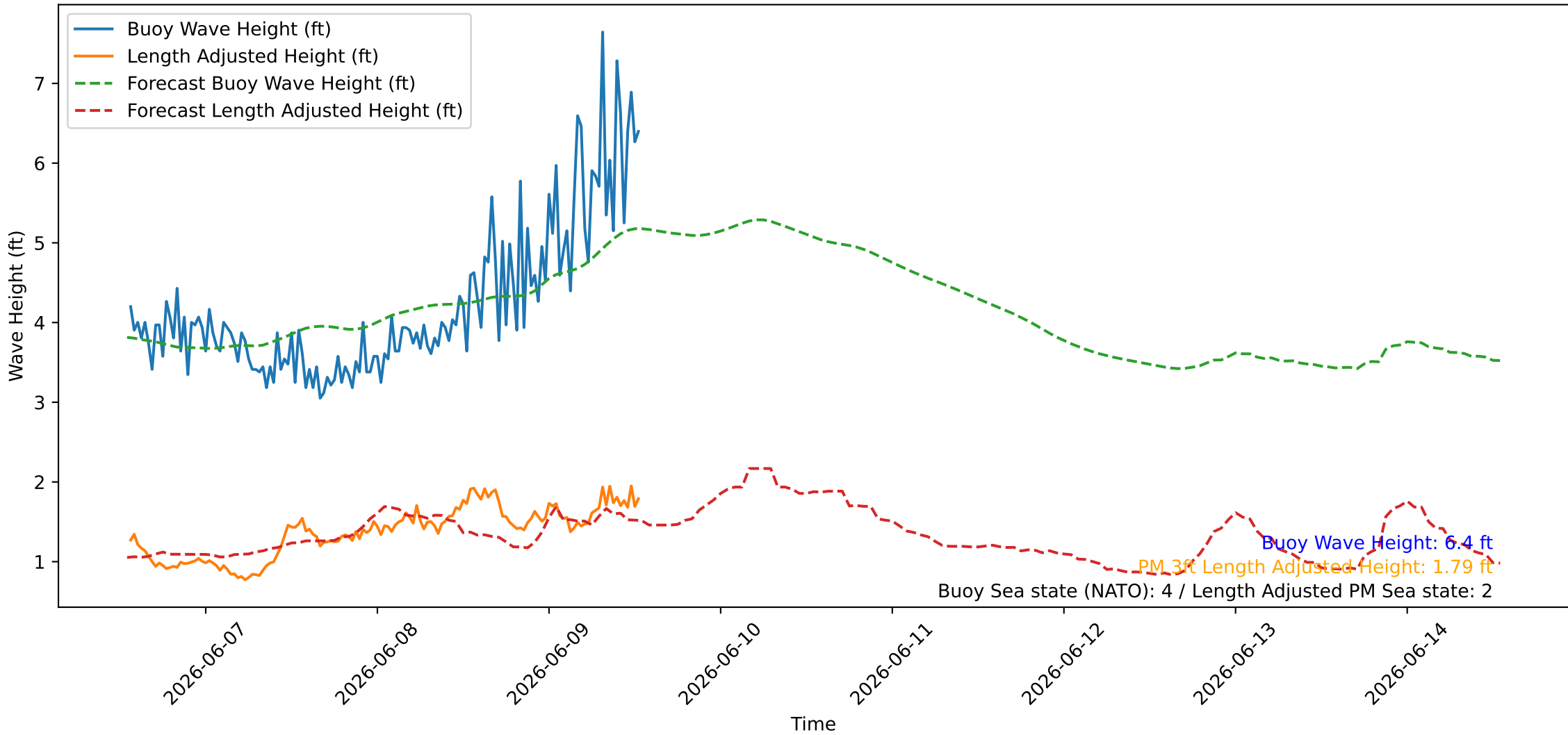
Wave Heights over Time for Red Beach at 2026-06-09 13:10:45
