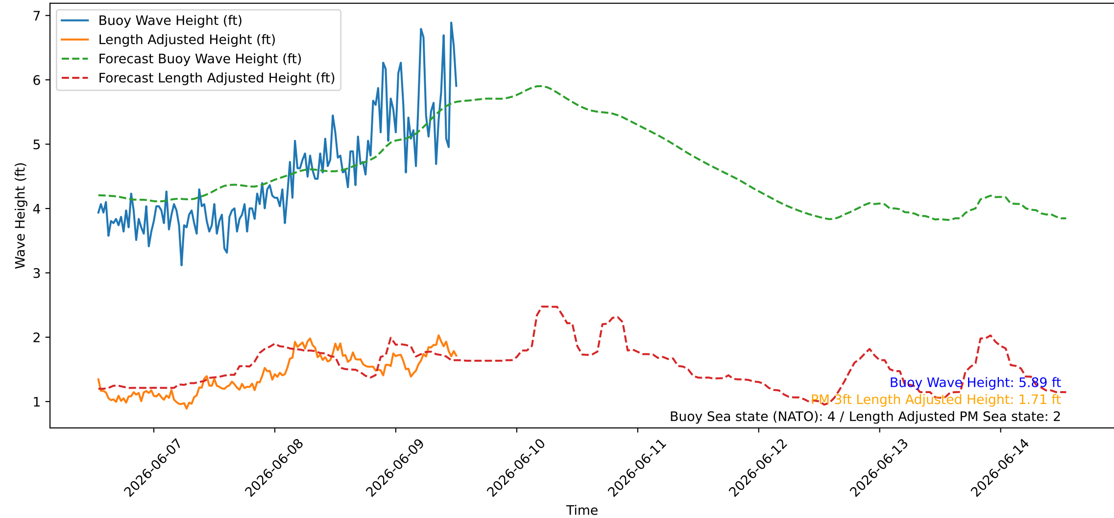
Wave Heights over Time for Green Beach at 2026-06-09 13:11:07
