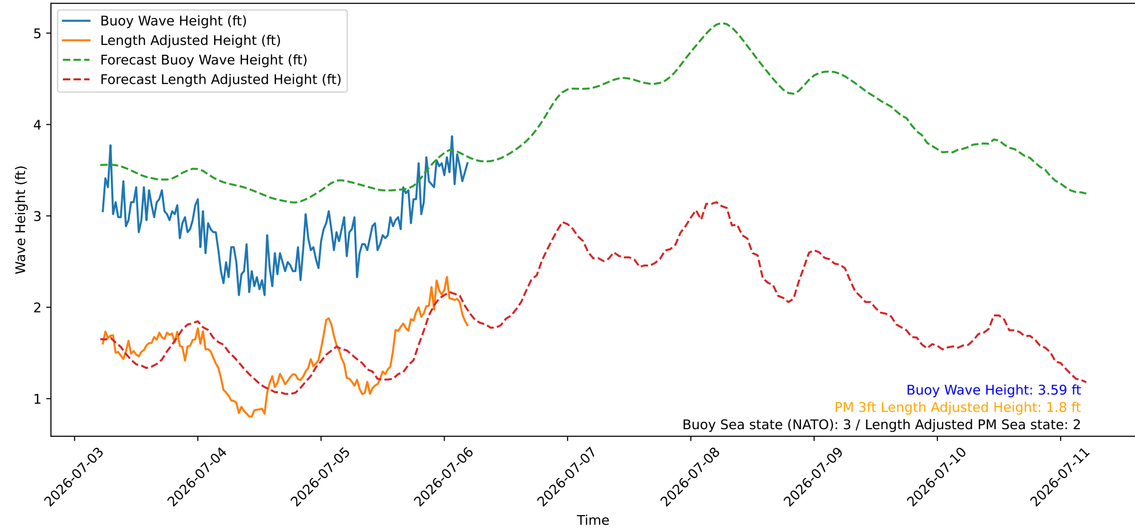
Wave Heights over Time for Oceanside Harbor at 2026-07-06 05:20:26
