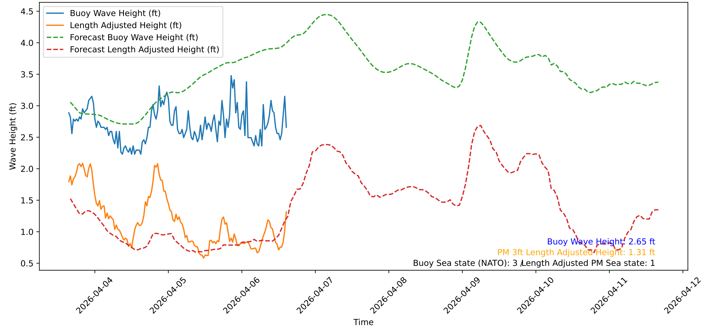
Wave Heights over Time for Green Beach at 2026-04-06 15:31:10
