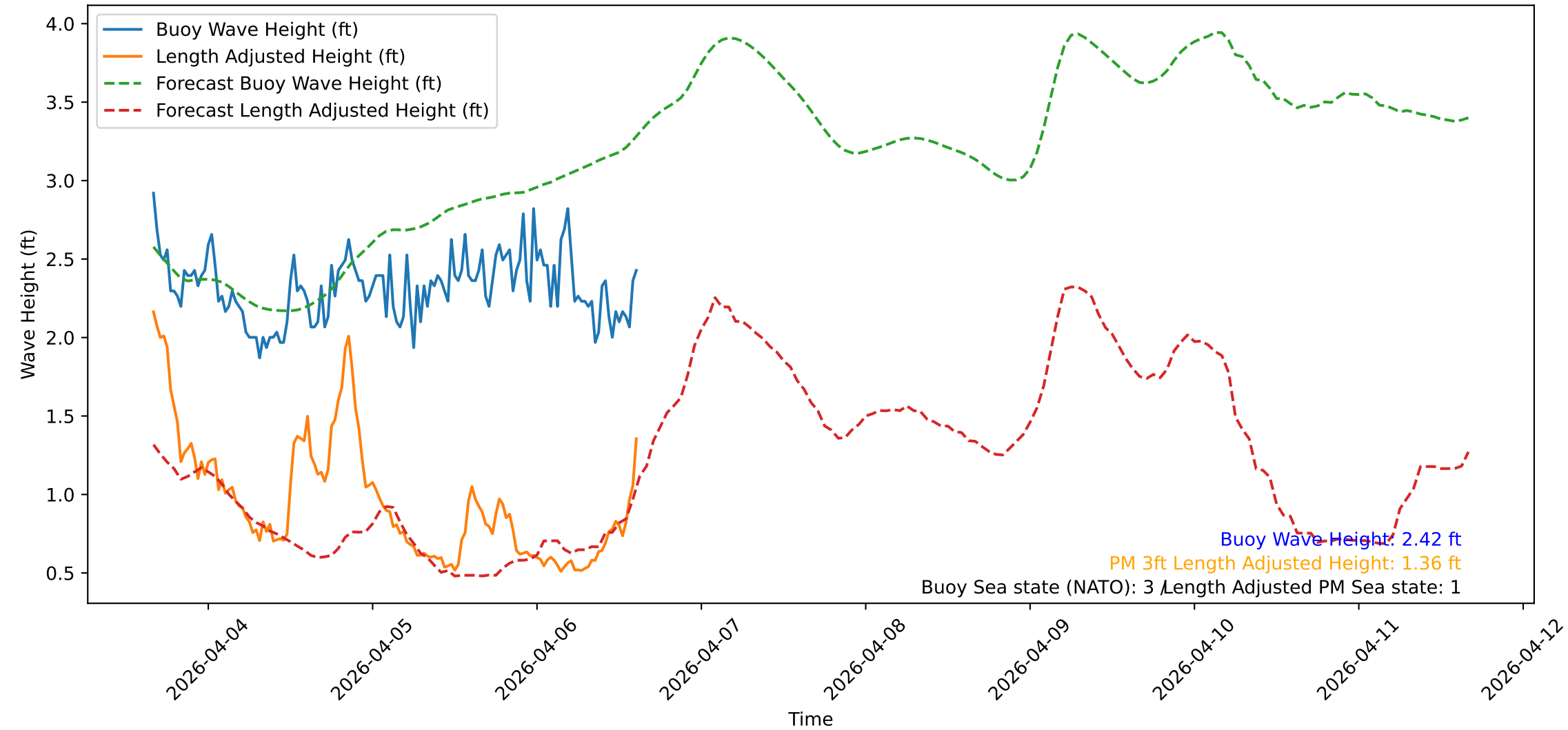
Wave Heights over Time for Red Beach at 2026-04-06 15:30:47
