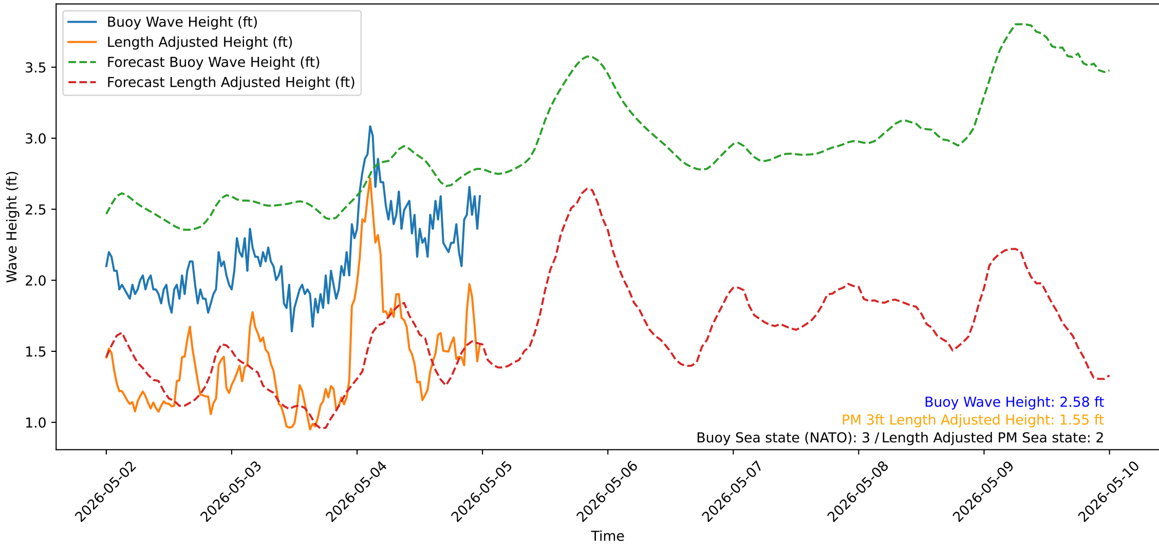
Wave Heights over Time for Oceanside Harbor at 2026-05-05 00:00:31
