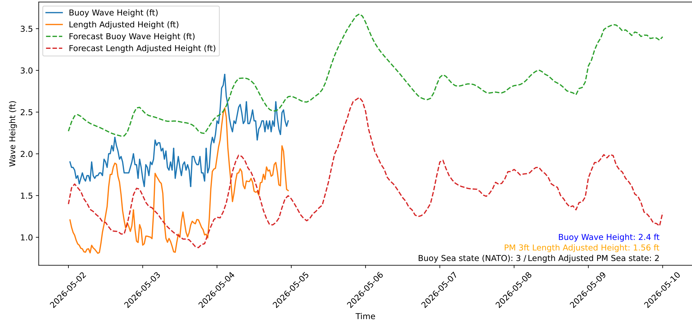
Wave Heights over Time for Red Beach at 2026-05-05 00:00:50
