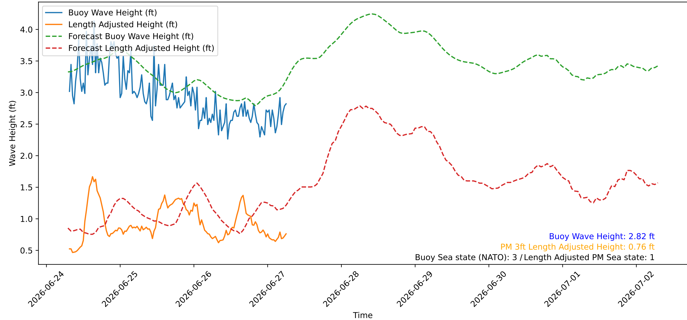
Wave Heights over Time for Red Beach at 2026-06-27 07:00:45
