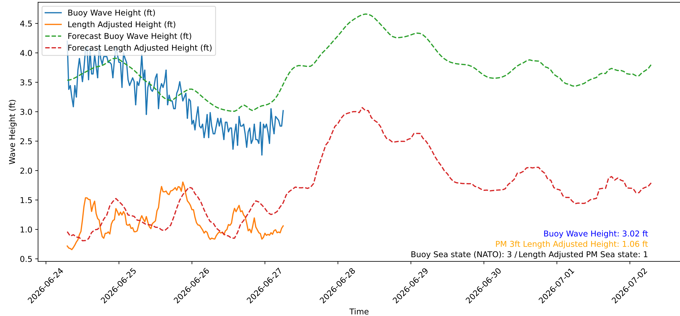
Wave Heights over Time for Green Beach at 2026-06-27 07:01:08
