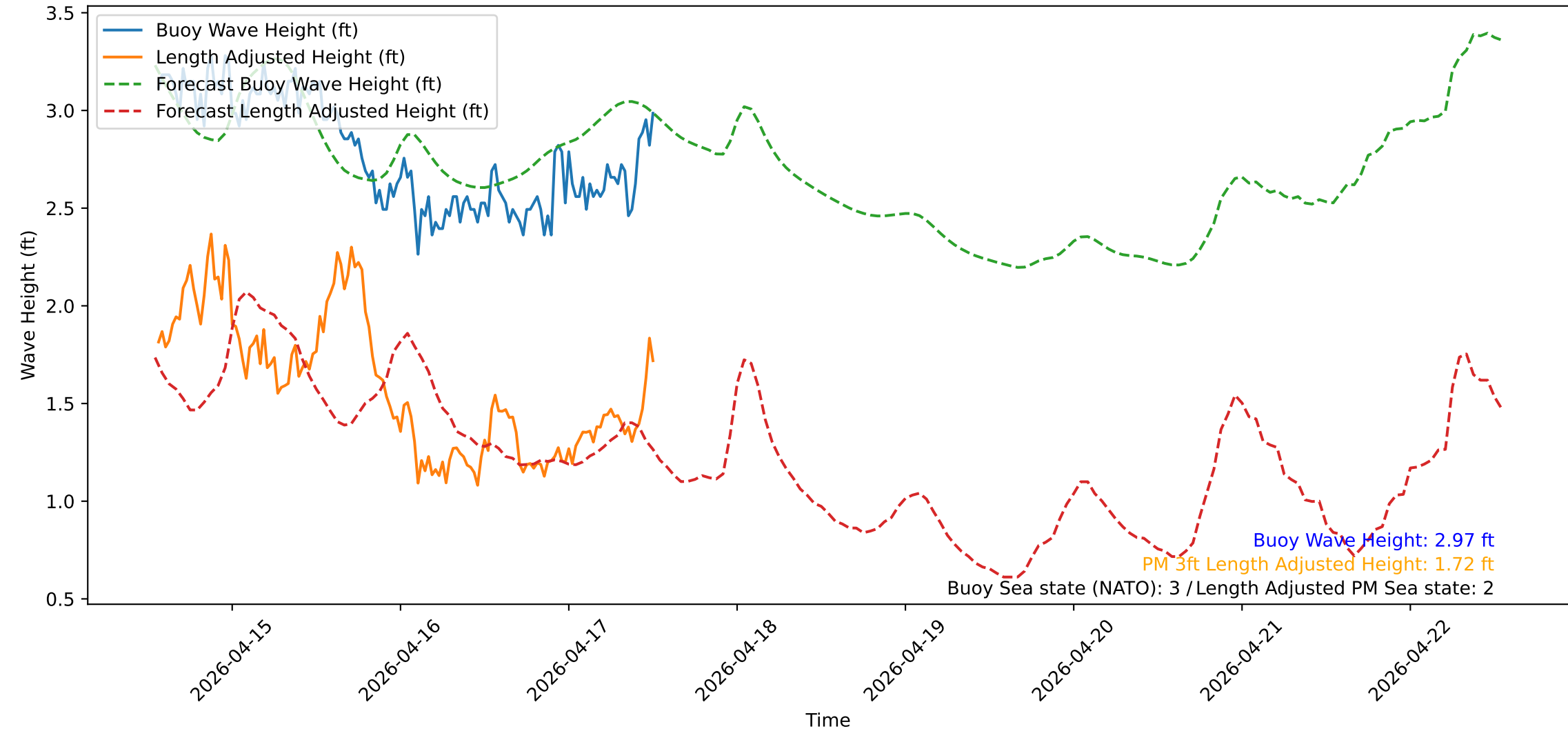
Wave Heights over Time for Red Beach at 2026-04-17 13:00:51
