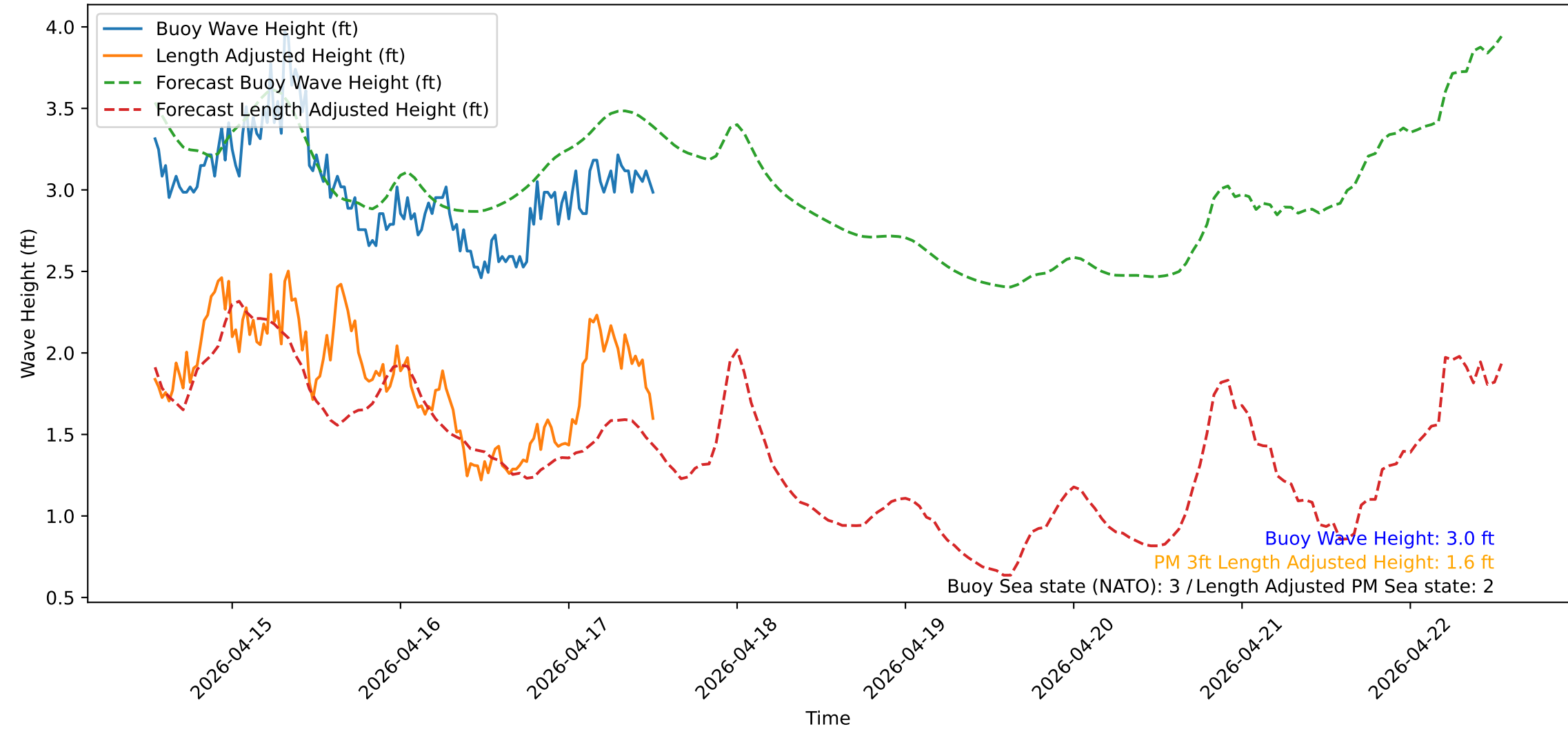
Wave Heights over Time for Green Beach at 2026-04-17 13:01:13
