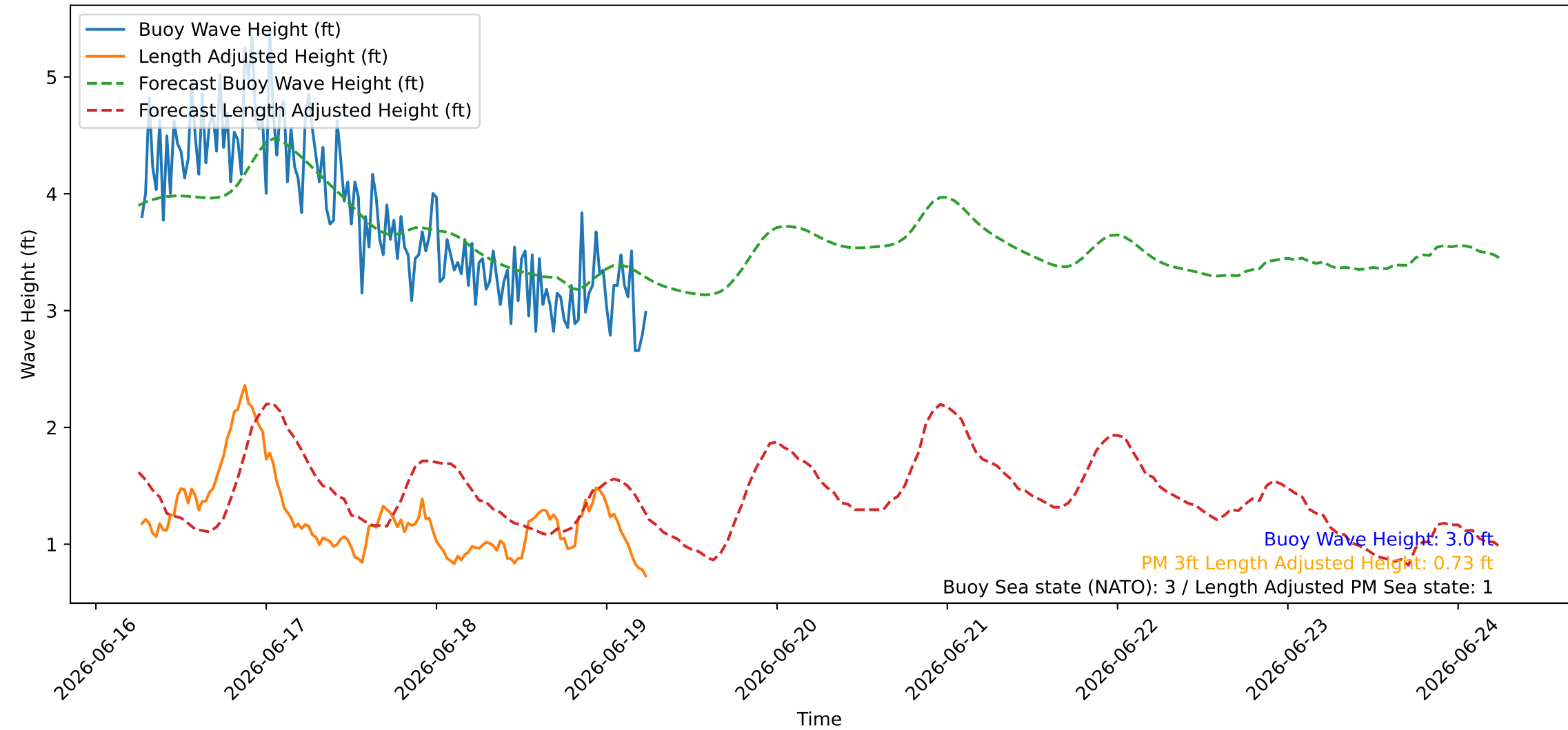
Wave Heights over Time for Red Beach at 2026-06-19 06:20:46
