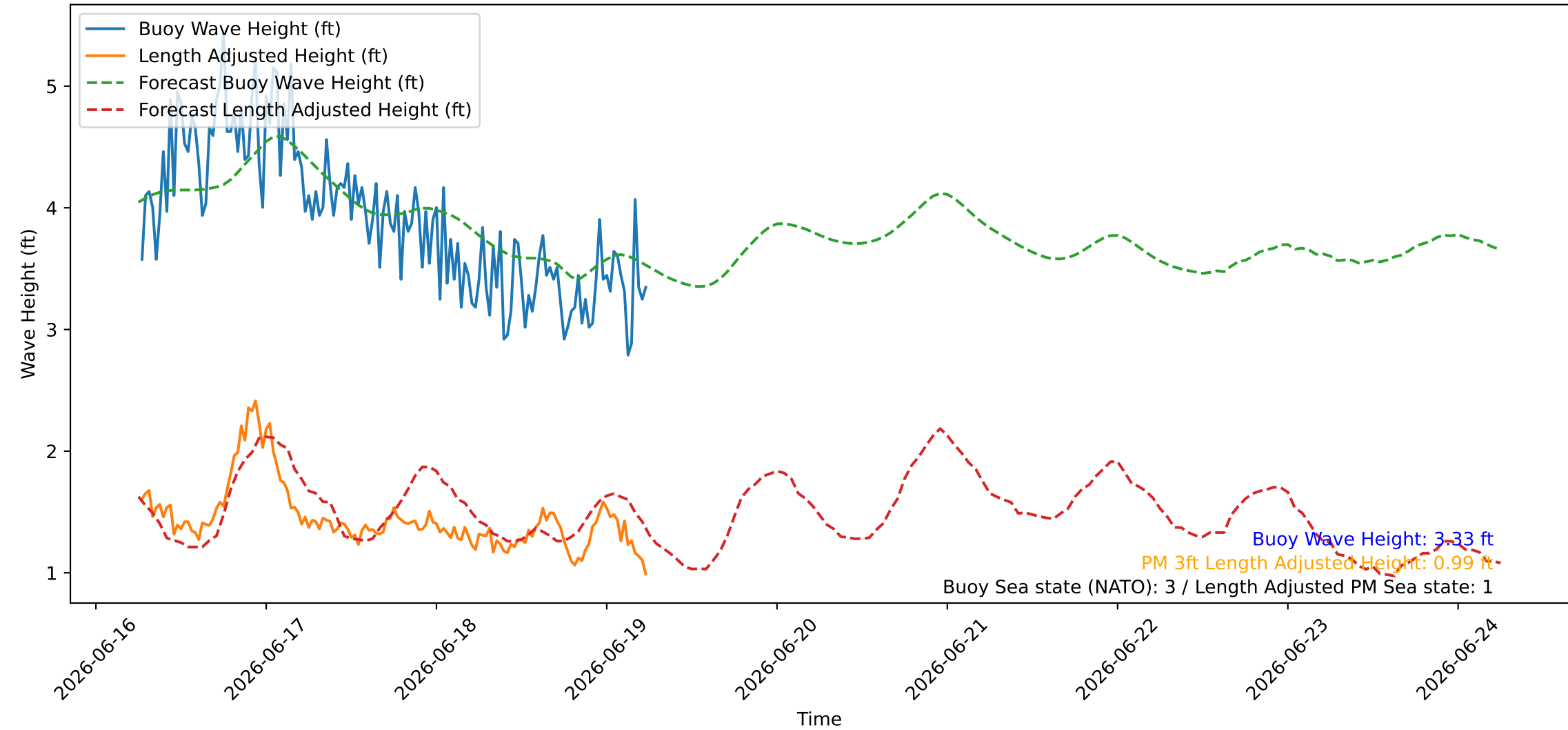
Wave Heights over Time for Oceanside Harbor at 2026-06-19 06:20:26
