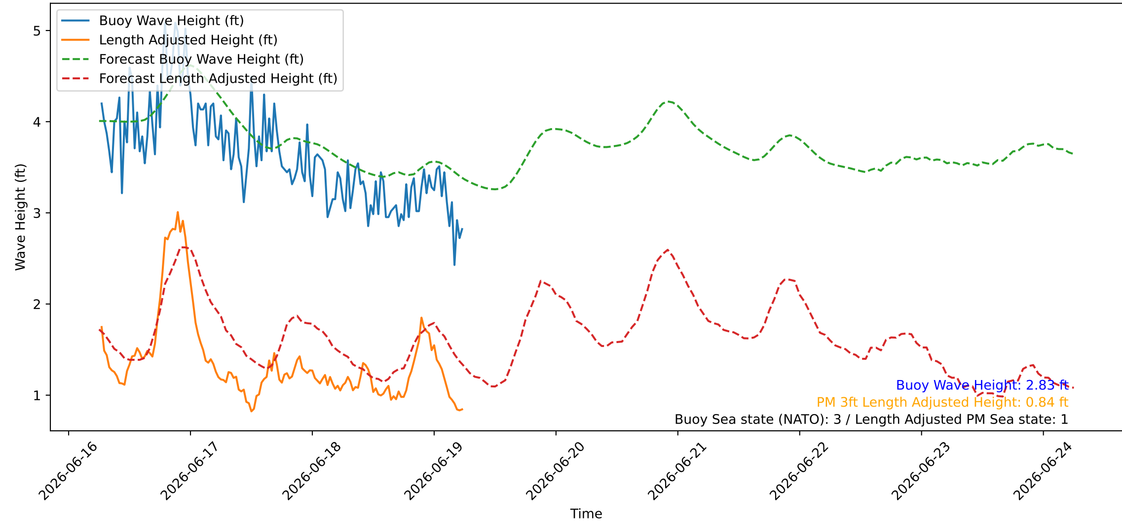
Wave Heights over Time for Green Beach at 2026-06-19 06:21:09
