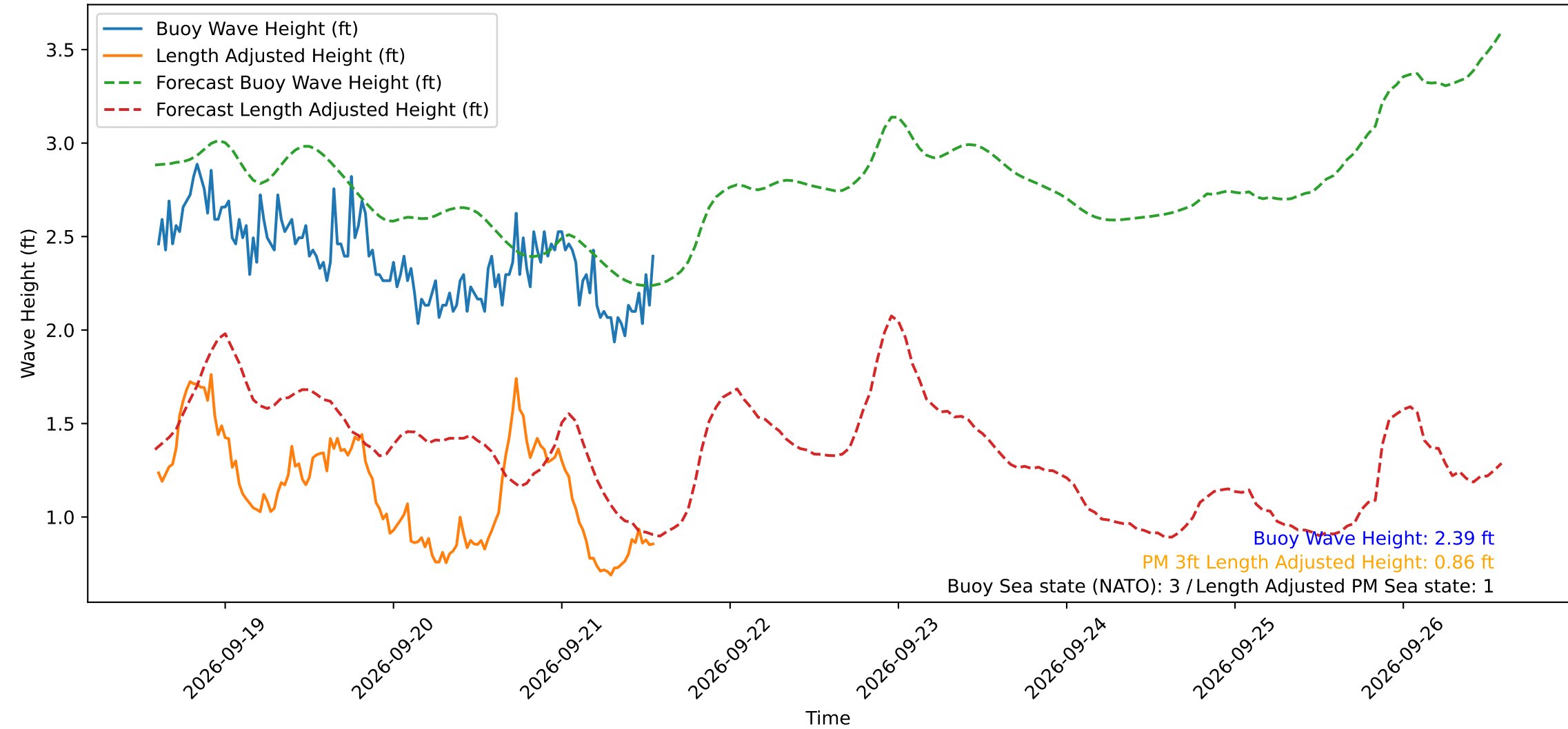
Wave Heights over Time for Red Beach at 2026-09-21 14:00:49
