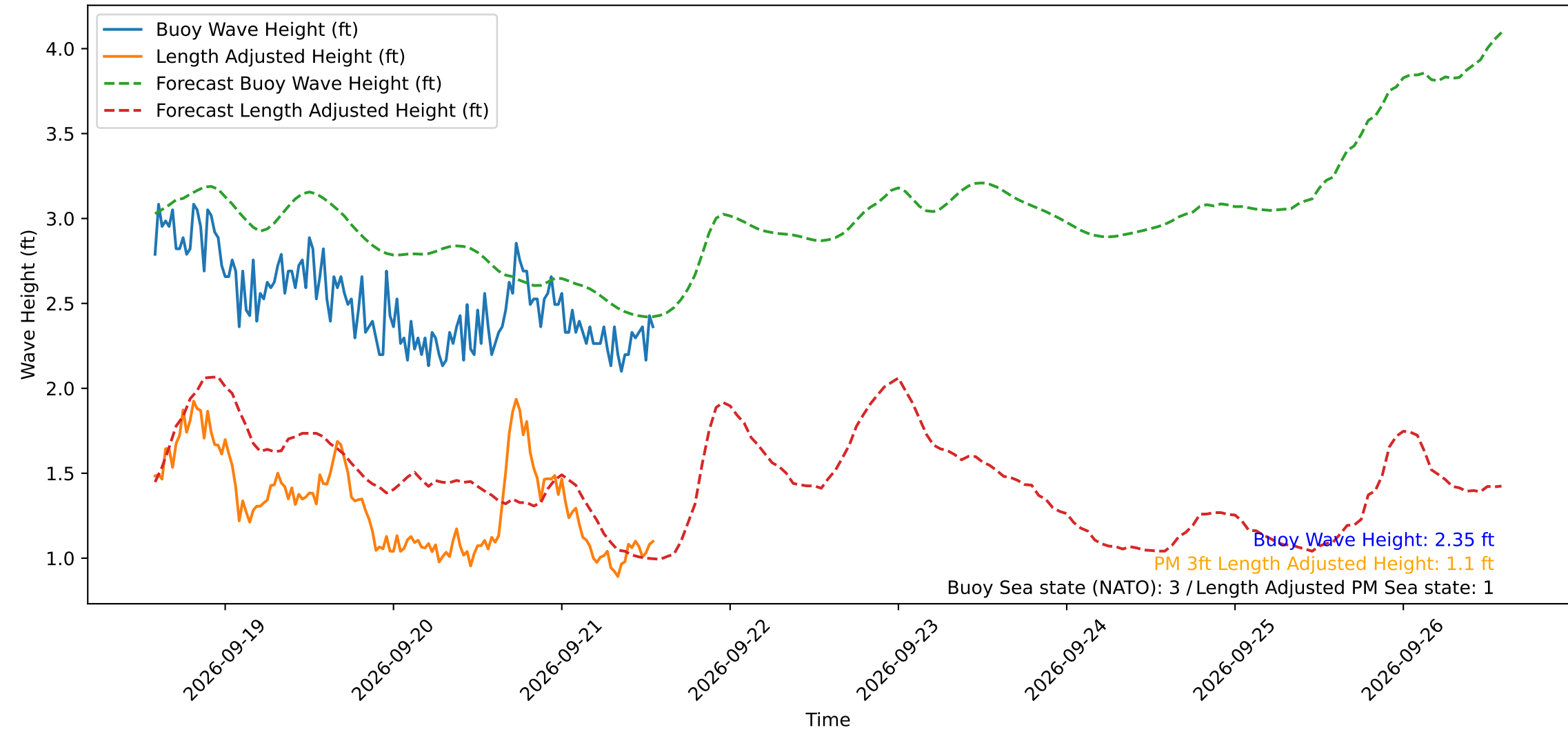
Wave Heights over Time for Oceanside Harbor at 2026-09-21 14:00:30
