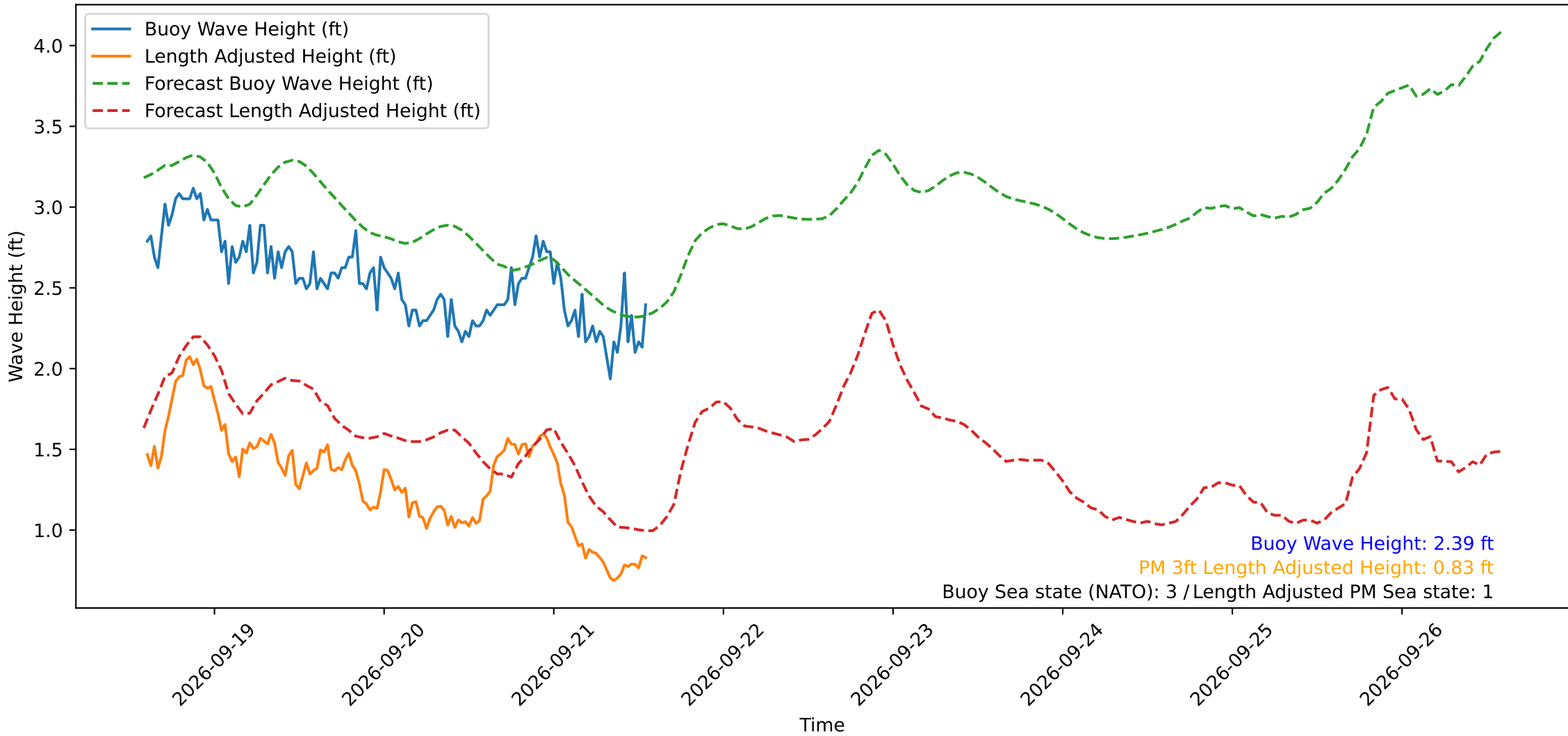
Wave Heights over Time for Green Beach at 2026-09-21 14:01:11
