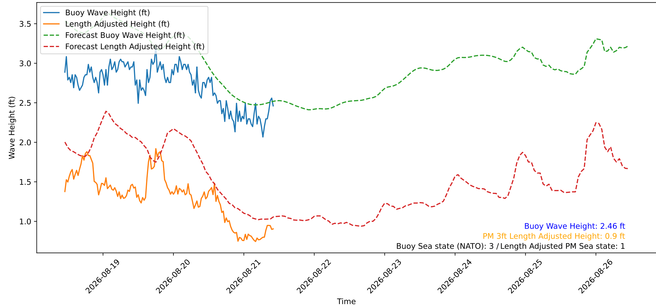
Wave Heights over Time for Red Beach at 2026-08-21 10:40:47
