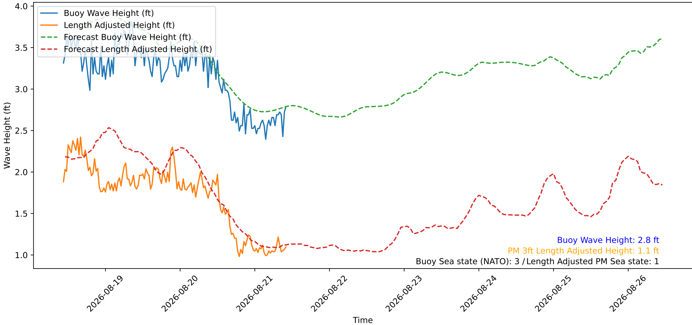
Wave Heights over Time for Oceanside Harbor at 2026-08-21 10:40:27
