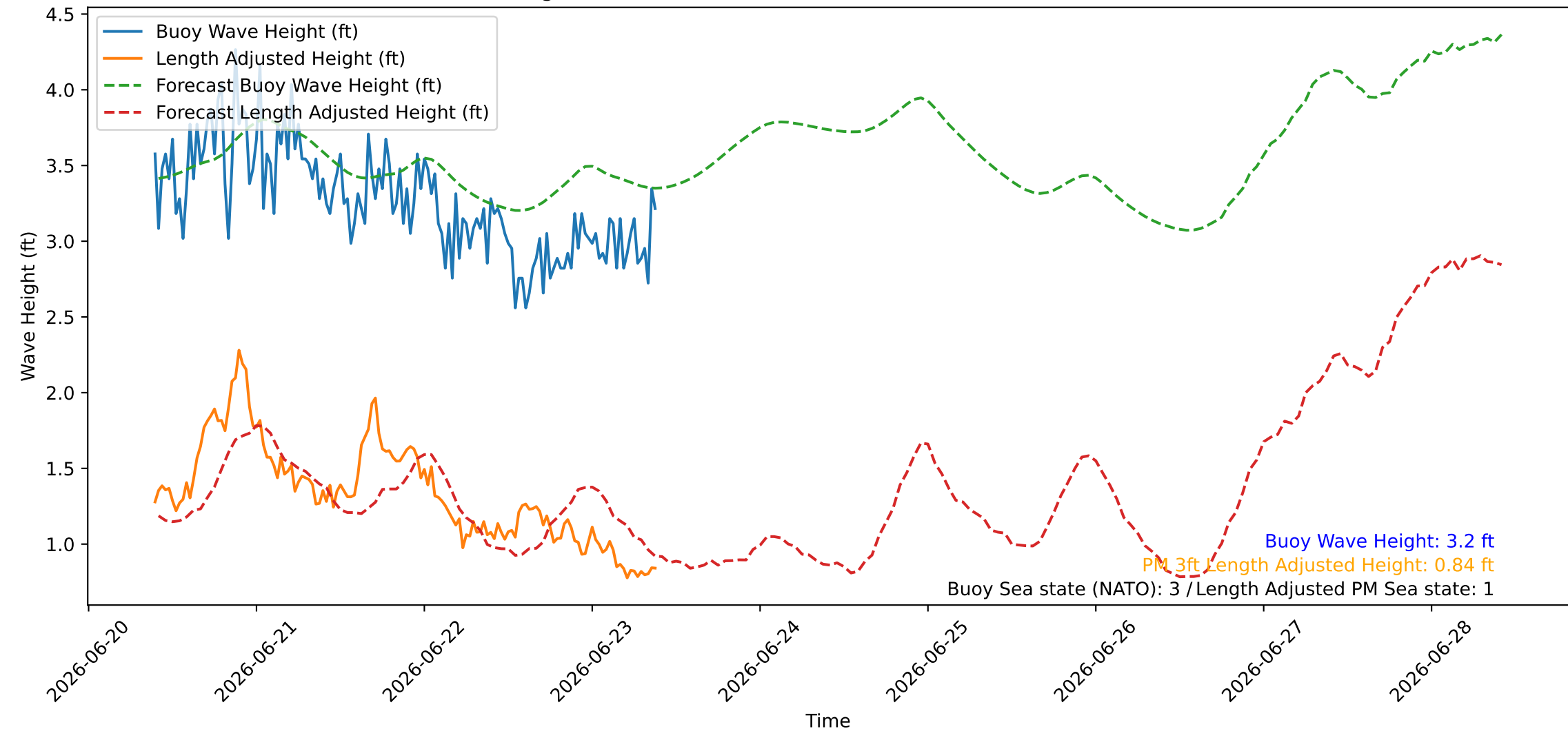
Wave Heights over Time for Oceanside Harbor at 2026-06-23 09:30:26
