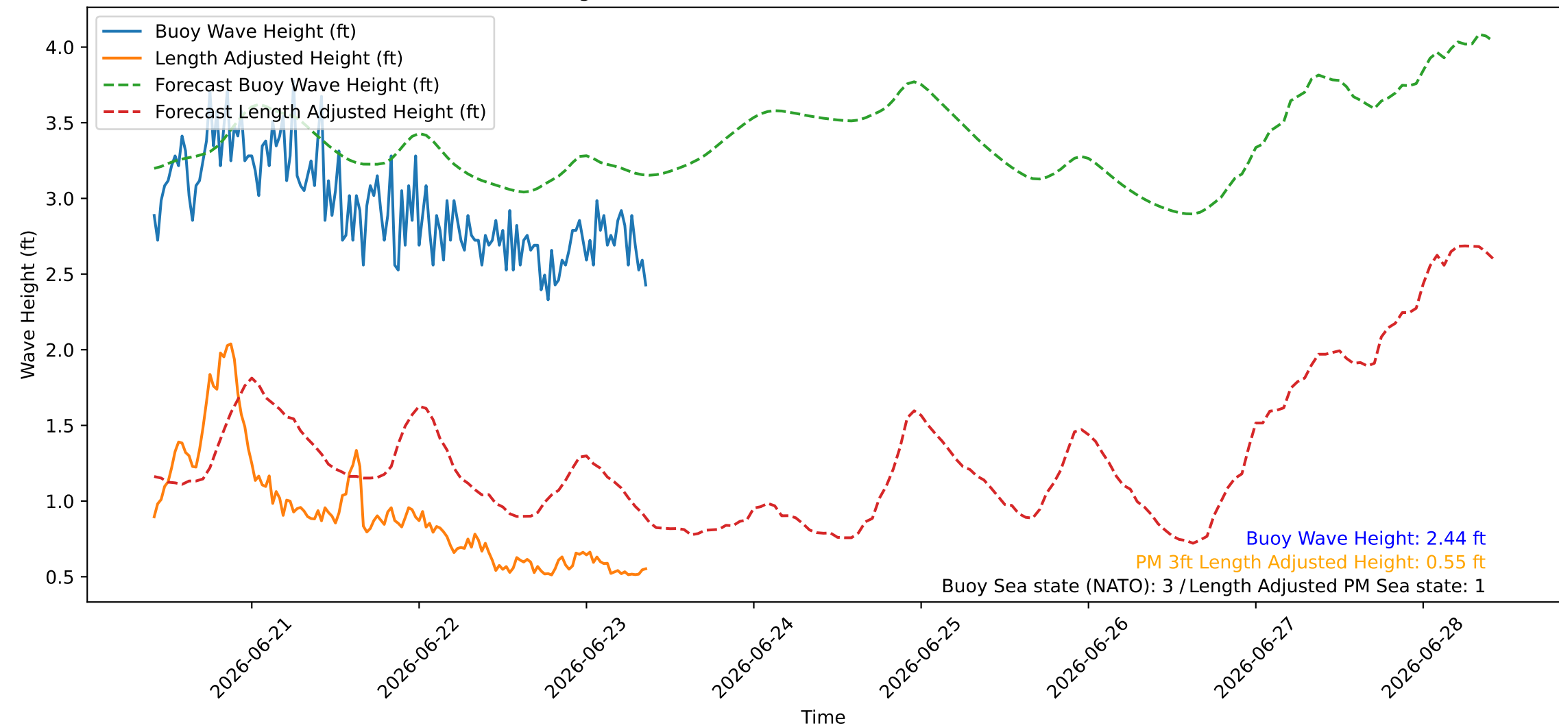
Wave Heights over Time for Red Beach at 2026-06-23 09:30:45
