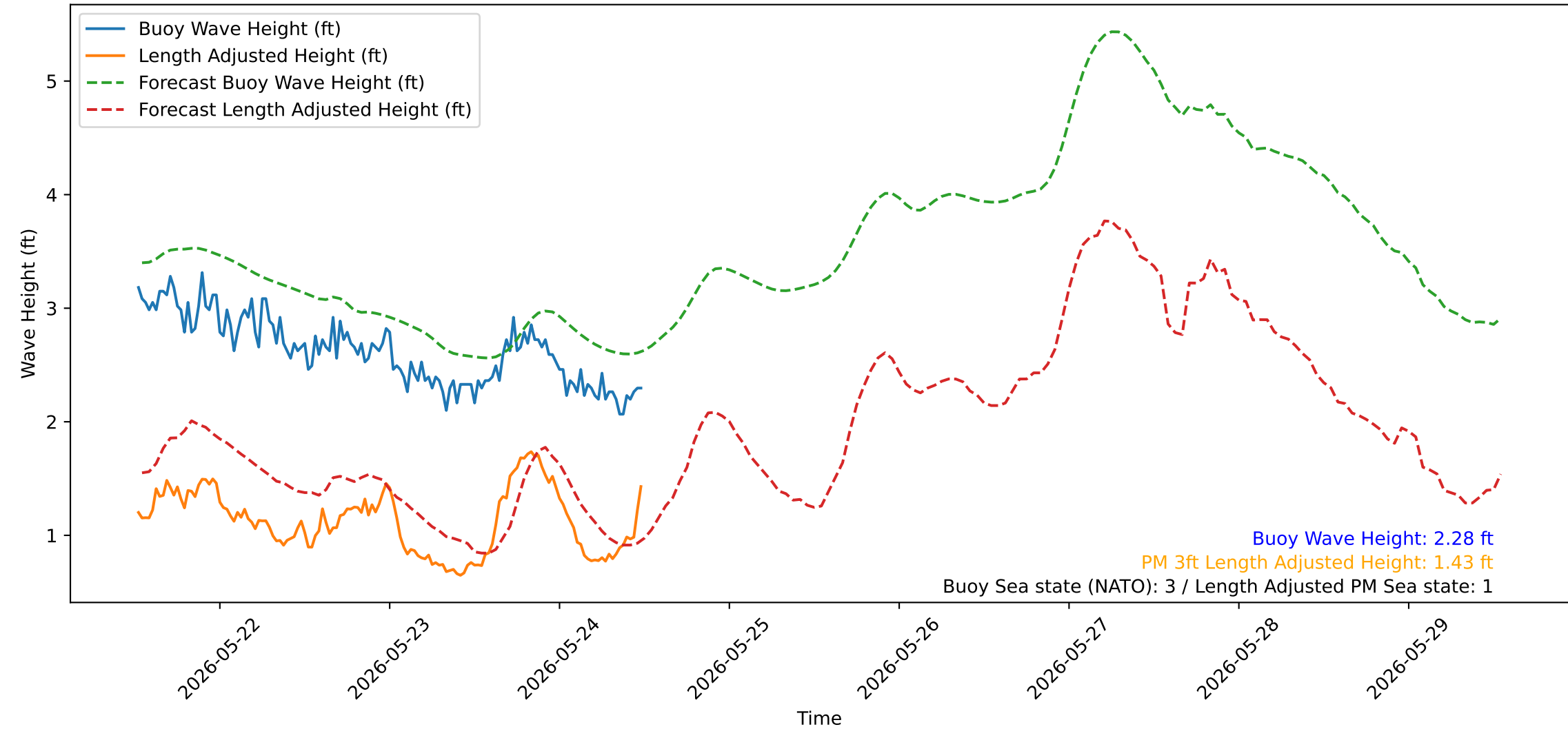
Wave Heights over Time for Green Beach at 2026-05-24 12:31:14
