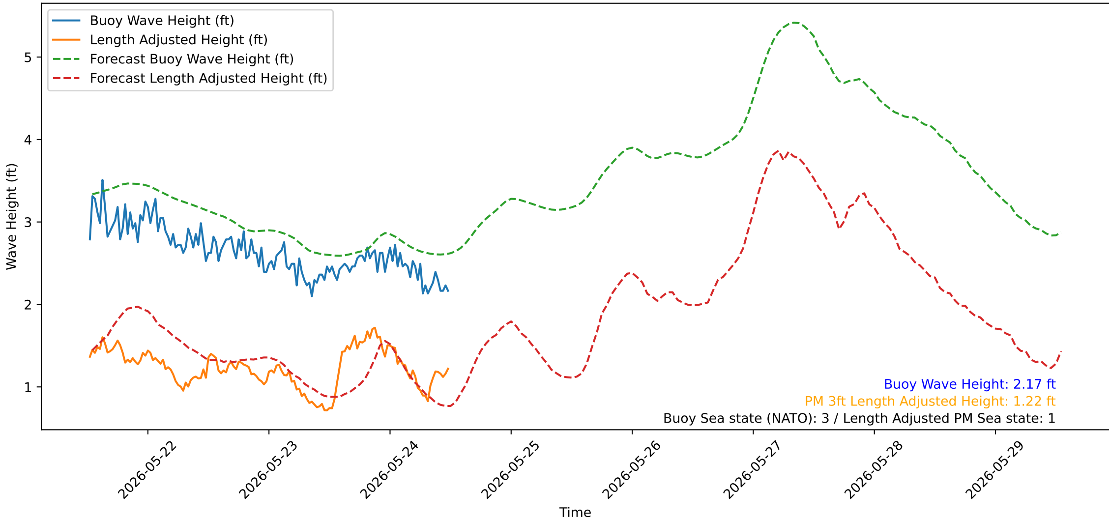
Wave Heights over Time for Oceanside Harbor at 2026-05-24 12:30:32
