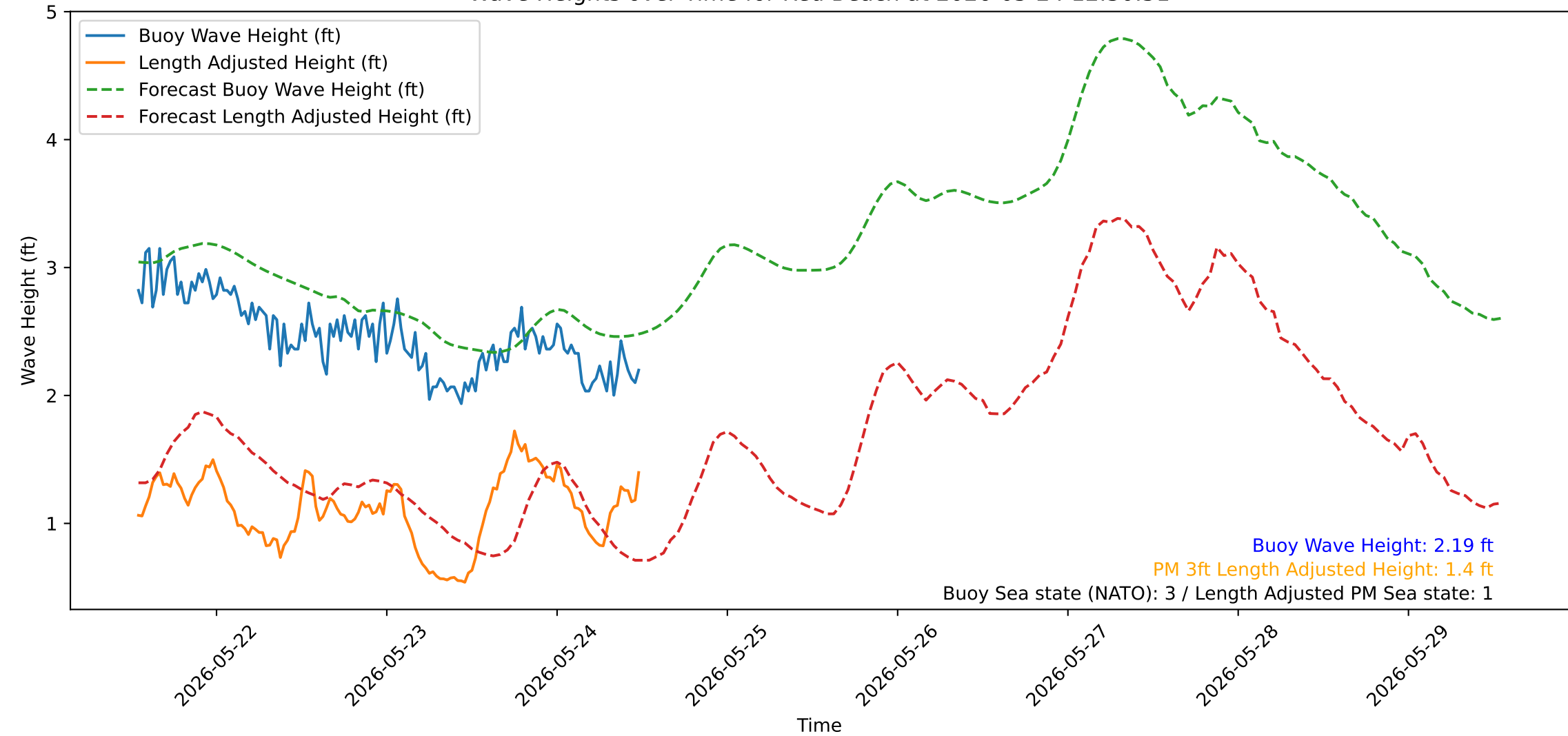
Wave Heights over Time for Red Beach at 2026-05-24 12:30:51
