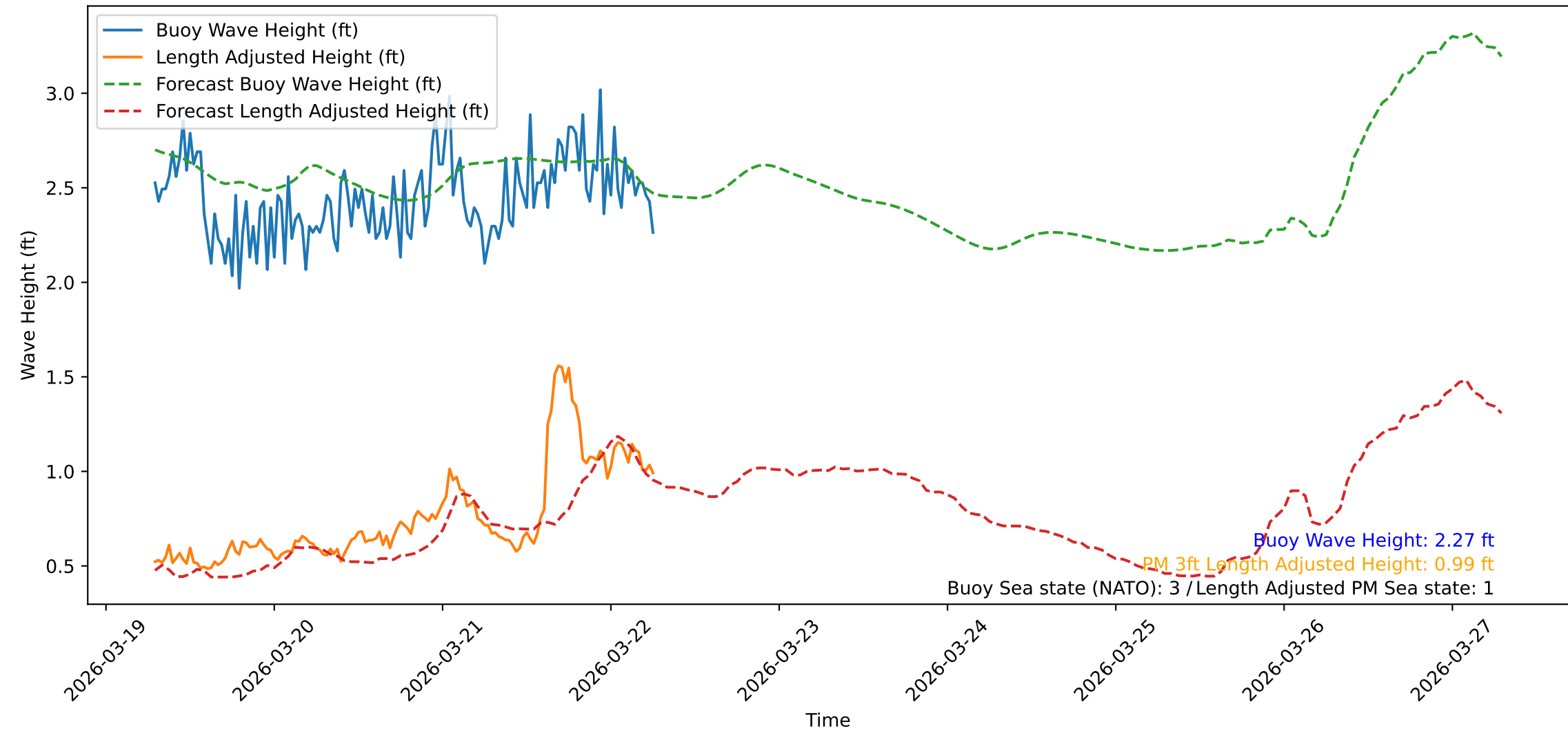
Wave Heights over Time for Oceanside Harbor at 2026-03-22 07:00:31
