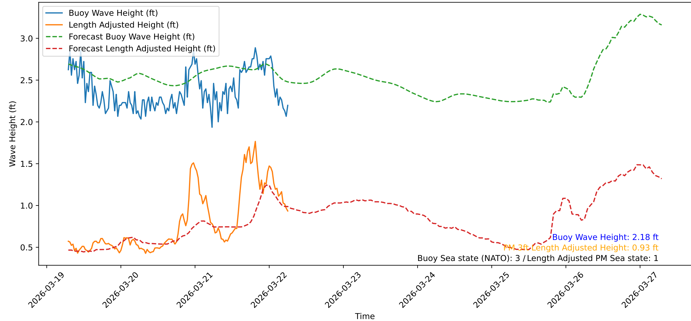
Wave Heights over Time for Green Beach at 2026-03-22 07:01:09
