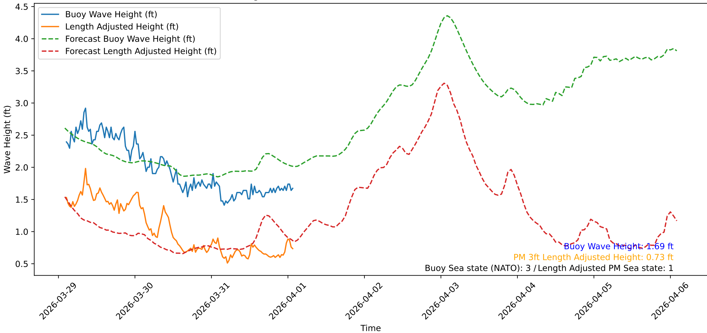
Wave Heights over Time for Green Beach at 2026-04-01 02:21:09
