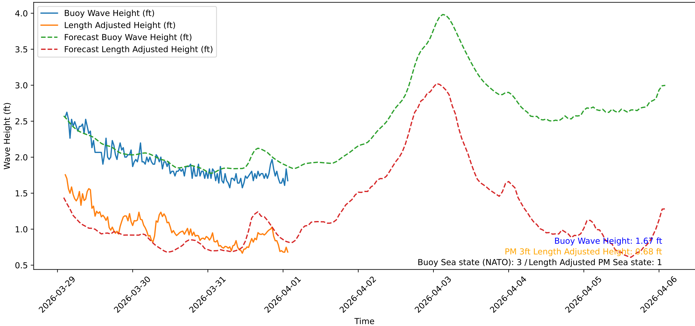
Wave Heights over Time for Oceanside Harbor at 2026-04-01 02:20:31
