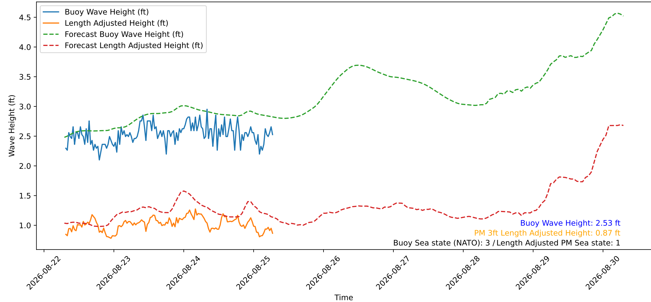
Wave Heights over Time for Red Beach at 2026-08-25 07:20:50
