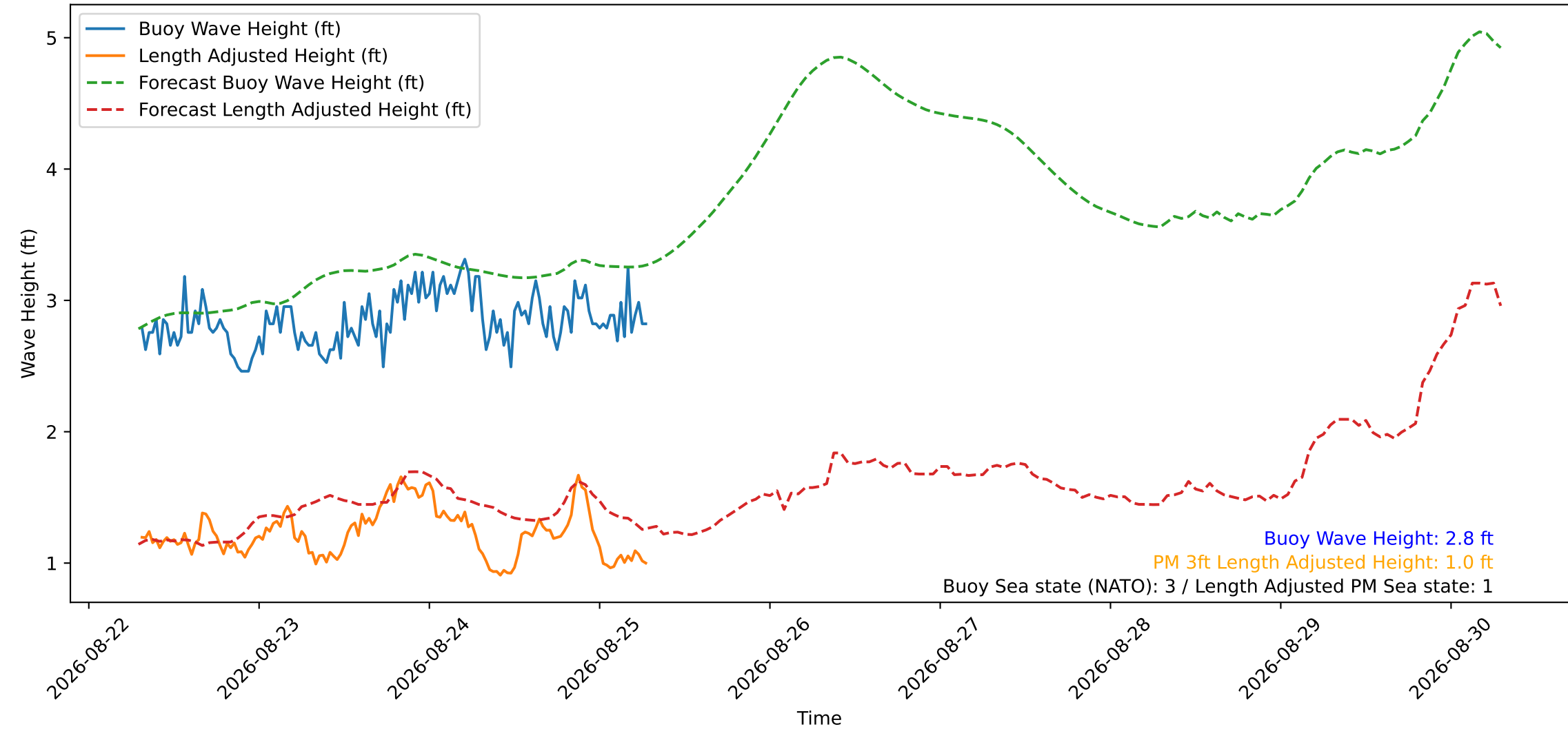
Wave Heights over Time for Green Beach at 2026-08-25 07:21:14
