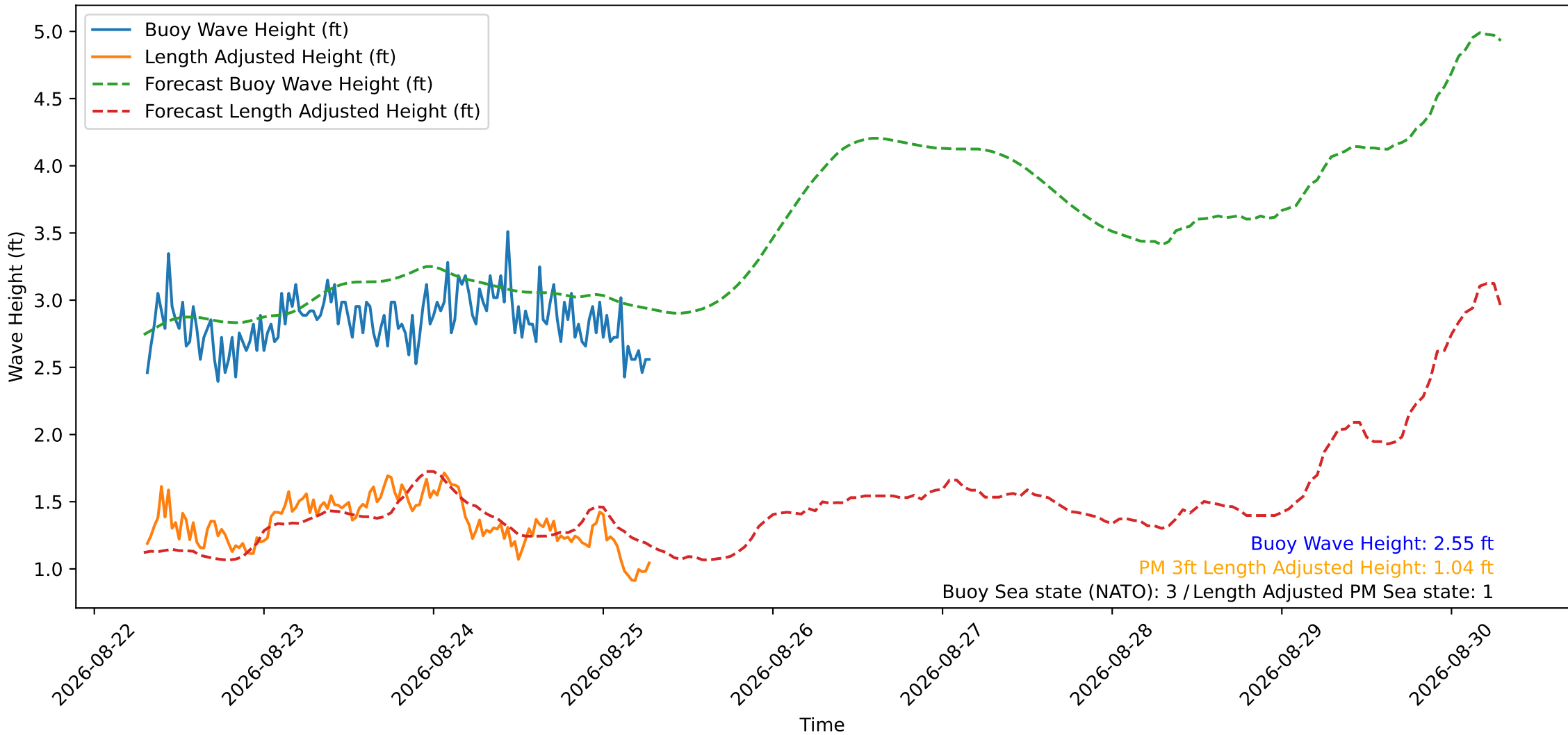
Wave Heights over Time for Oceanside Harbor at 2026-08-25 07:20:29
