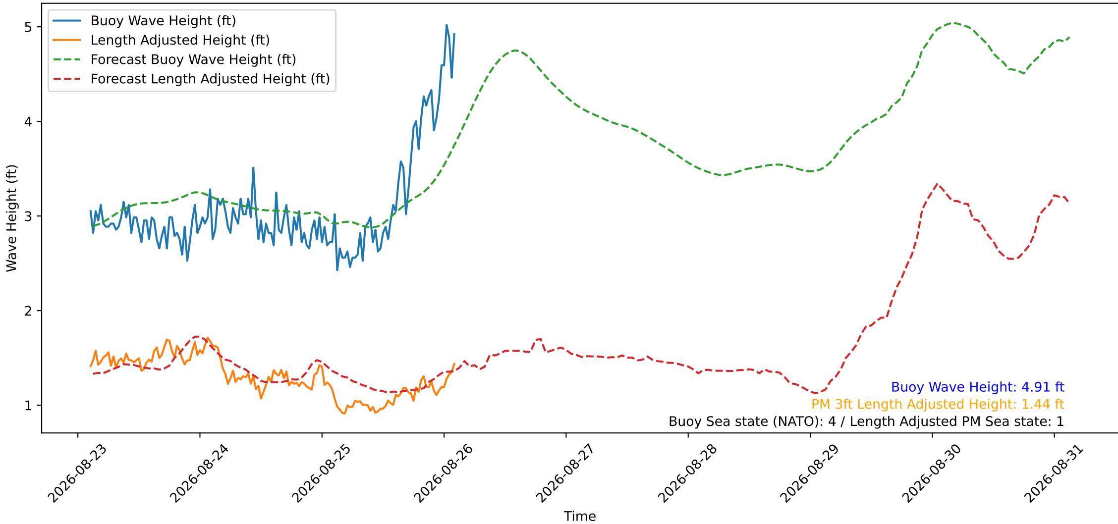
Wave Heights over Time for Oceanside Harbor at 2026-08-26 02:40:29
