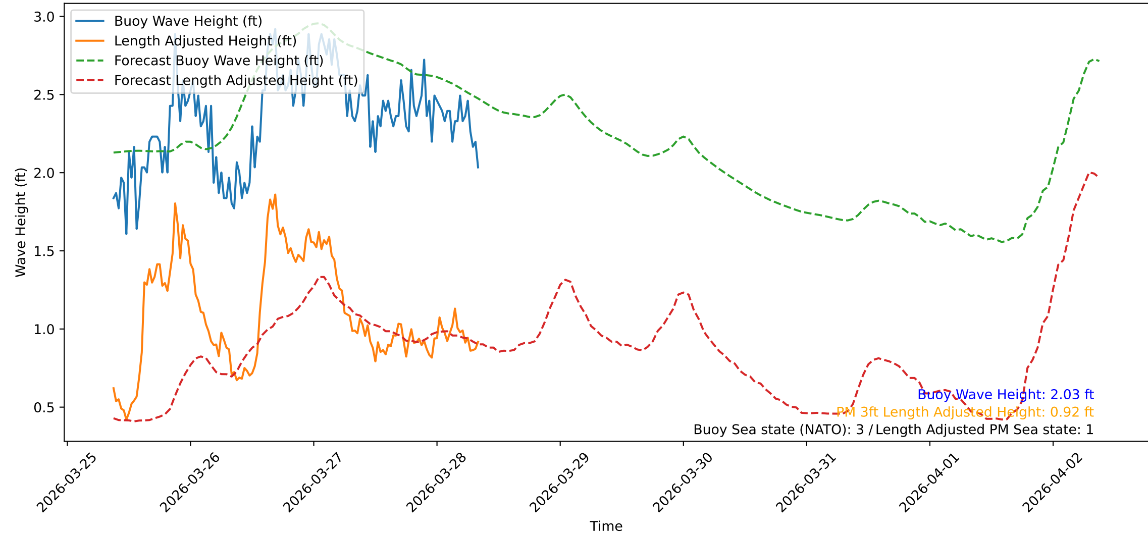
Wave Heights over Time for Oceanside Harbor at 2026-03-28 09:10:32
