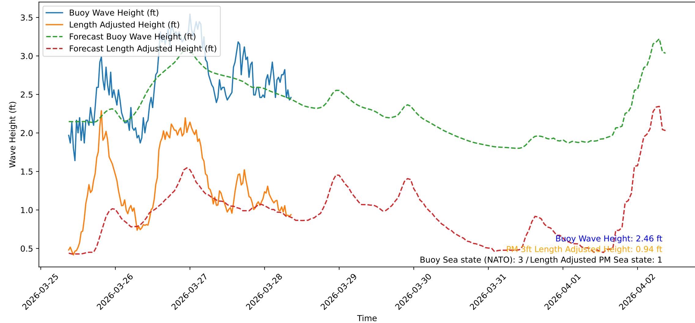
Wave Heights over Time for Green Beach at 2026-03-28 09:11:12
