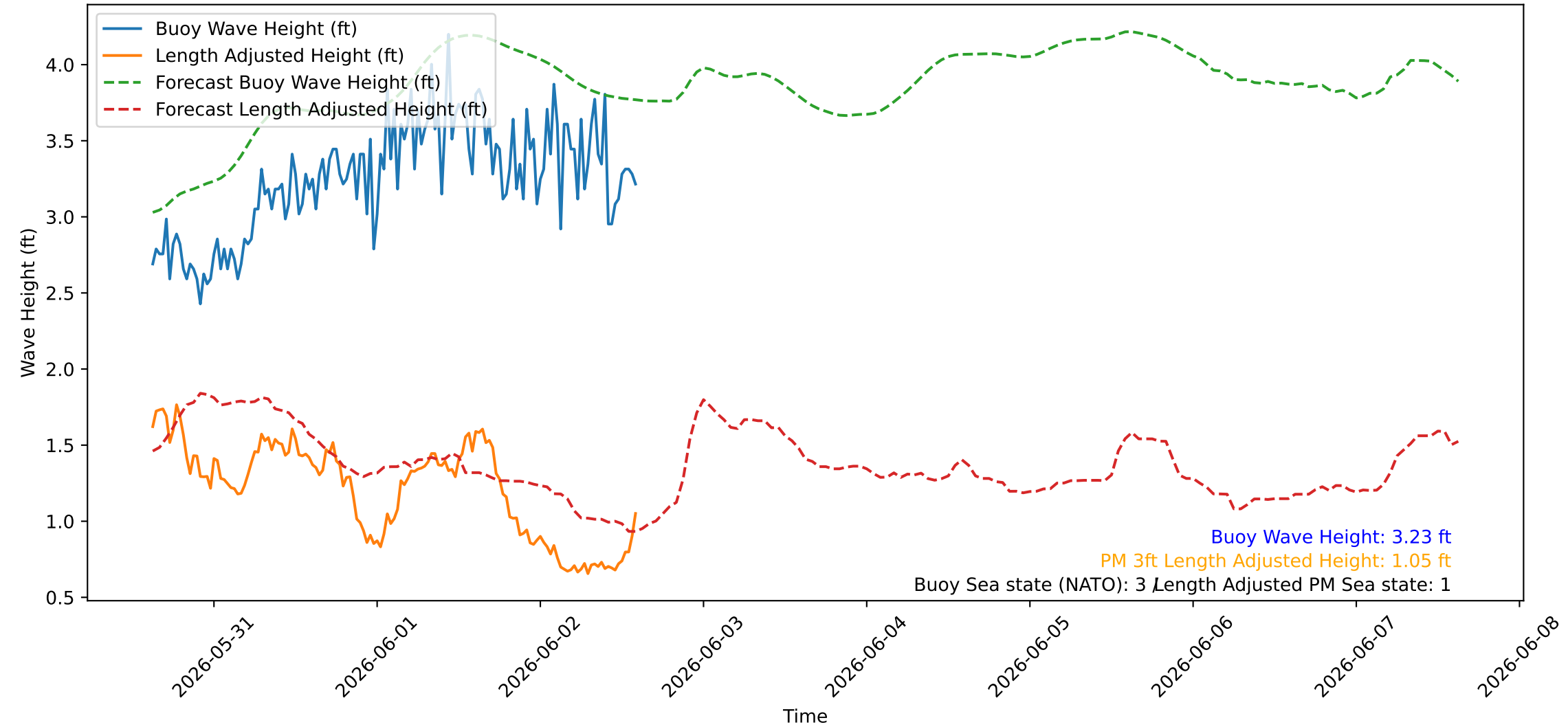
Wave Heights over Time for Red Beach at 2026-06-02 14:50:47
