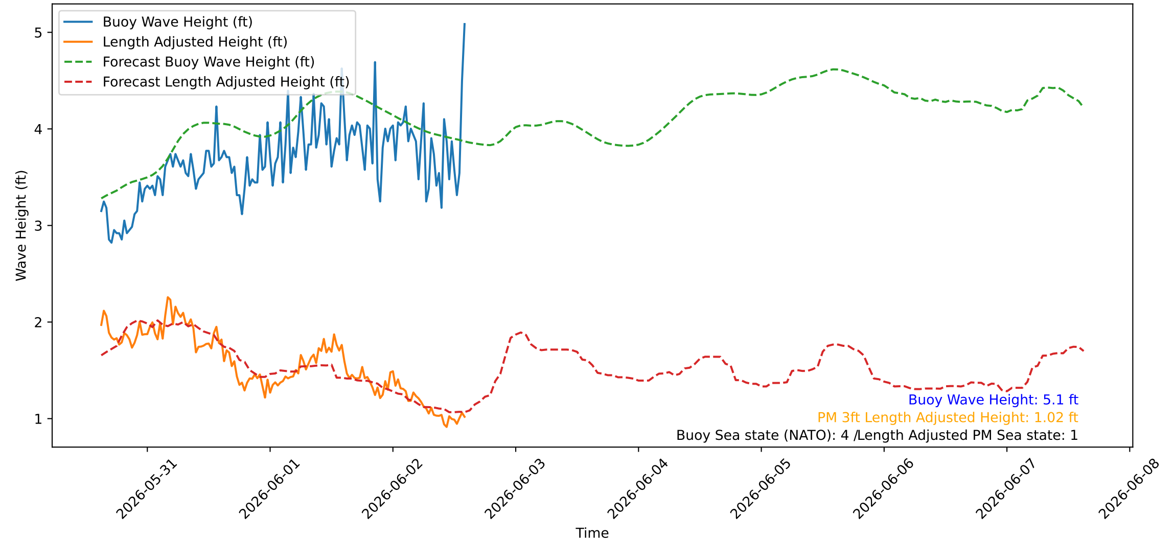
Wave Heights over Time for Oceanside Harbor at 2026-06-02 14:50:26
