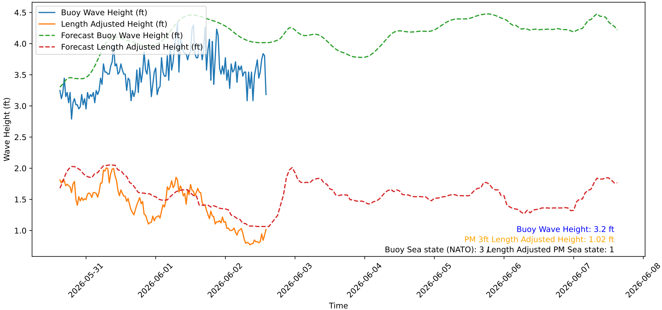
Wave Heights over Time for Green Beach at 2026-06-02 14:51:09
